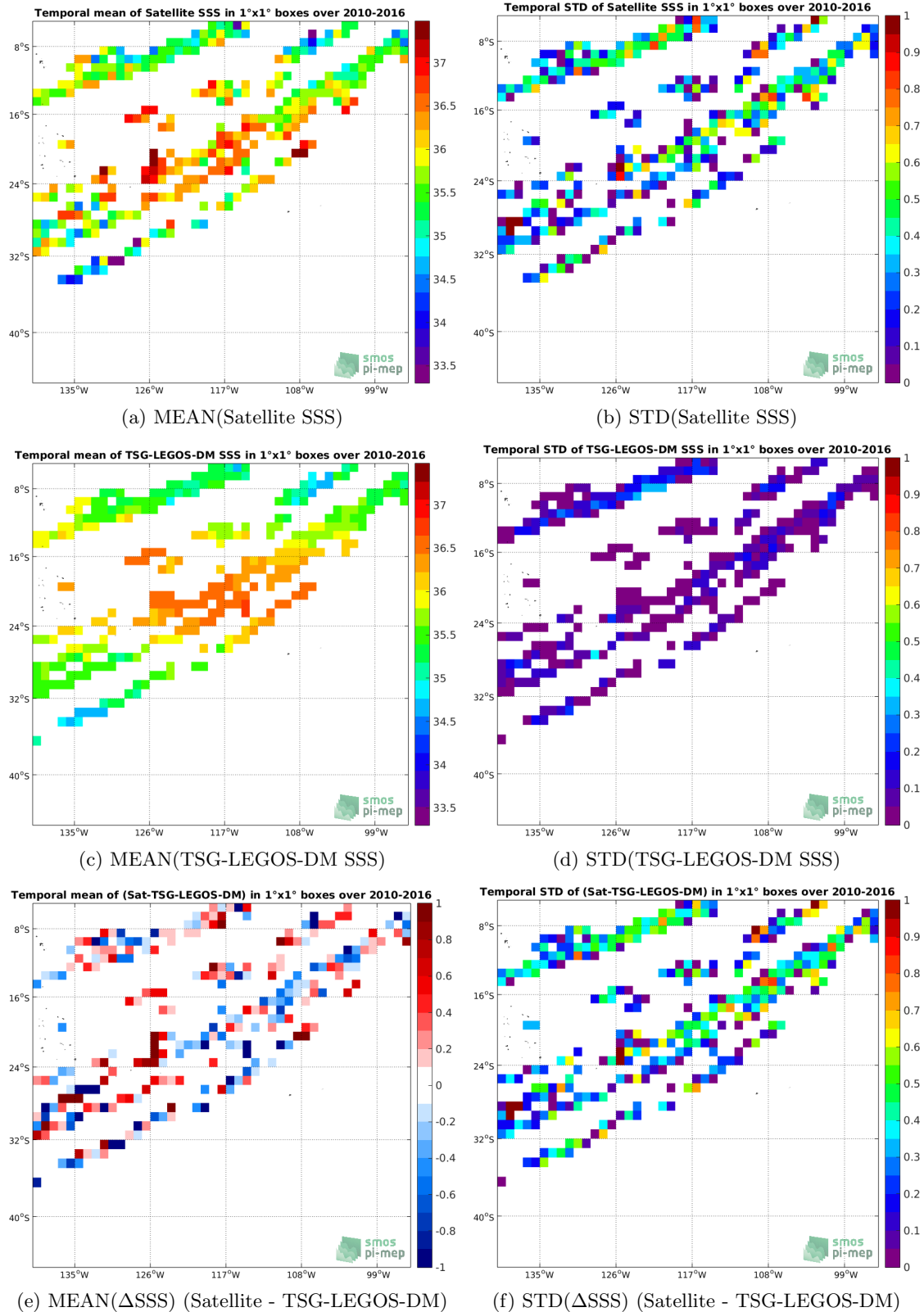
Figure 6: Temporal mean (left) and STD (right) of SSS from SMOS-L2-DPGS-v662 (top), TSG-LEGOS-DM (middle), and of \Delta SSS (Satellite - TSG-LEGOS-DM). Only match-up pairs are used to generate these maps.
