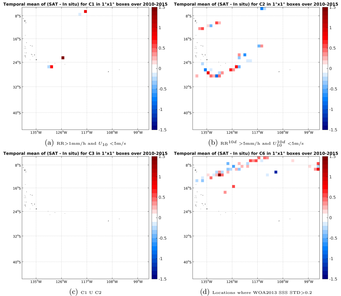
Figure 12: Temporal mean gridded over spatial boxes of size 1°x1° of \Delta SSS (SMOS-L2-DPGS-v662 - TSG-LEGOS-DM) for 4 different subdatasets corresponding to:RR>1mm/h and U_{10} < 5 m/s (a), RR^{10d} > 5 mm/h and U_{10}^{10d} < 5 m/s (b), C1 U C2 (c),Locations where WOA2013 SSS STD>0.2 (d).
