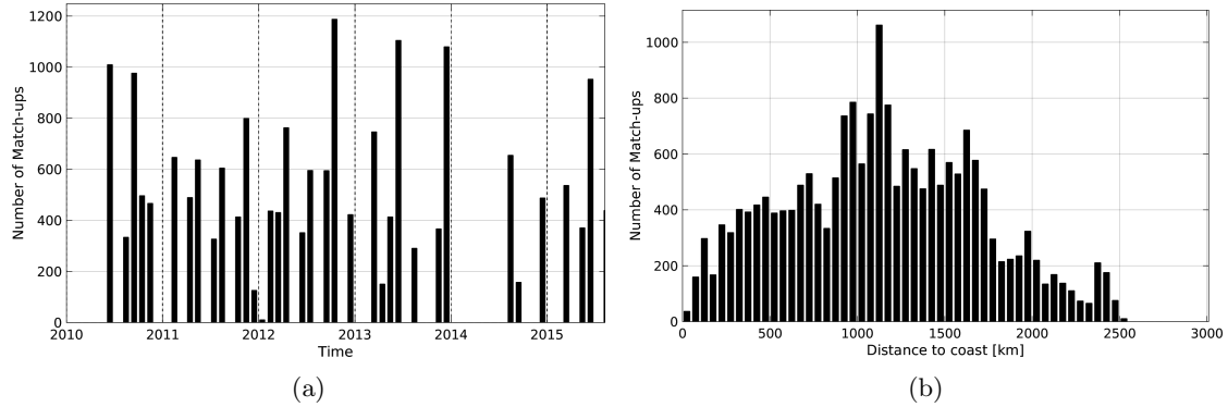
Figure 1: Number of match-ups between TSG-LEGOS-DM and SMOS-L2-DPGS-v662 SSS as a function of time (a) and as function of the distance to coast (b) over the OTT zone Pi-MEP region and for the full satellite product period.
