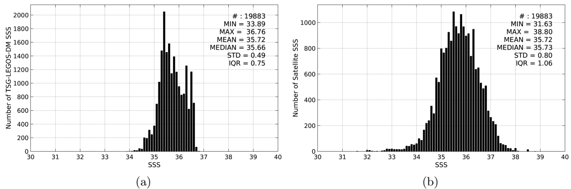
Figure 2: Histograms of SSS from TSG-LEGOS-DM (a) and SMOS-L2-DPGS-v662 (b) considering all match-up pairs per bins of 0.1 over the OTT zone Pi-MEP region and for the full satellite product period.
