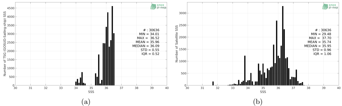
Figure 2: Histograms of SSS from TSG (GOSUD-Sailing-ship) (a) and SMOS SSS L2 v662 (ESA) (b) considering all match-up pairs per bins of 0.1 over the OTT zone Pi-MEP region and for the full satellite product period.
