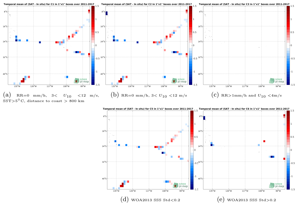
Figure 12: Temporal mean gridded over spatial boxes of size 1^\circ \times 1^\circ of \Delta SSS (SMOS SSS L2 v662 (ESA) - TSG (GOSUD-Sailing-ship)) for 5 different subdatasets corresponding to:RR=0 mm/h, 3 < U_{10} < 12 m/s, SST >5^\circ\text{C} , distance to coast > 800 km (a), RR=0 mm/h, 3 < U_{10} < 12 m/s (b), RR >1 mm/h and U_{10} < 4 m/s (c), WOA2013 SSS Std <0.2 (d), WOA2013 SSS Std >0.2 (e).
