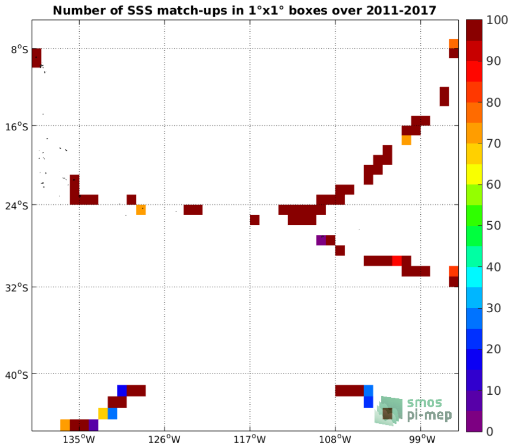
Figure 4: Number of SSS match-ups between TSG (GOSUD-Sailing-ship) SSS and the SMOS SSS L2 v662 (ESA) SSS product for the OTT zone Pi-MEP region over 1^\circ \times 1^\circ boxes and for the full satellite product period.
