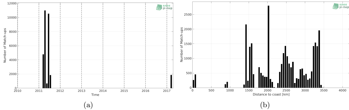
Figure 1: Number of match-ups between TSG (GOSUD-Sailing-ship) and SMOS SSS L2 v662 (ESA) SSS as a function of time (a) and as function of the distance to coast (b) over the OTT zone Pi-MEP region and for the full satellite product period.
