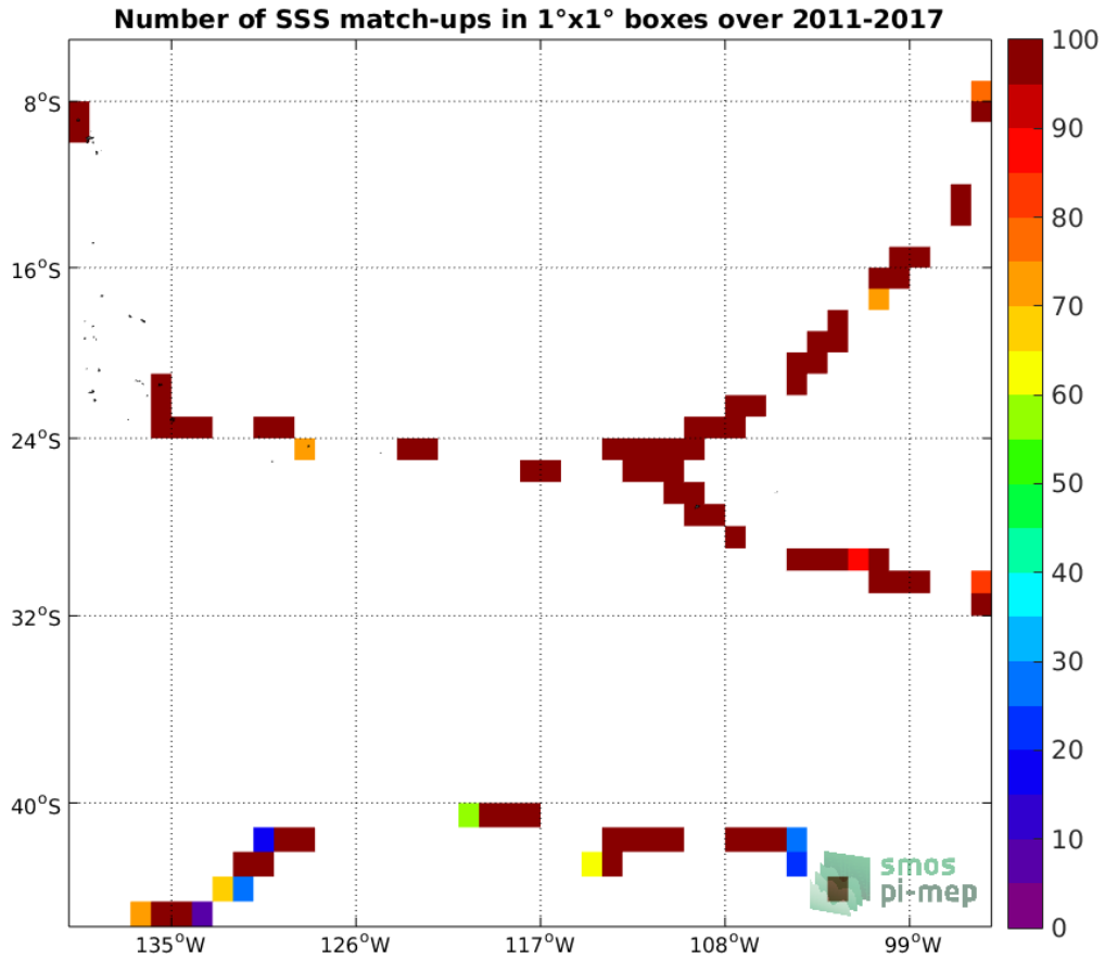
Figure 4: Number of SSS match-ups between TSG (GOSUD-Sailing-ship) SSS and the SMOS SSS L2 v662 (ESA) SSS product for the OTT zone Pi-MEP region over 1°x1° boxes and for the full satellite product period.
