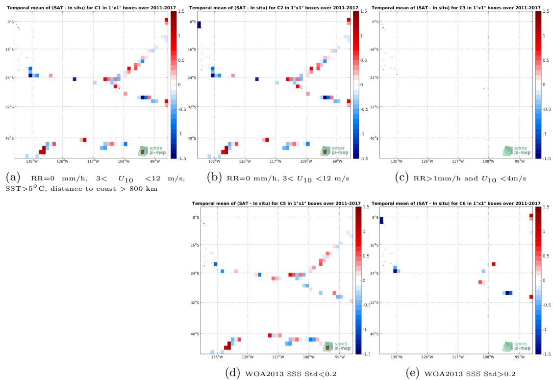
Figure 12: Temporal mean gridded over spatial boxes of size 1^\circ \times 1^\circ of \Delta\text{SSS} (SMOS SSS L2 v662 (ESA) - TSG (GOSUD-Sailing-ship)) for 5 different subdatasets corresponding to: RR=0 mm/h, 3 < U_{10} < 12 m/s, SST > 5°C, distance to coast > 800 km (a), RR=0 mm/h, 3 < U_{10} < 12 m/s (b), RR > 1mm/h and U_{10} < 4 m/s (c), WOA2013 SSS Std < 0.2 (d), WOA2013 SSS Std > 0.2 (e).
