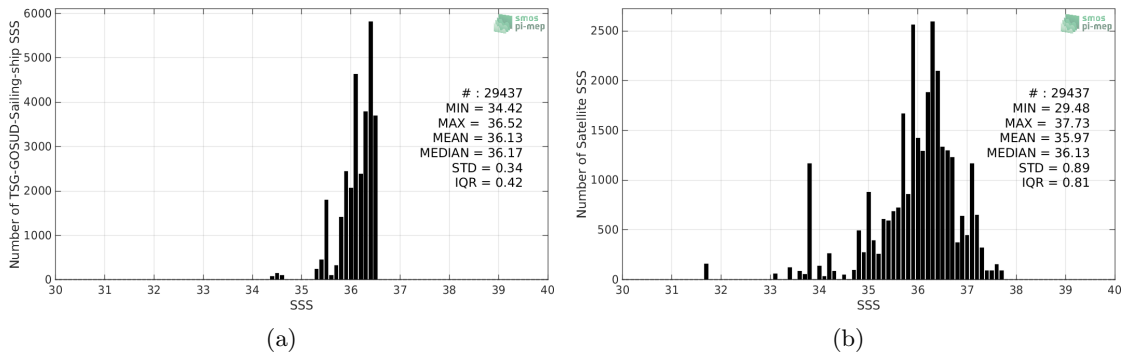
Figure 2: Histograms of SSS from TSG-GOSUD-Sailing-ship (a) and SMOS-L2-DPGS-v662 (b) considering all match-up pairs per bins of 0.1 over the OTT zone Pi-MEP region and for the full satellite product period.
