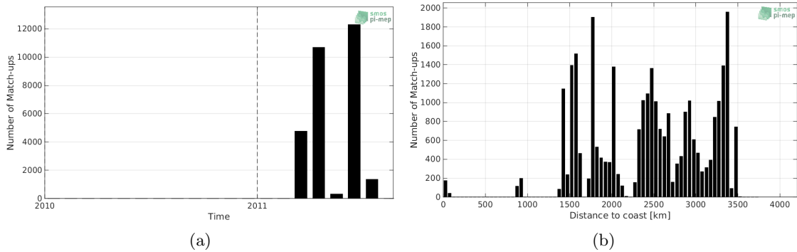
Figure 1: Number of match-ups between TSG-GOSUD-Sailing-ship and SMOS-L2-DPGS-v662 SSS as a function of time (a) and as function of the distance to coast (b) over the OTT zone Pi-MEP region and for the full satellite product period.
