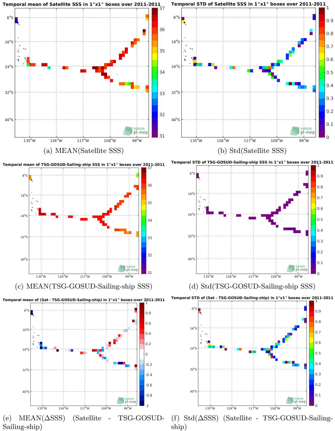
Figure 6: Temporal mean (left) and Std (right) of SSS from SMOS-L2-DPGS-v662 (top), TSG-GOSUD-Sailing-ship (middle), and of \Delta SSS (Satellite - TSG-GOSUD-Sailing-ship). Only match-up pairs are used to generate these maps.
