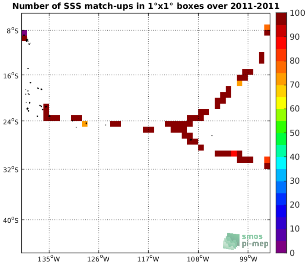
Figure 4: Number of SSS match-ups between TSG-GOSUD-Sailing-ship SSS and the SMOS-L2-DPGS-v662 SSS product for the OTT zone Pi-MEP region over 1°x1° boxes and for the full satellite product period.
