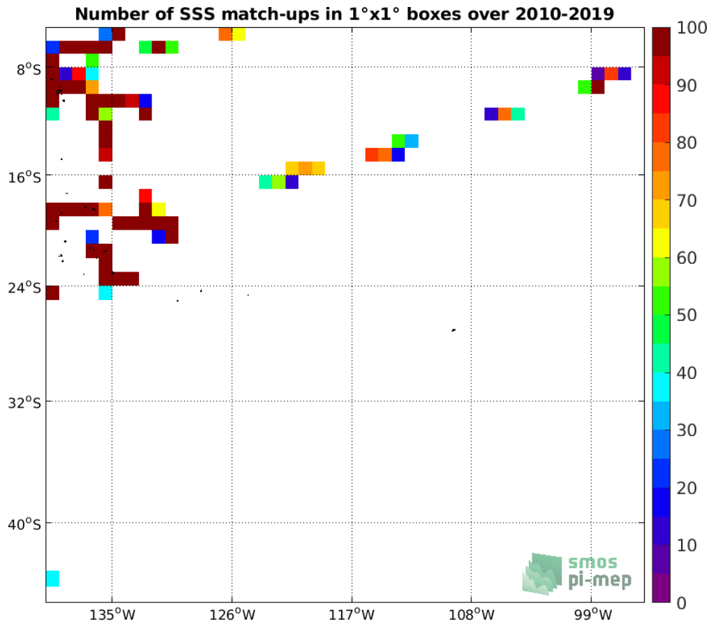
Figure 4: Number of SSS match-ups between TSG (GOSUD-Research-vessel) SSS and the SMOS SSS L2 v662 (ESA) SSS product for the OTT zone Pi-MEP region over 1^\circ \times 1^\circ boxes and for the full satellite product period.
