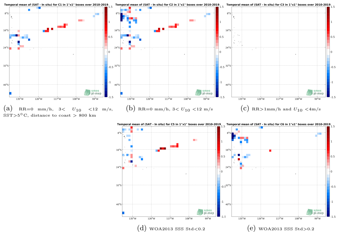
Figure 12: Temporal mean gridded over spatial boxes of size 1^\circ \times 1^\circ of \Delta SSS (SMOS SSS L2 v662 (ESA) - TSG (GOSUD-Research-vessel)) for 5 different subdatasets corresponding to:RR=0 mm/h, 3 < U_{10} < 12 m/s, SST > 5^\circ\text{C} , distance to coast > 800 km (a), RR=0 mm/h, 3 < U_{10} < 12 m/s (b), RR > 1 mm/h and U_{10} < 4 m/s (c), WOA2013 SSS Std < 0.2 (d), WOA2013 SSS Std > 0.2 (e).
