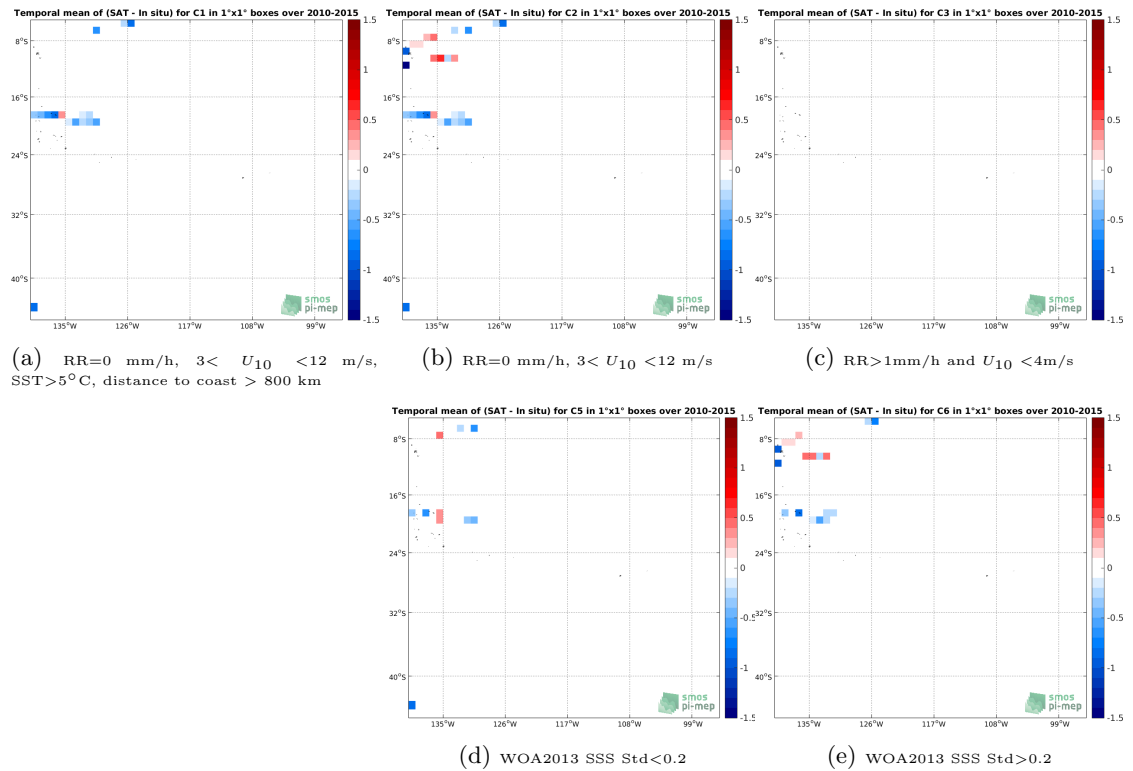
Figure 12: Temporal mean gridded over spatial boxes of size 1^\circ \times 1^\circ of \Delta SSS (SMOS-L2-DPGS-v662 - TSG-GOSUD-Research-vessel) for 5 different subdatasets corresponding to: RR=0 mm/h, 3 < U_{10} < 12 m/s, SST > 5^\circ C , distance to coast > 800 km (a), RR=0 mm/h, 3 < U_{10} < 12 m/s (b), RR > 1 mm/h and U_{10} < 4 m/s (c), WOA2013 SSS Std < 0.2 (d), WOA2013 SSS Std > 0.2 (e).
