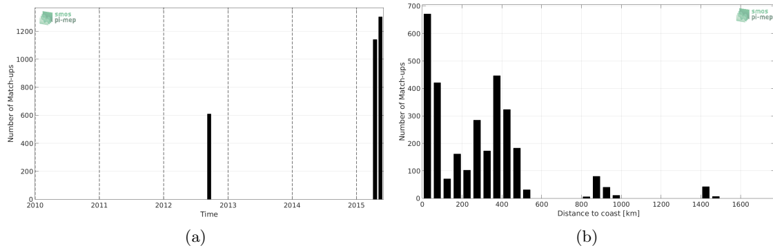
Figure 1: Number of match-ups between TSG-GOSUD-Research-vessel and SMOS-L2-DPGS-v662 SSS as a function of time (a) and as function of the distance to coast (b) over the OTT zone Pi-MEP region and for the full satellite product period.
