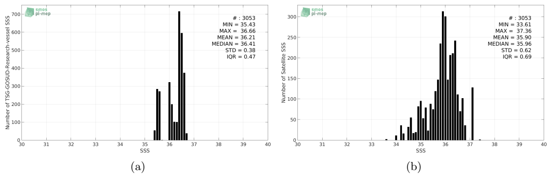
Figure 2: Histograms of SSS from TSG-GOSUD-Research-vessel (a) and SMOS-L2-DPGS-v662 (b) considering all match-up pairs per bins of 0.1 over the OTT zone Pi-MEP region and for the full satellite product period.
