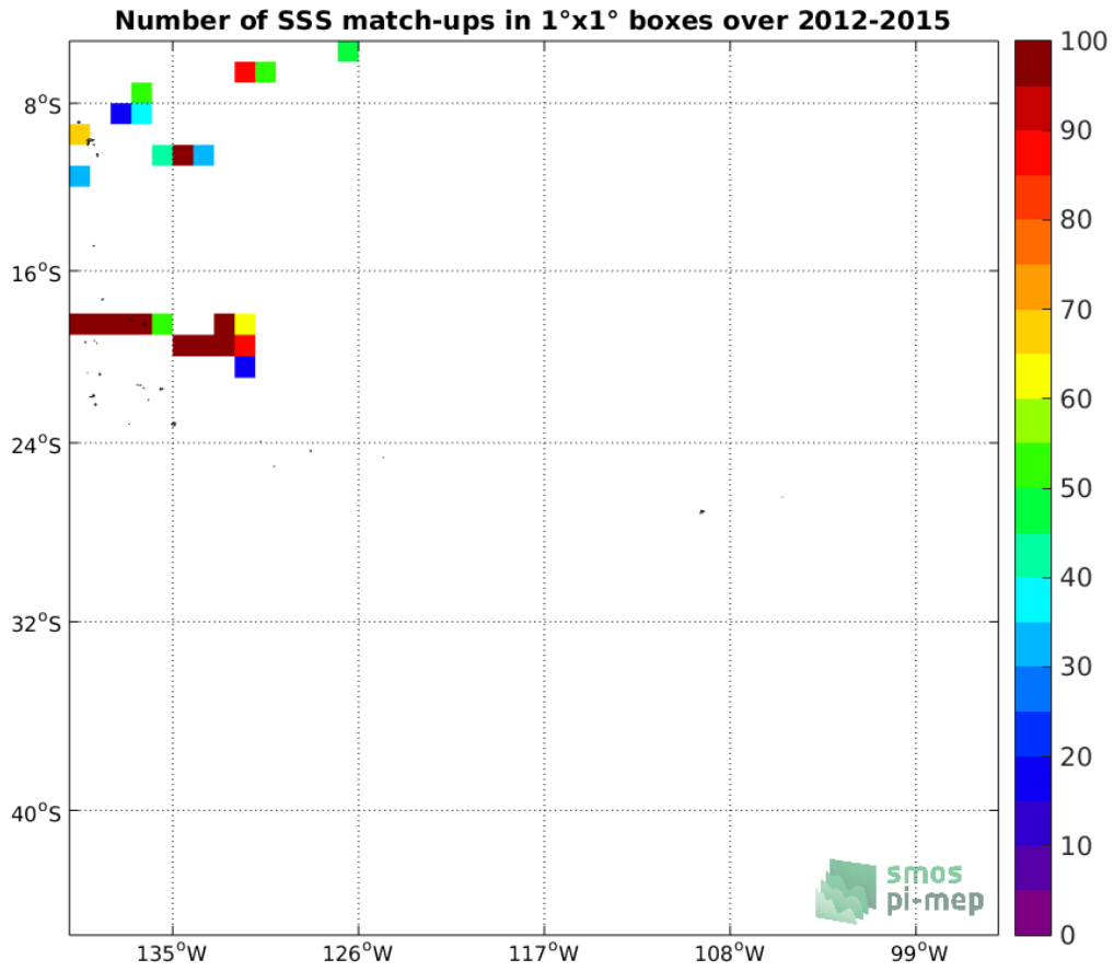
Figure 4: Number of SSS match-ups between TSG-GOSUD-Research-vessel SSS and the SMOS-L2-DPGS-v662 SSS product for the OTT zone Pi-MEP region over 1°x1° boxes and for the full satellite product period.
