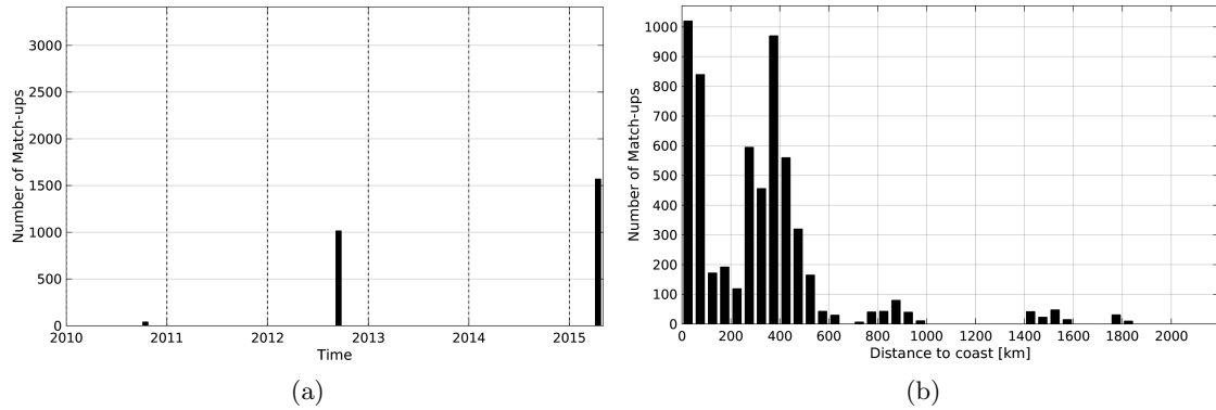
Figure 1: Number of match-ups between TSG-GOSUD-Research-vessel and SMOS-L2-DPGS-v662 SSS as a function of time (a) and as function of the distance to coast (b) over the OTT zone Pi-MEP region and for the full satellite product period.
