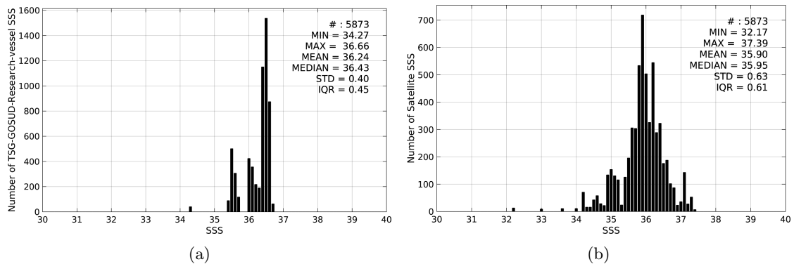
Figure 2: Histograms of SSS from TSG-GOSUD-Research-vessel (a) and SMOS-L2-DPGS-v662 (b) considering all match-up pairs per bins of 0.1 over the OTT zone Pi-MEP region and for the full satellite product period.
