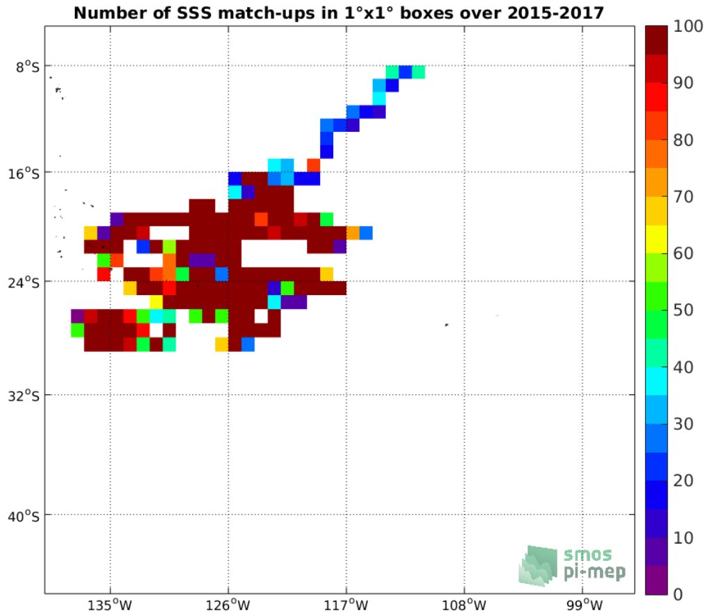
Figure 3: Number of SSS match-ups between Surface drifters SSS and the SMOS SSS L2 v662 (ESA) SSS product for the OTT zone Pi-MEP region over 1^\circ \times 1^\circ boxes and for the full satellite product period.
