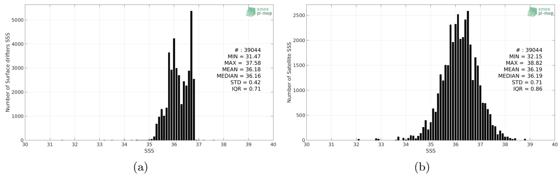
Figure 2: Histograms of SSS from Surface drifters (a) and SMOS SSS L2 v662 (ESA) (b) considering all match-up pairs per bins of 0.1 over the OTT zone Pi-MEP region and for the full satellite product period.
