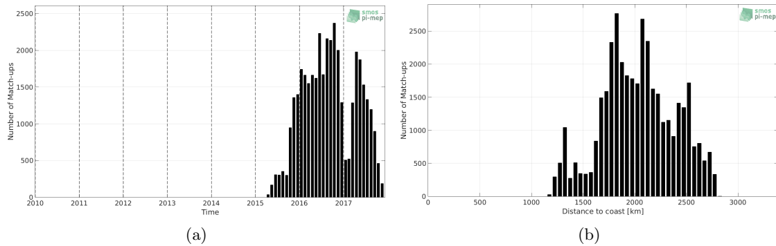
Figure 1: Number of match-ups between Surface drifters and SMOS SSS L2 v662 (ESA) SSS as a function of time (a) and as function of the distance to coast (b) over the OTT zone Pi-MEP region and for the full satellite product period.
