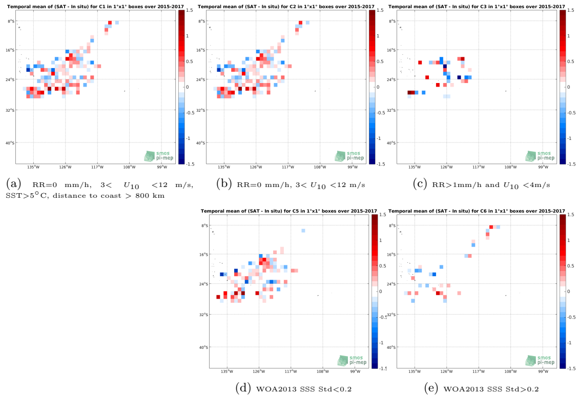
Figure 11: Temporal mean gridded over spatial boxes of size 1^\circ \times 1^\circ of \Delta SSS (SMOS SSS L2 v662 (ESA) - Surface drifters) for 5 different subdatasets corresponding to:RR=0 mm/h, 3 < U_{10} < 12 m/s, SST > 5^\circ\text{C} , distance to coast > 800 km (a), RR=0 mm/h, 3 < U_{10} < 12 m/s (b), RR > 1 mm/h and U_{10} < 4 m/s (c), WOA2013 SSS Std < 0.2 (d), WOA2013 SSS Std > 0.2 (e).
