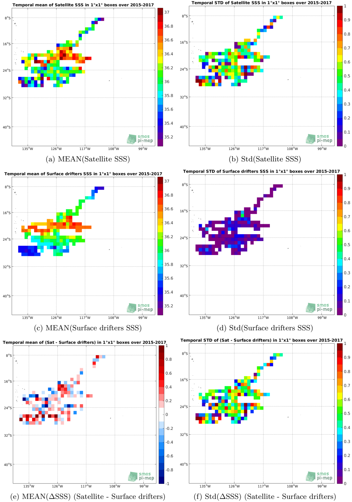
Figure 5: Temporal mean (left) and Std (right) of SSS from SMOS SSS L2 v662 (ESA) (top), Surface drifters (middle), and of \Delta SSS (Satellite - Surface drifters). Only match-up pairs are used to generate these maps.
