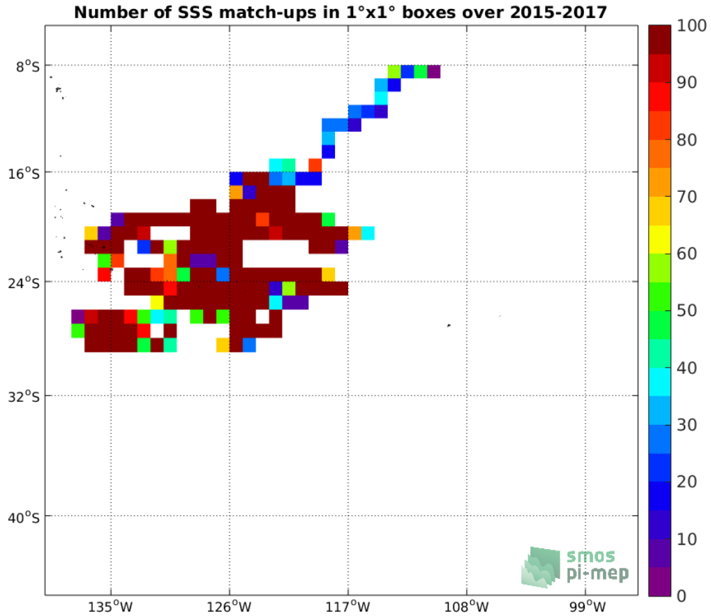
Figure 3: Number of SSS match-ups between Surface drifters SSS and the SMOS SSS L2 v662 (ESA) SSS product for the OTT zone Pi-MEP region over 1°x1° boxes and for the full satellite product period.
