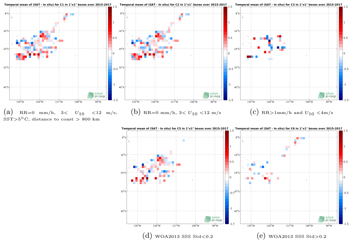
Figure 11: Temporal mean gridded over spatial boxes of size 1^\circ \times 1^\circ of \Delta\text{SSS} (SMOS SSS L2 v662 (ESA) - Surface drifters) for 5 different subdatasets corresponding to:RR=0 mm/h, 3 < U_{10} < 12 m/s, SST >5^\circ\text{C} , distance to coast > 800 km (a), RR=0 mm/h, 3 < U_{10} < 12 m/s (b), RR >1 mm/h and U_{10} < 4 m/s (c), WOA2013 SSS Std <0.2 (d), WOA2013 SSS Std >0.2 (e).
