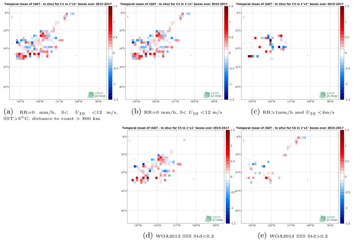
Figure 11: Temporal mean gridded over spatial boxes of size 1^\circ \times 1^\circ of \Delta SSS (SMOS L2 v662 (ESA) - Surface drifters) for 5 different subdatasets corresponding to:RR=0 mm/h, 3 < U_{10} < 12 m/s, SST >5^\circ\text{C} , distance to coast > 800 km (a), RR=0 mm/h, 3 < U_{10} < 12 m/s (b), RR >1 mm/h and U_{10} < 4 m/s (c), WOA2013 SSS Std <0.2 (d), WOA2013 SSS Std >0.2 (e).
