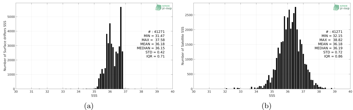
Figure 2: Histograms of SSS from Surface drifters (a) and SMOS L2 v662 (ESA) (b) considering all match-up pairs per bins of 0.1 over the OTT zone Pi-MEP region and for the full satellite product period.
