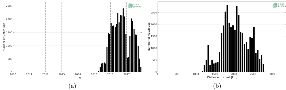
Figure 1: Number of match-ups between Surface drifters and SMOS L2 v662 (ESA) SSS as a function of time (a) and as function of the distance to coast (b) over the OTT zone Pi-MEP region and for the full satellite product period.
