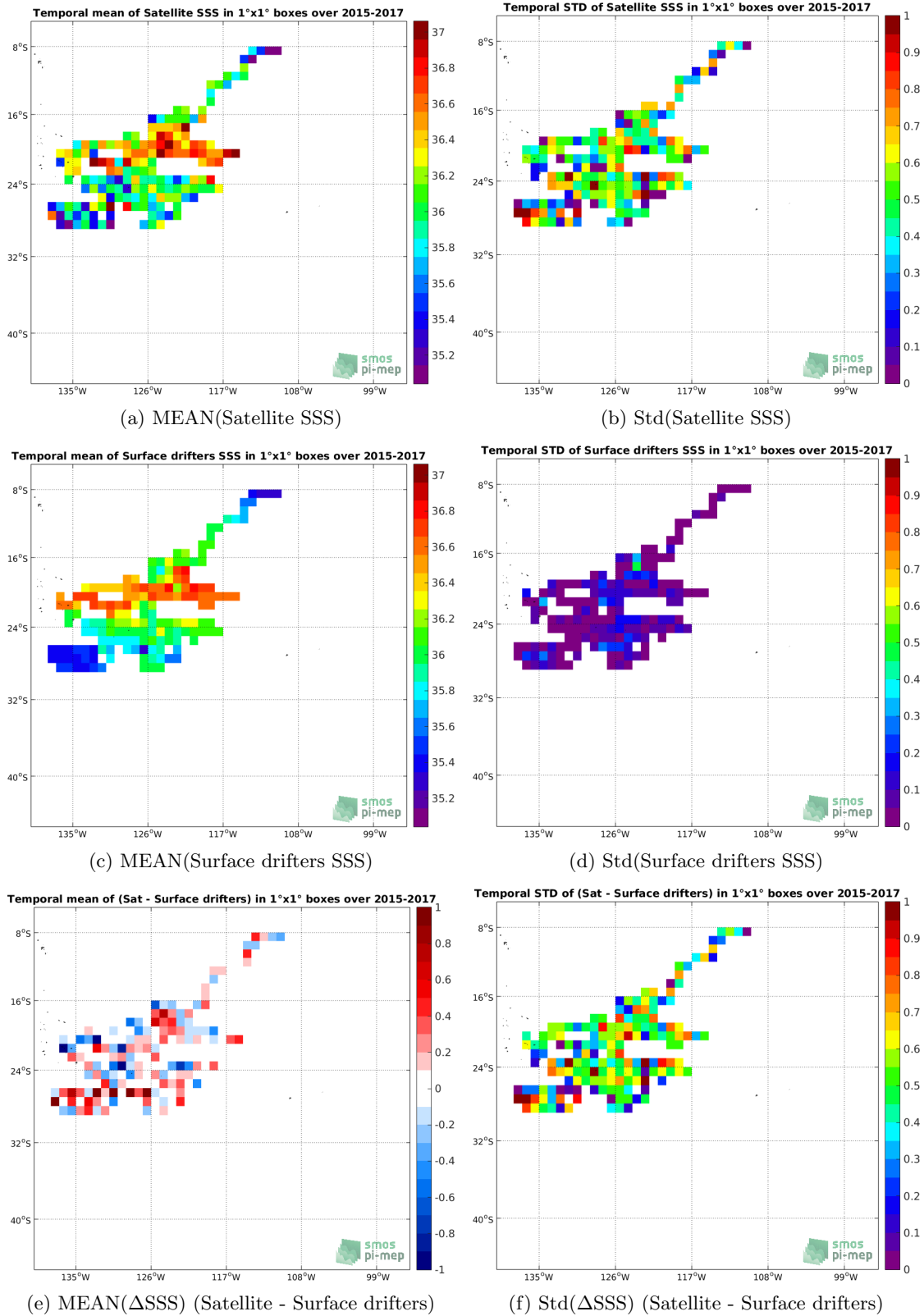
Figure 5: Temporal mean (left) and Std (right) of SSS from SMOS L2 v662 (ESA) (top), Surface drifters (middle), and of \Delta SSS (Satellite - Surface drifters). Only match-up pairs are used to generate these maps.
