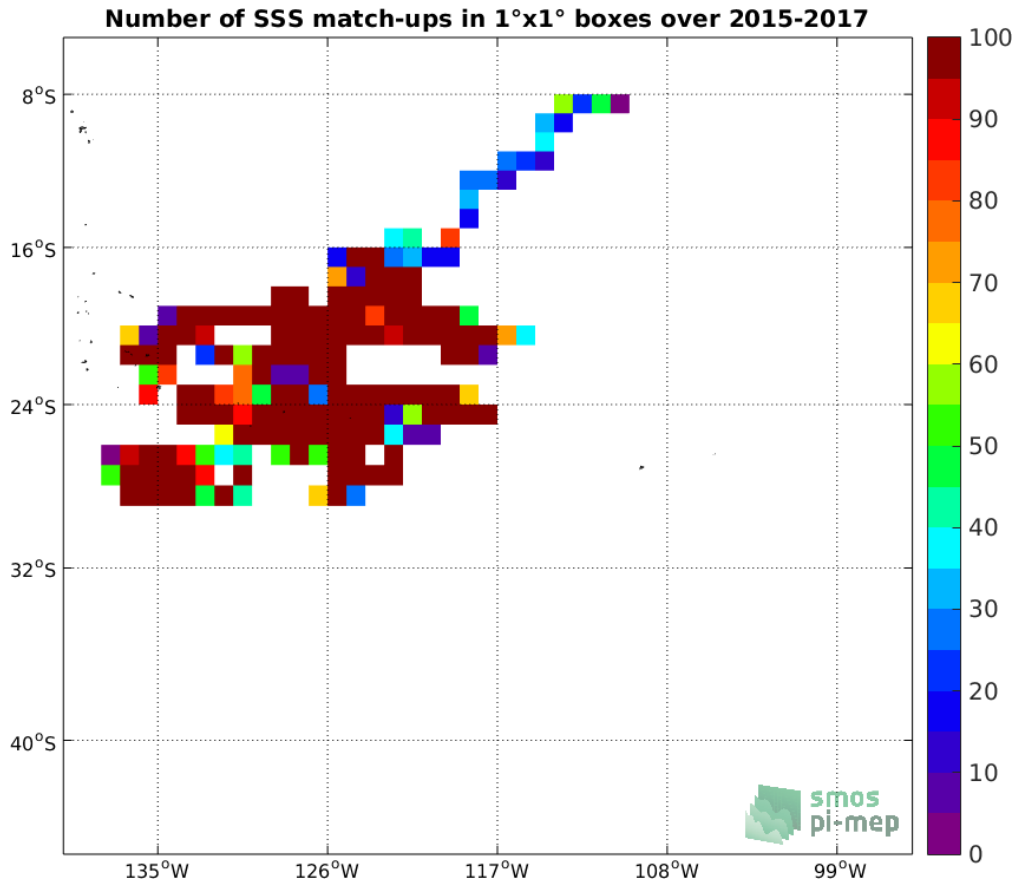
Figure 3: Number of SSS match-ups between Surface drifters SSS and the SMOS L2 v662 (ESA) SSS product for the OTT zone Pi-MEP region over 1°x1° boxes and for the full satellite product period.
