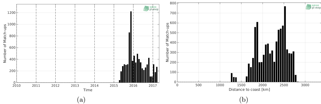
Figure 1: Number of match-ups between Surface drifters and SMOS-L2-DPGS-v662 SSS as a function of time (a) and as function of the distance to coast (b) over the OTT zone Pi-MEP region and for the full satellite product period.
