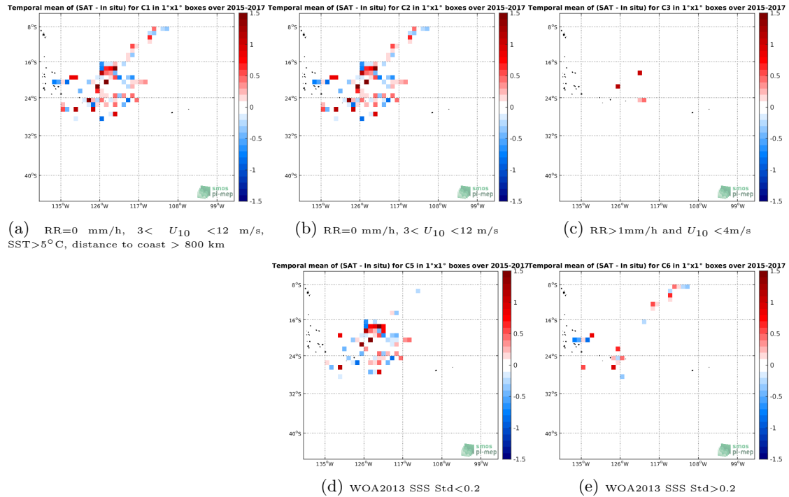
Figure 11: Temporal mean gridded over spatial boxes of size 1^\circ \times 1^\circ of \Delta SSS (SMOS-L2-DPGS-v662 - Surface drifters) for 5 different subdatasets corresponding to:RR=0 mm/h, 3 < U_{10} < 12 m/s, SST >5^\circ C, distance to coast > 800 km (a), RR=0 mm/h, 3 < U_{10} < 12 m/s (b), RR >1 mm/h and U_{10} < 4 m/s (c), WOA2013 SSS Std <0.2 (d), WOA2013 SSS Std >0.2 (e).
