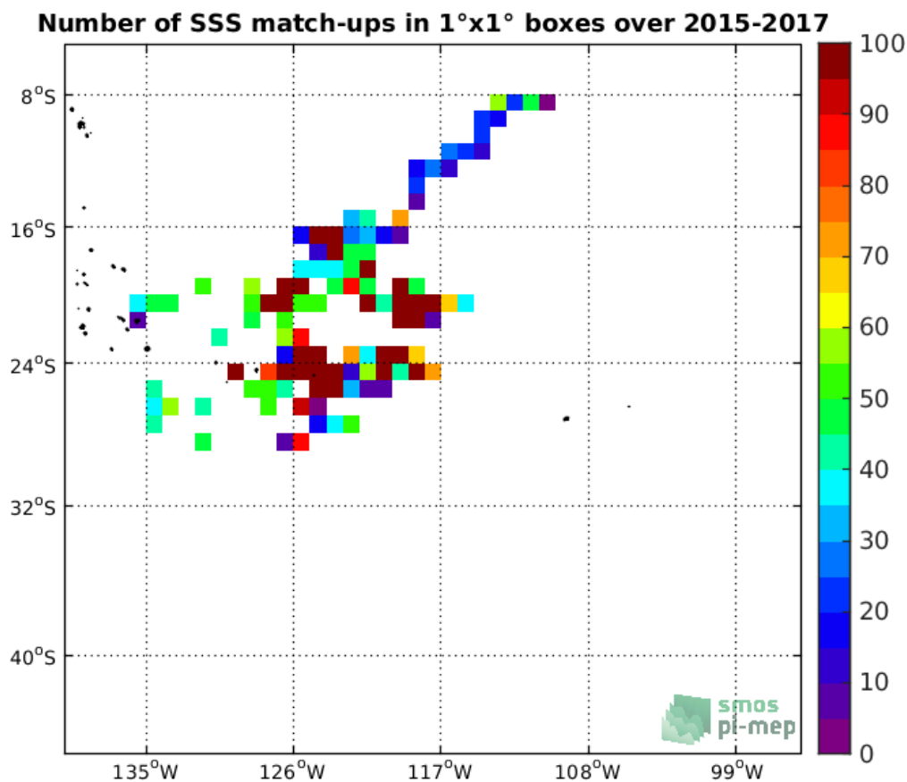
Figure 3: Number of SSS match-ups between Surface drifters SSS and the SMOS-L2-DPGS-v662 SSS product for the OTT zone Pi-MEP region over 1°x1° boxes and for the full satellite product period.
