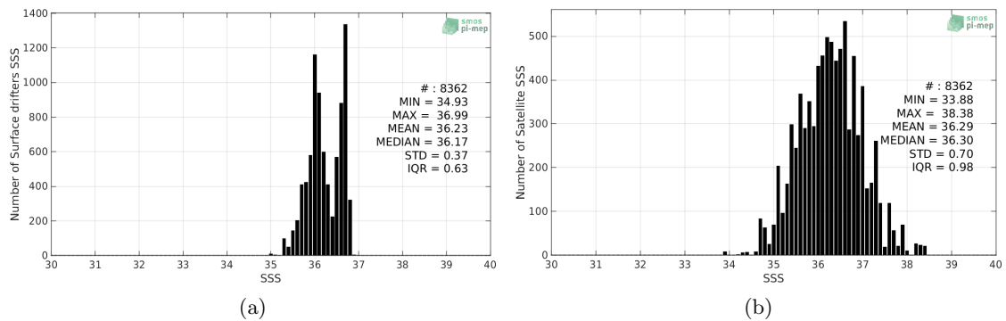
Figure 2: Histograms of SSS from Surface drifters (a) and SMOS-L2-DPGS-v662 (b) considering all match-up pairs per bins of 0.1 over the OTT zone Pi-MEP region and for the full satellite product period.
