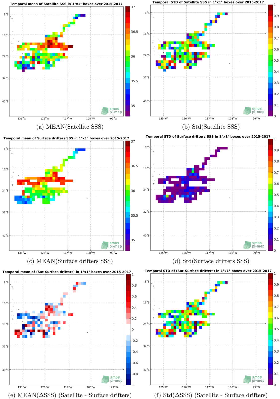
(a) MEAN(Satellite SSS) (b) Std(Satellite SSS) (c) MEAN(Surface drifters SSS) (d) Std(Surface drifters SSS) (e) MEAN( \Delta SSS) (Satellite - Surface drifters) (f) Std( \Delta SSS) (Satellite - Surface drifters) Figure 5: Temporal mean (left) and Std (right) of SSS from SMOS-L2-DPGS-v662 (top), Surface drifters (middle), and of \Delta SSS (Satellite - Surface drifters). Only match-up pairs are used to generate these maps.
