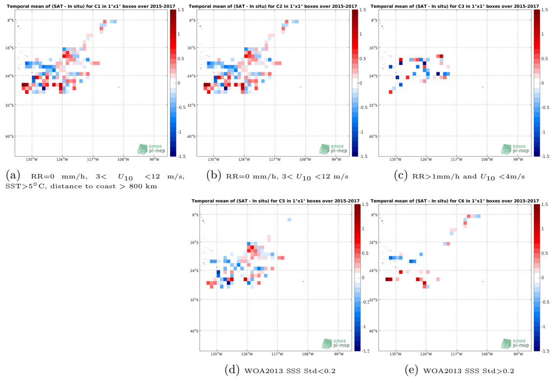
Figure 11: Temporal mean gridded over spatial boxes of size 1^\circ \times 1^\circ of \Delta SSS (SMOS-L2-DPGS-v662 - Surface drifters) for 5 different subdatasets corresponding to:RR=0 mm/h, 3 < U_{10} < 12 m/s, SST >5^\circ C, distance to coast > 800 km (a), RR=0 mm/h, 3 < U_{10} < 12 m/s (b), RR >1 mm/h and U_{10} < 4 m/s (c), WOA2013 SSS Std <0.2 (d), WOA2013 SSS Std >0.2 (e).
