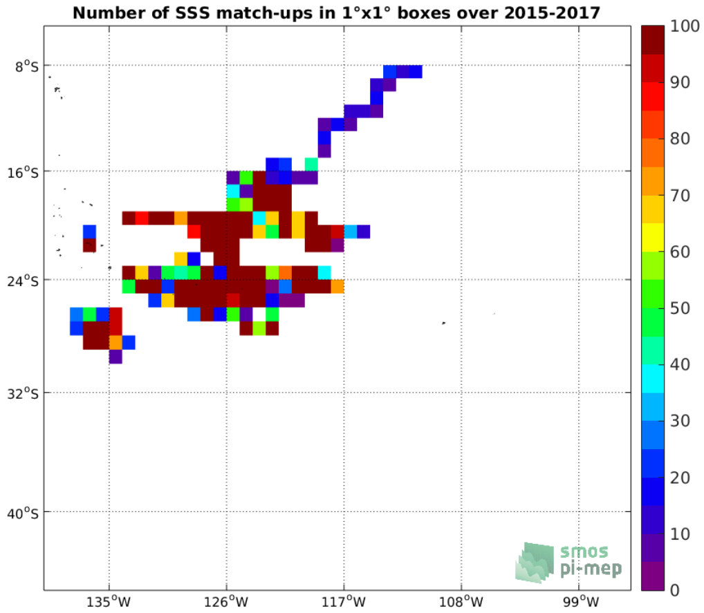
Figure 3: Number of SSS match-ups between Surface drifters SSS and the SMOS-2 L2-TPGS-v662 SSS product for the OTT zone Pi-MEP region over 1°x1° boxes and for the full satellite product period.
