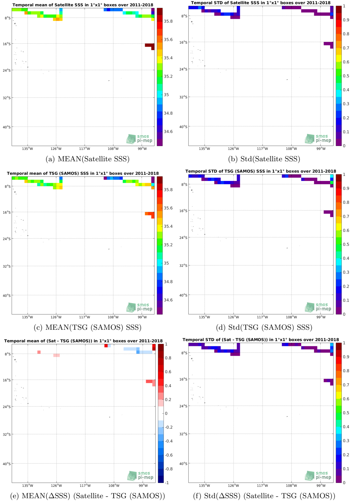
Figure 6: Temporal mean (left) and Std (right) of SSS from SMAP SSS L4 OI v1 - 7 Days (IPRC) (top), TSG (SAMOS) (middle), and of \Delta SSS (Satellite - TSG (SAMOS)). Only match-up pairs are used to generate these maps.
