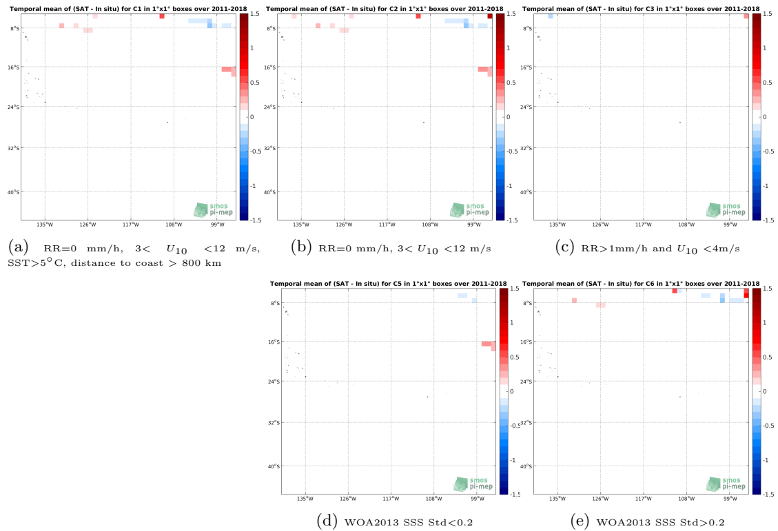
Figure 12: Temporal mean gridded over spatial boxes of size 1^\circ \times 1^\circ of \Delta SSS (SMAP SSS L4 OI v1 - 7 Days (IPRC) - TSG (SAMOS)) for 5 different subdatasets corresponding to: RR=0 mm/h, 3 < U_{10} < 12 m/s, SST > 5^\circ C , distance to coast > 800 km (a), RR=0 mm/h, 3 < U_{10} < 12 m/s (b), RR > 1 mm/h and U_{10} < 4 m/s (c), WOA2013 SSS Std < 0.2 (d), WOA2013 SSS Std > 0.2 (e).
