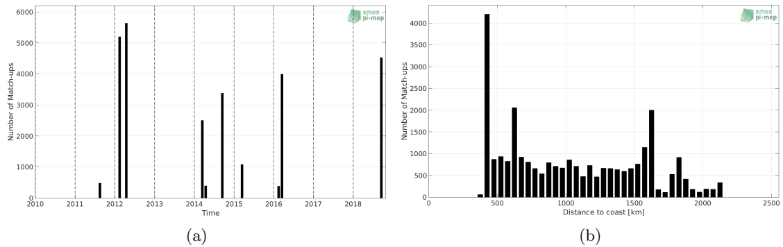
Figure 1: Number of match-ups between TSG (SAMOS) and SMAP SSS L4 OI v1 - 7 Days (IPRC) SSS as a function of time (a) and as function of the distance to coast (b) over the OTT zone Pi-MEP region and for the full satellite product period.
