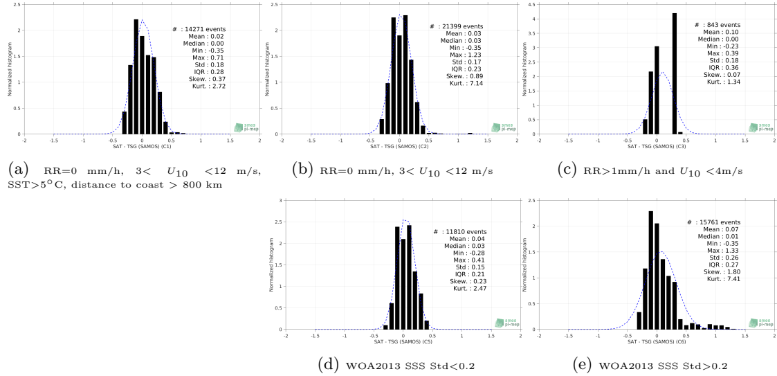
Figure 13: Normalized histogram of \Delta\text{SSS} (SMAP SSS L4 OI v1 - 7 Days (IPRC) - TSG (SAMOS)) for 5 different subdatasets corresponding to: RR=0 mm/h, 3 < U_{10} < 12 m/s, SST>5°C, distance to coast > 800 km (a), RR=0 mm/h, 3 < U_{10} < 12 m/s (b), RR>1mm/h and U_{10} < 4 m/s (c), WOA2013 SSS Std<0.2 (d), WOA2013 SSS Std>0.2 (e).
