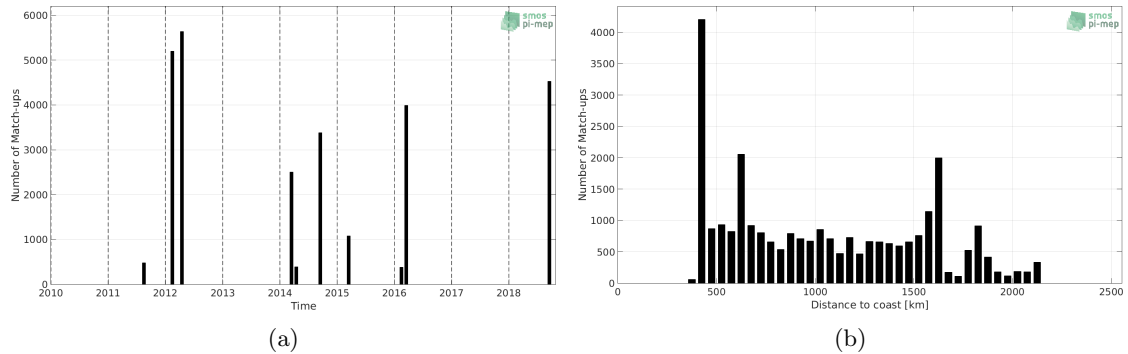
Figure 1: Number of match-ups between TSG (SAMOS) and SMAP SSS L4 OI v1 - 7day (IPRC) SSS as a function of time (a) and as function of the distance to coast (b) over the OTT zone Pi-MEP region and for the full satellite product period.
