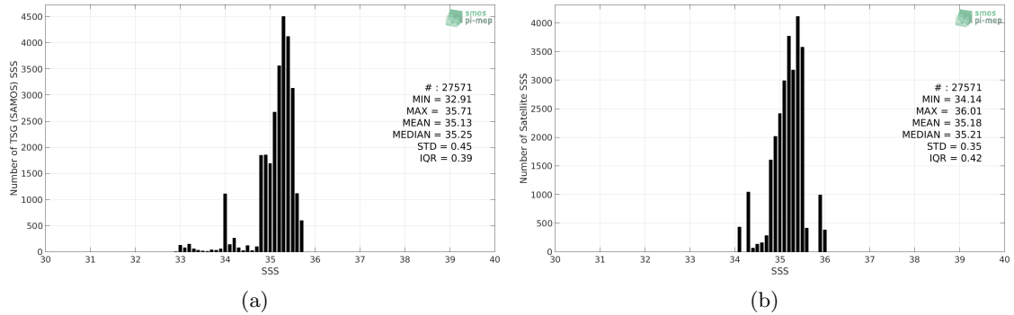
Figure 2: Histograms of SSS from TSG (SAMOS) (a) and SMAP SSS L4 OI v1 - 7day (IPRC) (b) considering all match-up pairs per bins of 0.1 over the OTT zone Pi-MEP region and for the full satellite product period.
