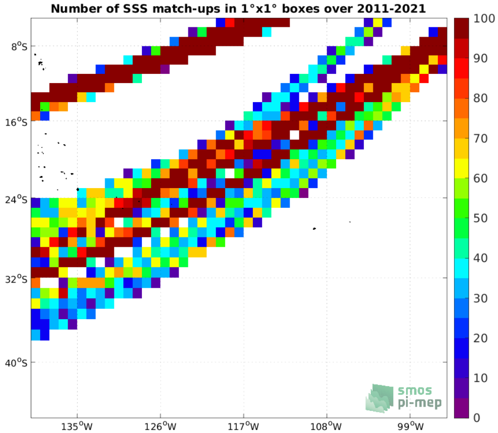
Figure 4: Number of SSS match-ups between TSG (LEGOS-DM) SSS and the SMAP SSS L4 OI v1 - 7 Days (IPRC) SSS product for the OTT zone Pi-MEP region over 1^\circ \times 1^\circ boxes and for the full satellite product period.
