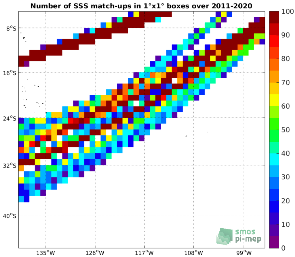
Figure 4: Number of SSS match-ups between TSG (LEGOS-DM) SSS and the SMAP SSS L4 OI v1 - 7 Days (IPRC) SSS product for the OTT zone Pi-MEP region over 1^{\circ} \times 1^{\circ} boxes and for the full satellite product period.
