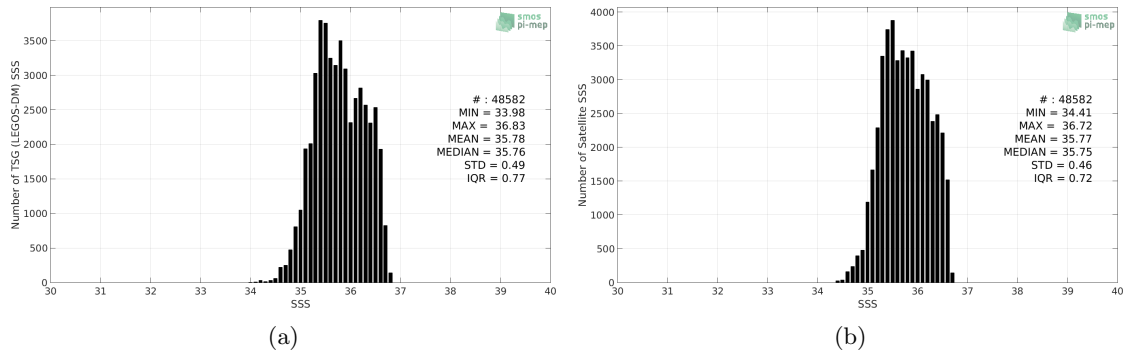
Figure 2: Histograms of SSS from TSG (LEGOS-DM) (a) and SMAP SSS L4 OI v1 - 7 Days (IPRC) (b) considering all match-up pairs per bins of 0.1 over the OTT zone Pi-MEP region and for the full satellite product period.
