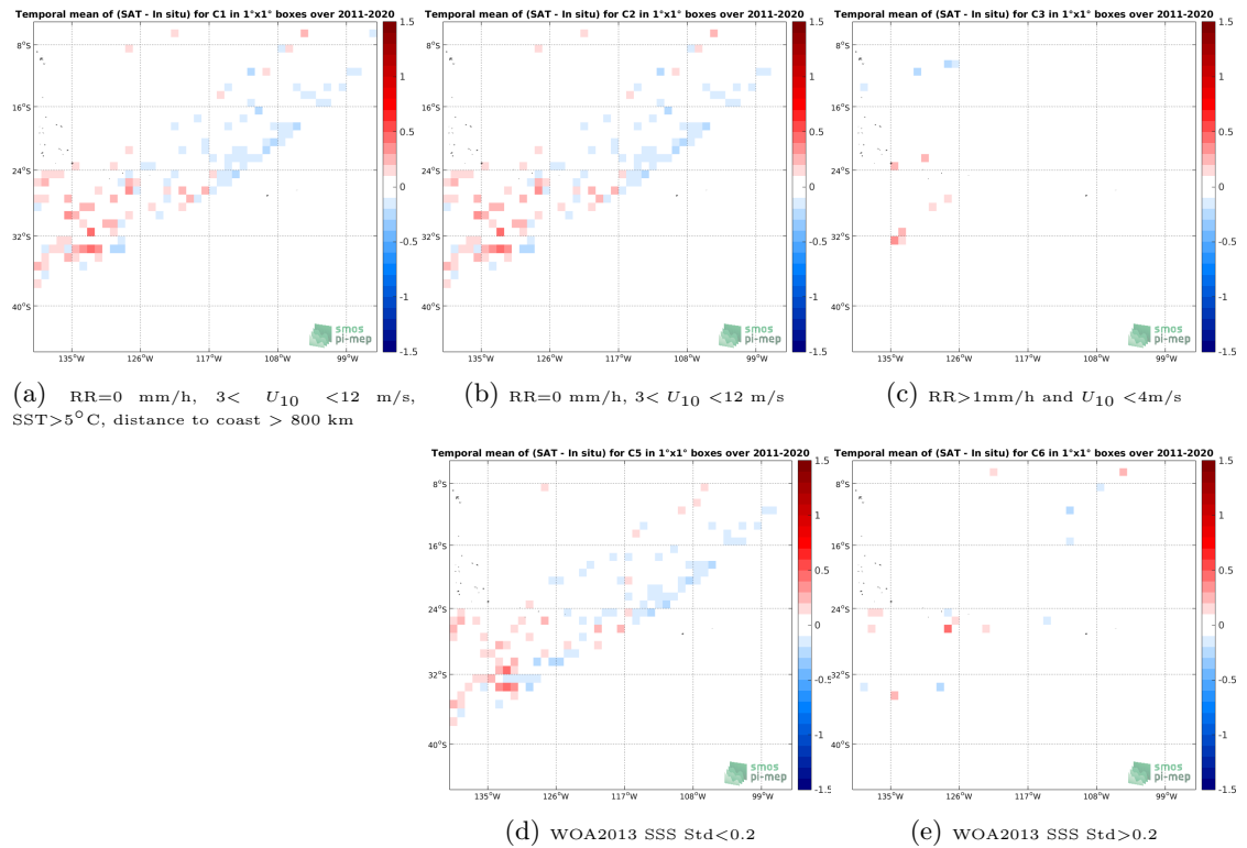
Figure 12: Temporal mean gridded over spatial boxes of size 1^\circ \times 1^\circ of \Delta SSS (SMAP SSS L4 OI v1 - 7 Days (IPRC) - TSG (LEGOS-DM)) for 5 different subdatasets corresponding to:RR=0 mm/h, 3 < U_{10} < 12 m/s, SST >5^\circ C, distance to coast > 800 km (a), RR=0 mm/h, 3 < U_{10} < 12 m/s (b), RR >1 mm/h and U_{10} < 4 m/s (c), WOA2013 SSS Std <0.2 (d), WOA2013 SSS Std >0.2 (e).
