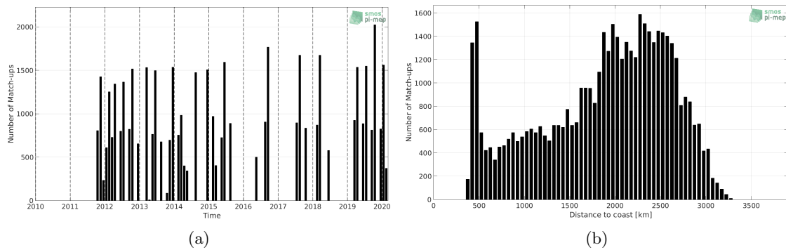
Figure 1: Number of match-ups between TSG (LEGOS-DM) and SMAP SSS L4 OI v1 - 7 Days (IPRC) SSS as a function of time (a) and as function of the distance to coast (b) over the OTT zone Pi-MEP region and for the full satellite product period.
