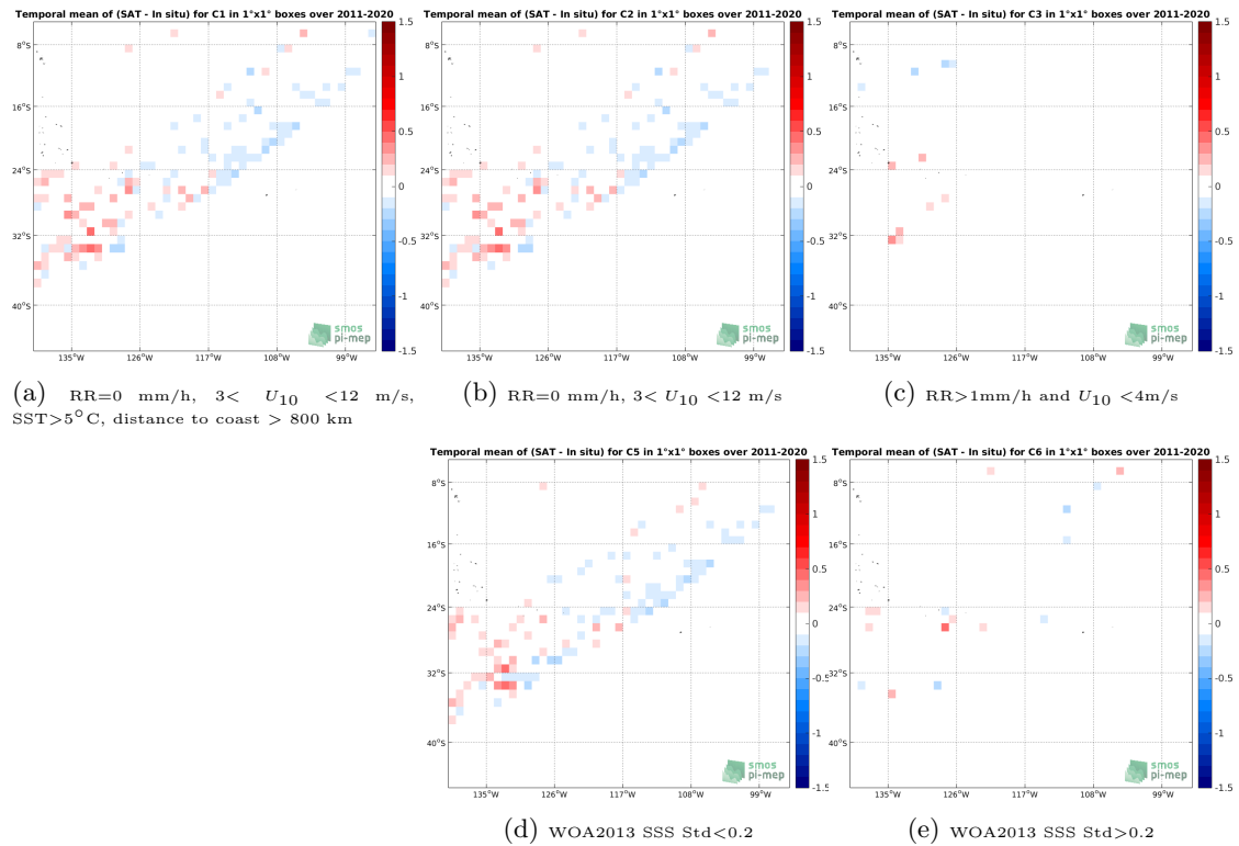
Figure 12: Temporal mean gridded over spatial boxes of size 1^\circ \times 1^\circ of \Delta\text{SSS} (SMAP SSS L4 OI v1 - 7day (IPRC) - TSG (LEGOS-DM)) for 5 different subdatasets corresponding to:RR=0 mm/h, 3 < U_{10} < 12 m/s, SST >5^\circ\text{C} , distance to coast > 800 km (a), RR=0 mm/h, 3 < U_{10} < 12 m/s (b), RR >1 mm/h and U_{10} < 4 m/s (c), WOA2013 SSS Std <0.2 (d), WOA2013 SSS Std >0.2 (e).
