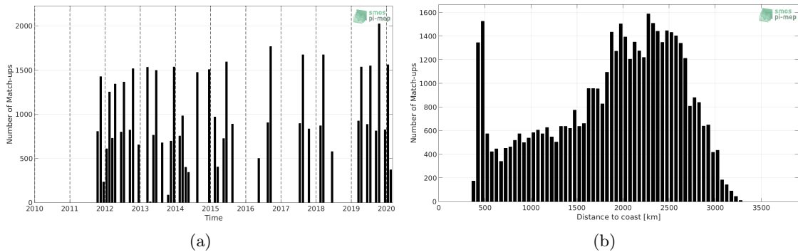
Figure 1: Number of match-ups between TSG (LEGOS-DM) and SMAP SSS L4 OI v1 - 7day (IPRC) SSS as a function of time (a) and as function of the distance to coast (b) over the OTT zone Pi-MEP region and for the full satellite product period.
