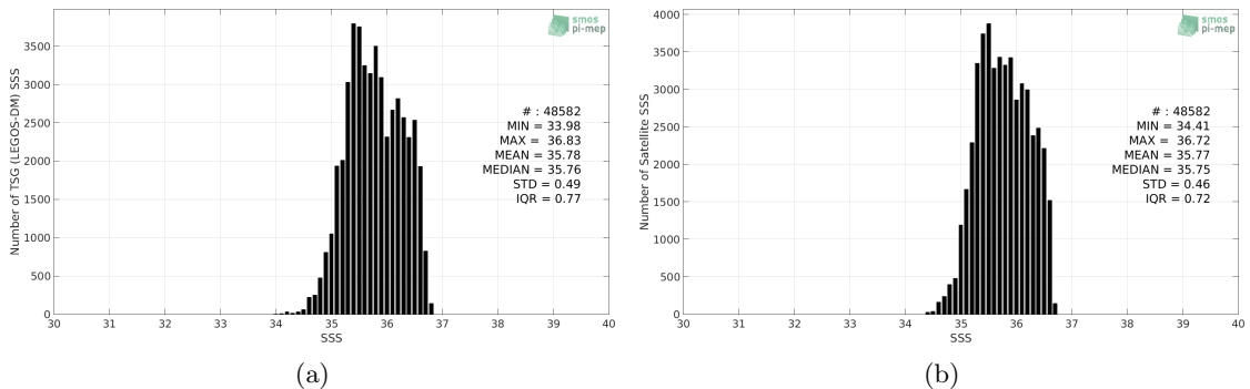
Figure 2: Histograms of SSS from TSG (LEGOS-DM) (a) and SMAP SSS L4 OI v1 - 7day (IPRC) (b) considering all match-up pairs per bins of 0.1 over the OTT zone Pi-MEP region and for the full satellite product period.
