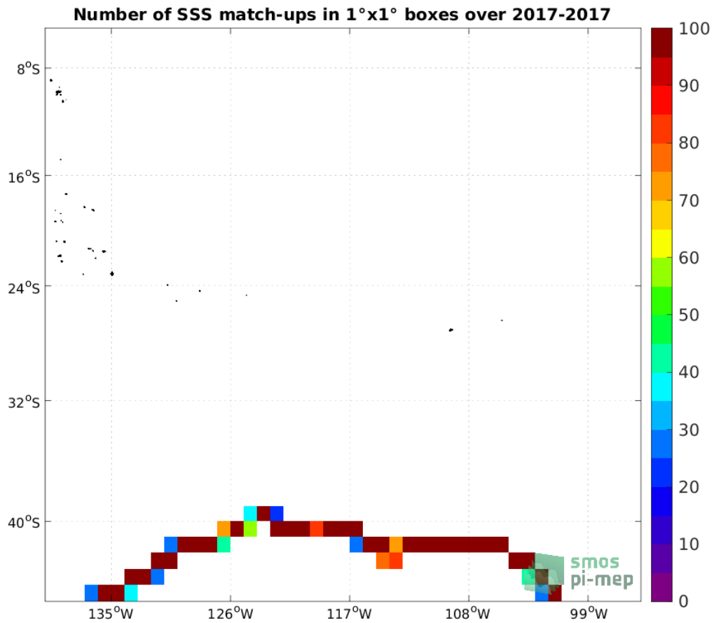
Figure 4: Number of SSS match-ups between TSG (GOSUD-Sailing-ship) SSS and the SMAP SSS L4 OI v1 - 7 Days (IPRC) SSS product for the OTT zone Pi-MEP region over 1^\circ \times 1^\circ boxes and for the full satellite product period.
