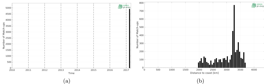
Figure 1: Number of match-ups between TSG (GOSUD-Sailing-ship) and SMAP SSS L4 OI v1 - 7 Days (IPRC) SSS as a function of time (a) and as function of the distance to coast (b) over the OTT zone Pi-MEP region and for the full satellite product period.
