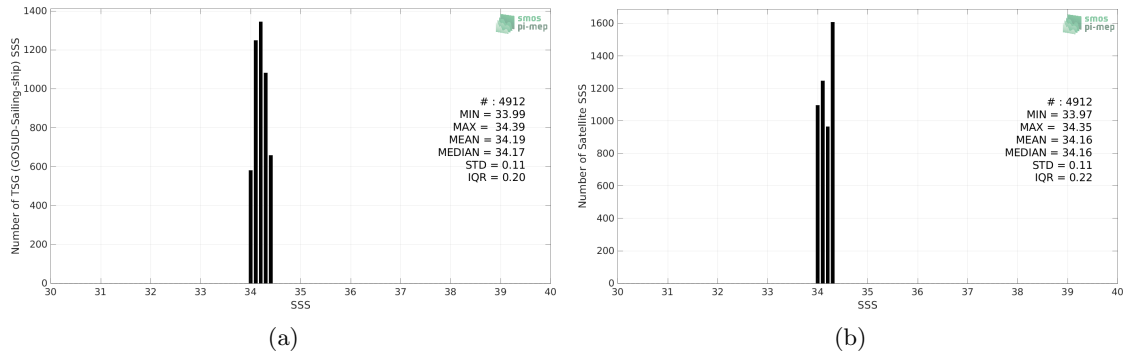
Figure 2: Histograms of SSS from TSG (GOSUD-Sailing-ship) (a) and SMAP SSS L4 OI v1 - 7 Days (IPRC) (b) considering all match-up pairs per bins of 0.1 over the OTT zone Pi-MEP region and for the full satellite product period.
