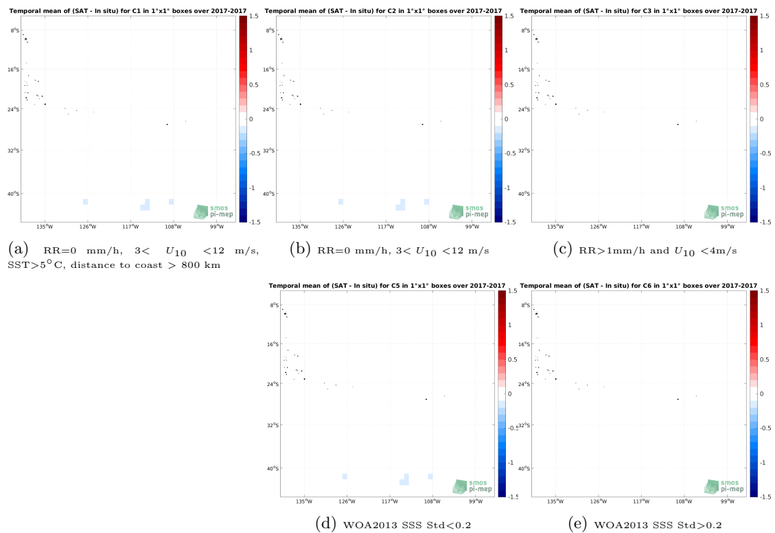
Figure 12: Temporal mean gridded over spatial boxes of size 1^\circ \times 1^\circ of \Delta SSS (SMAP SSS L4 OI v1 - 7 Days (IPRC) - TSG (GOSUD-Sailing-ship)) for 5 different subdatasets corresponding to: RR=0 mm/h, 3 < U_{10} < 12 m/s, SST > 5°C, distance to coast > 800 km (a), RR=0 mm/h, 3 < U_{10} < 12 m/s (b), RR > 1mm/h and U_{10} < 4 m/s (c), WOA2013 SSS Std < 0.2 (d), WOA2013 SSS Std > 0.2 (e).
