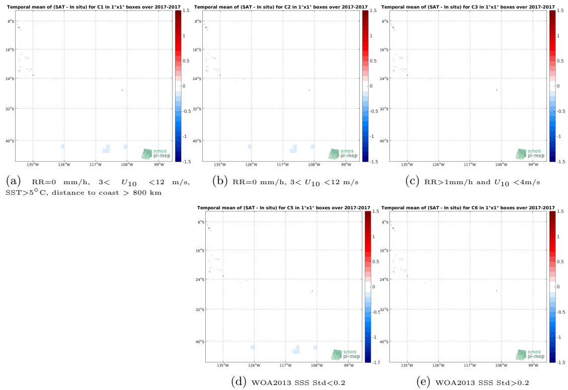
Figure 12: Temporal mean gridded over spatial boxes of size 1^\circ \times 1^\circ of \Delta\text{SSS} (SMAP SSS L4 OI v1 - 7 Days (IPRC) - TSG (GOSUD-Sailing-ship)) for 5 different subdatasets corresponding to: \text{RR}=0 \text{ mm/h} , 3 < U_{10} < 12 \text{ m/s} , \text{SST} > 5^\circ\text{C} , distance to coast > 800 \text{ km} (a), \text{RR}=0 \text{ mm/h} , 3 < U_{10} < 12 \text{ m/s} (b), \text{RR} > 1 \text{ mm/h} and U_{10} < 4 \text{ m/s} (c), WOA2013 SSS Std < 0.2 (d), WOA2013 SSS Std > 0.2 (e).
