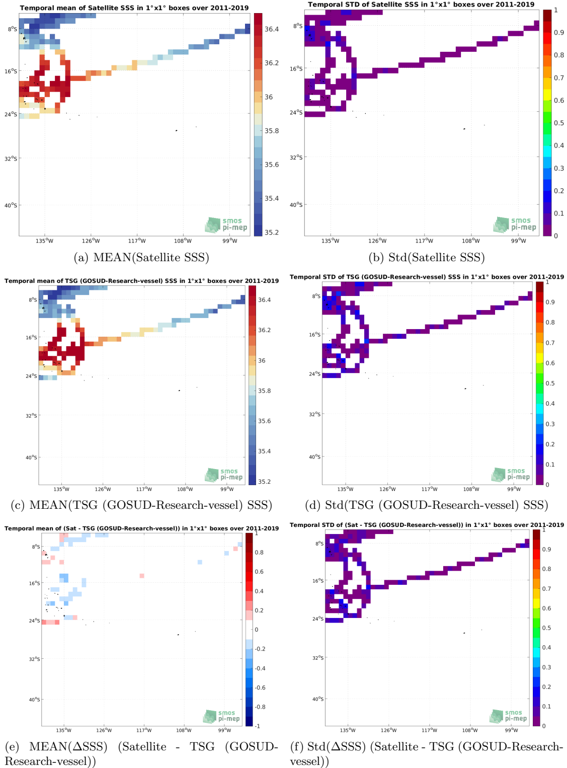
Figure 6: Temporal mean (left) and Std (right) of SSS from SMAP SSS L4 OI v1 - 7 Days (IPRC) (top), TSG (GOSUD-Research-vessel) (middle), and of \Delta SSS (Satellite - TSG (GOSUD-Research-vessel)). Only match-up pairs are used to generate these maps.
