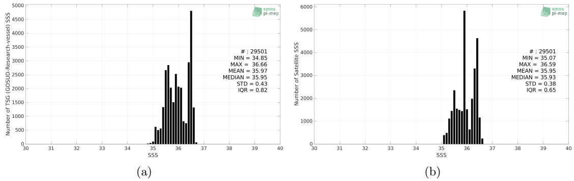
Figure 2: Histograms of SSS from TSG (GOSUD-Research-vessel) (a) and SMAP SSS L4 OI v1 - 7 Days (IPRC) (b) considering all match-up pairs per bins of 0.1 over the OTT zone Pi-MEP region and for the full satellite product period.
