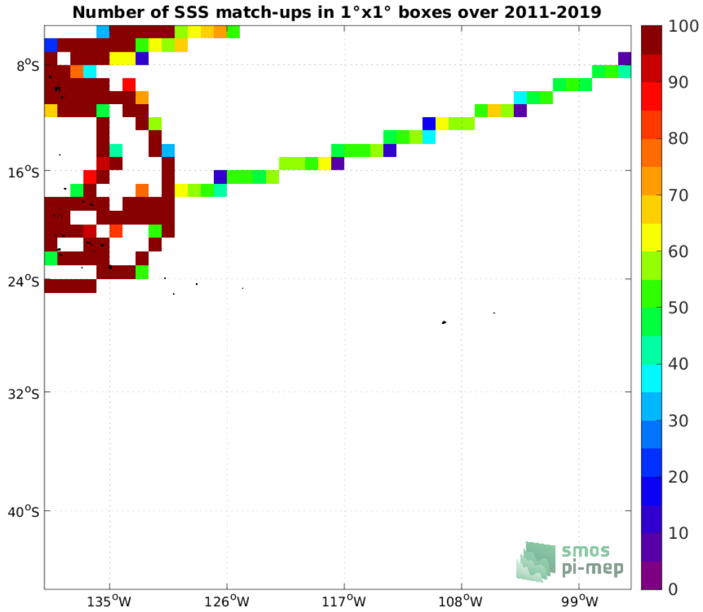
Figure 4: Number of SSS match-ups between TSG (GOSUD-Research-vessel) SSS and the SMAP SSS L4 OI v1 - 7 Days (IPRC) SSS product for the OTT zone Pi-MEP region over 1^\circ \times 1^\circ boxes and for the full satellite product period.
