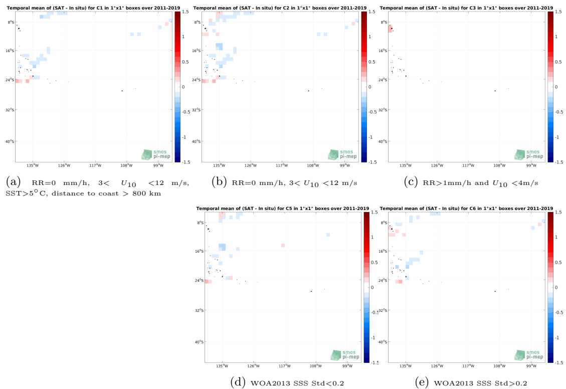
Figure 12: Temporal mean gridded over spatial boxes of size 1^\circ \times 1^\circ of \Delta SSS (SMAP SSS L4 OI v1 - 7 Days (IPRC) - TSG (GOSUD-Research-vessel)) for 5 different subdatasets corresponding to:RR=0 mm/h, 3 < U_{10} < 12 m/s, SST >5^\circ\text{C} , distance to coast > 800 km (a), RR=0 mm/h, 3 < U_{10} < 12 m/s (b), RR >1 mm/h and U_{10} < 4 m/s (c), WOA2013 SSS Std <0.2 (d), WOA2013 SSS Std >0.2 (e).
