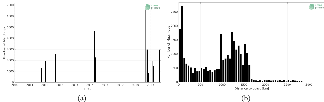
Figure 1: Number of match-ups between TSG (GOSUD-Research-vessel) and SMAP SSS L4 OI v1 - 7 Days (IPRC) SSS as a function of time (a) and as function of the distance to coast (b) over the OTT zone Pi-MEP region and for the full satellite product period.
