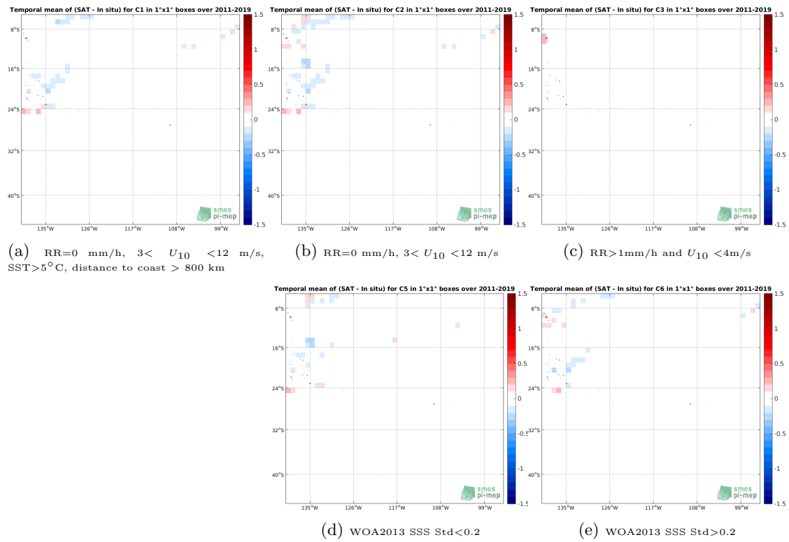
Figure 12: Temporal mean gridded over spatial boxes of size 1^\circ \times 1^\circ of \Delta SSS (SMAP SSS L4 OI v1 - 7 Days (IPRC) - TSG (GOSUD-Research-vessel)) for 5 different subdatasets corresponding to:RR=0 mm/h, 3 < U_{10} < 12 m/s, SST>5°C, distance to coast > 800 km (a), RR=0 mm/h, 3 < U_{10} < 12 m/s (b), RR>1mm/h and U_{10} < 4 m/s (c), WOA2013 SSS Std<0.2 (d), WOA2013 SSS Std>0.2 (e).
