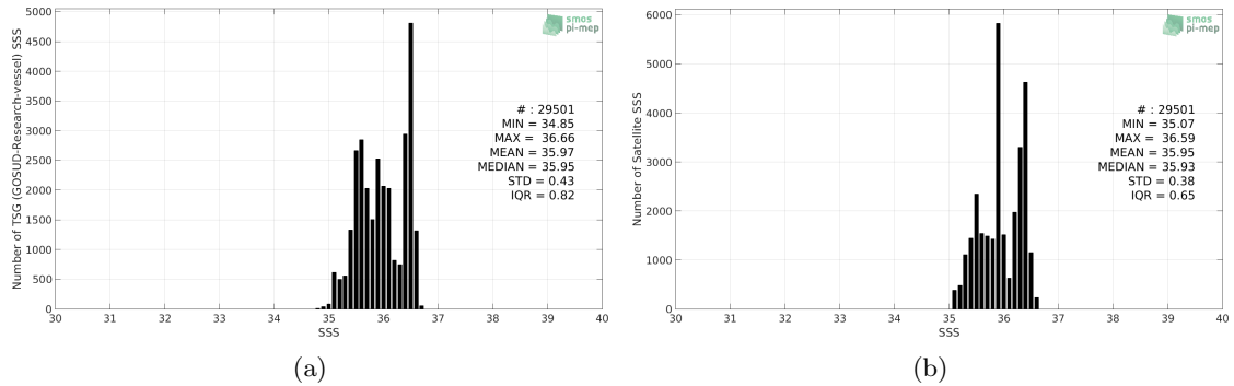
Figure 2: Histograms of SSS from TSG (GOSUD-Research-vessel) (a) and SMAP SSS L4 OI v1 - 7day (IPRC) (b) considering all match-up pairs per bins of 0.1 over the OTT zone Pi-MEP region and for the full satellite product period.
