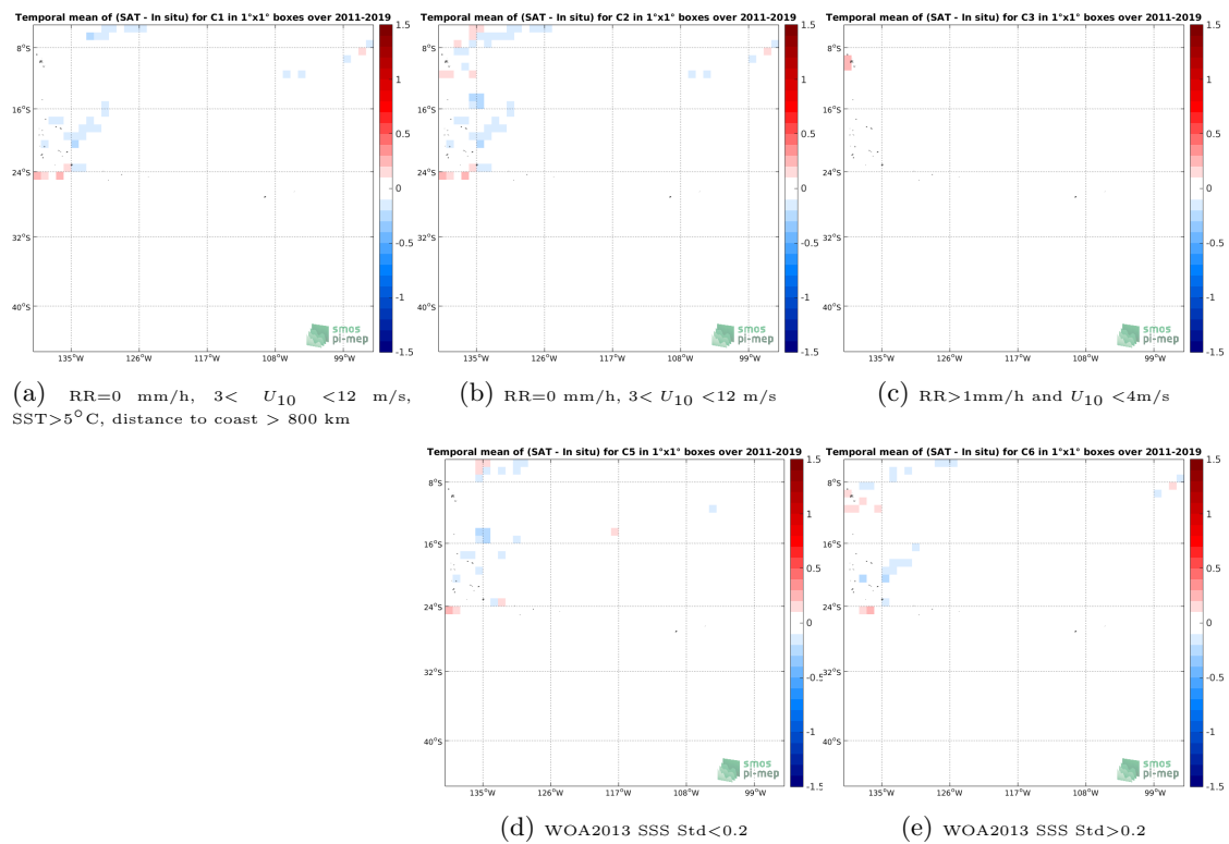
Figure 12: Temporal mean gridded over spatial boxes of size 1^\circ \times 1^\circ of \Delta SSS (SMAP SSS L4 OI v1 - 7day (IPRC) - TSG (GOSUD-Research-vessel)) for 5 different subdatasets corresponding to: RR=0 mm/h, 3 < U_{10} < 12 m/s, SST > 5^\circ C , distance to coast > 800 km (a), RR=0 mm/h, 3 < U_{10} < 12 m/s (b), RR > 1 mm/h and U_{10} < 4 m/s (c), WOA2013 SSS Std < 0.2 (d), WOA2013 SSS Std > 0.2 (e).
