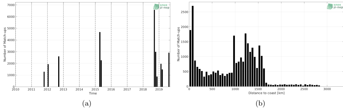
Figure 1: Number of match-ups between TSG (GOSUD-Research-vessel) and SMAP SSS L4 OI v1 - 7day (IPRC) SSS as a function of time (a) and as function of the distance to coast (b) over the OTT zone Pi-MEP region and for the full satellite product period.
