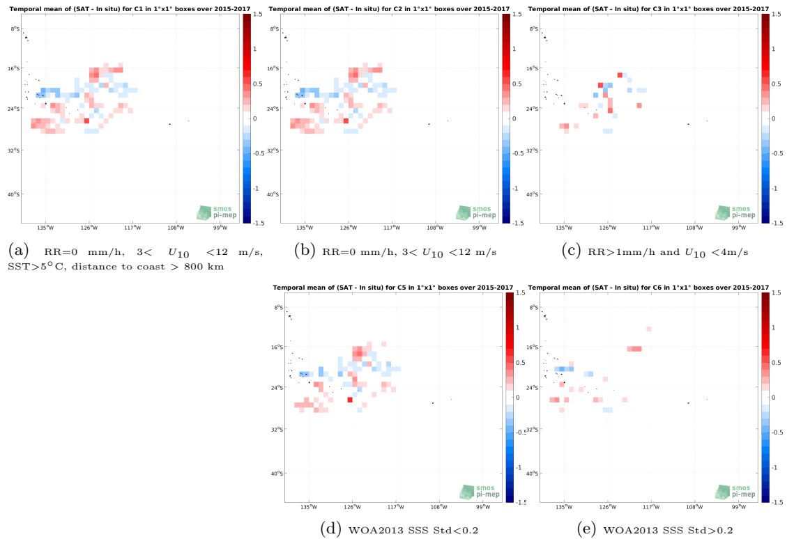
Figure 11: Temporal mean gridded over spatial boxes of size 1^\circ \times 1^\circ of \Delta SSS (SMAP SSS L4 OI v1 - 7 Days (IPRC) - Surface drifters) for 5 different subdatasets corresponding to:RR=0 mm/h, 3 < U_{10} < 12 m/s, SST > 5^\circ\text{C} , distance to coast > 800 km (a), RR=0 mm/h, 3 < U_{10} < 12 m/s (b), RR > 1 mm/h and U_{10} < 4 m/s (c), WOA2013 SSS Std < 0.2 (d), WOA2013 SSS Std > 0.2 (e).
