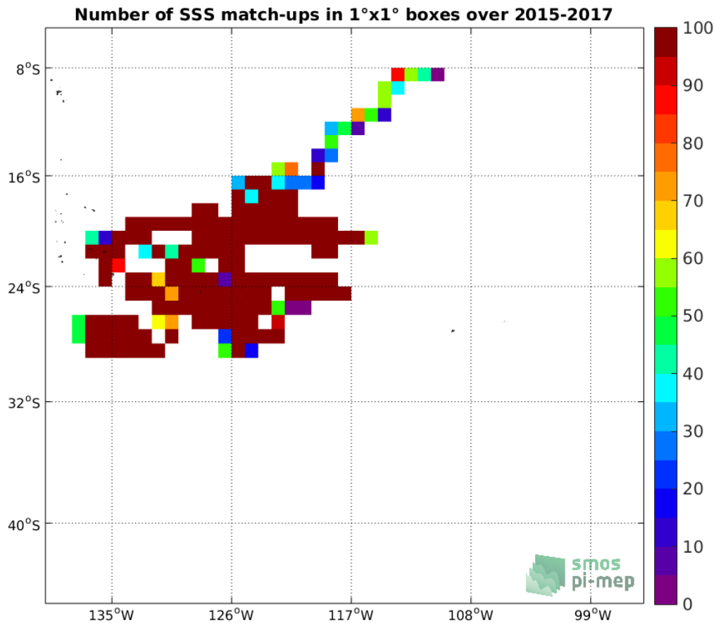
Figure 3: Number of SSS match-ups between Surface drifters SSS and the SMAP SSS L4 OI v1 - 7 Days (IPRC) SSS product for the OTT zone Pi-MEP region over 1^\circ \times 1^\circ boxes and for the full satellite product period.
