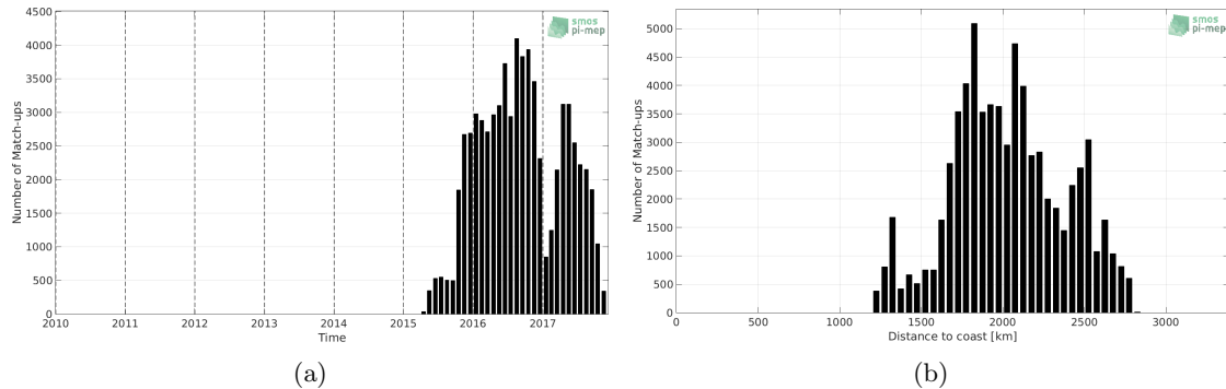
Figure 1: Number of match-ups between Surface drifters and SMAP SSS L4 OI v1 - 7 Days (IPRC) SSS as a function of time (a) and as function of the distance to coast (b) over the OTT zone Pi-MEP region and for the full satellite product period.
