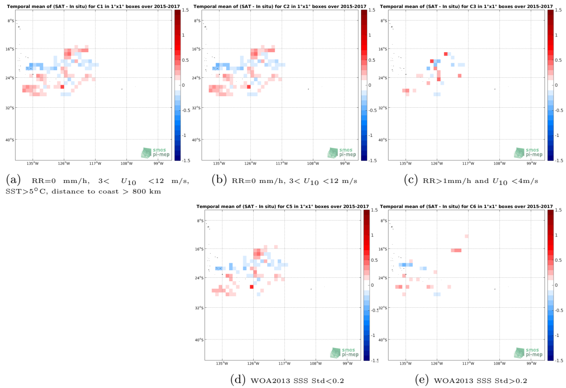
Figure 11: Temporal mean gridded over spatial boxes of size 1^\circ \times 1^\circ of \Delta\text{SSS} (SMAP SSS L4 OI v1 - 7 Days (IPRC) - Surface drifters) for 5 different subdatasets corresponding to:RR=0 mm/h, 3 < U_{10} < 12 m/s, SST >5^\circ\text{C} , distance to coast > 800 km (a), RR=0 mm/h, 3 < U_{10} < 12 m/s (b), RR >1 mm/h and U_{10} < 4 m/s (c), WOA2013 SSS Std <0.2 (d), WOA2013 SSS Std >0.2 (e).
