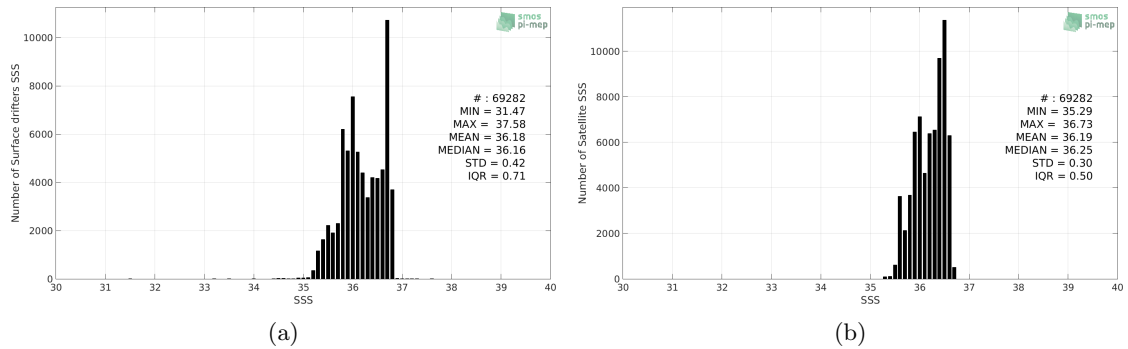
Figure 2: Histograms of SSS from Surface drifters (a) and SMAP SSS L4 OI v1 - 7 Days (IPRC) (b) considering all match-up pairs per bins of 0.1 over the OTT zone Pi-MEP region and for the full satellite product period.
