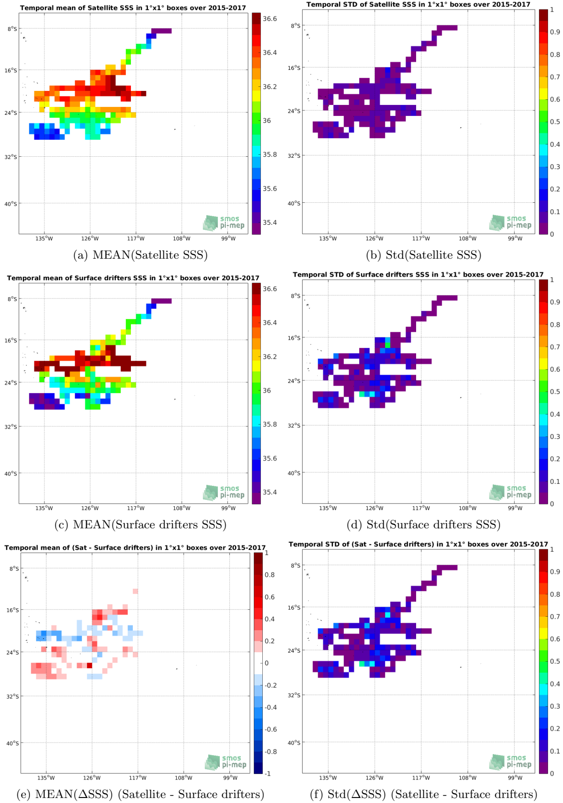
Figure 5: Temporal mean (left) and Std (right) of SSS from SMAP SSS L4 OI v1 - 7 Days (IPRC) (top), Surface drifters (middle), and of \Delta SSS (Satellite - Surface drifters). Only match-up pairs are used to generate these maps.
