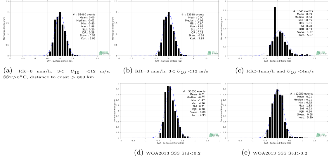
Figure 12: Normalized histogram of \Delta SSS (SMAP SSS L4 OI v1 - 7 Days (IPRC) - Surface drifters) for 5 different subdatasets corresponding to: RR=0 mm/h, 3 < U_{10} < 12 m/s, SST > 5°C, distance to coast > 800 km (a), RR=0 mm/h, 3 < U_{10} < 12 m/s (b), RR > 1mm/h and U_{10} < 4 m/s (c), WOA2013 SSS Std < 0.2 (d), WOA2013 SSS Std > 0.2 (e).
