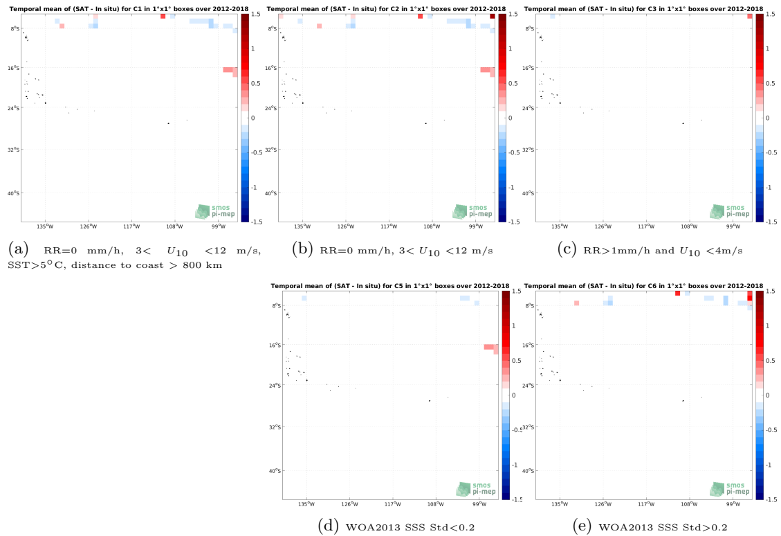
Figure 12: Temporal mean gridded over spatial boxes of size 1^\circ \times 1^\circ of \Delta SSS (SMAP SSS L4 OI v1 - Monthly (IPRC) - TSG (SAMOS)) for 5 different subdatasets corresponding to:RR=0 mm/h, 3 < U_{10} < 12 m/s, SST >5^\circ C, distance to coast > 800 km (a), RR=0 mm/h, 3 < U_{10} < 12 m/s (b), RR >1 mm/h and U_{10} < 4 m/s (c), WOA2013 SSS Std <0.2 (d), WOA2013 SSS Std >0.2 (e).
