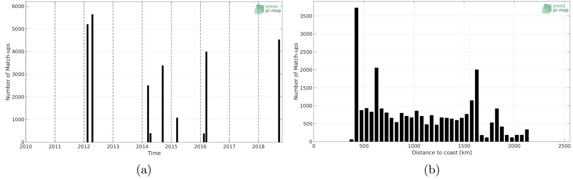
Figure 1: Number of match-ups between TSG (SAMOS) and SMAP SSS L4 OI v1 - Monthly (IPRC) SSS as a function of time (a) and as function of the distance to coast (b) over the OTT zone Pi-MEP region and for the full satellite product period.
