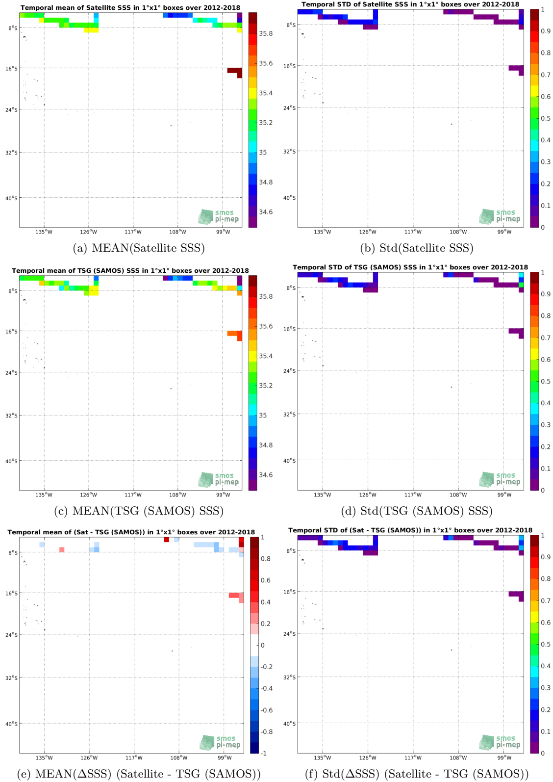
Figure 6: Temporal mean (left) and Std (right) of SSS from SMAP SSS L4 OI v1 - Monthly (IPRC) (top), TSG (SAMOS) (middle), and of \Delta SSS (Satellite - TSG (SAMOS)). Only match-up pairs are used to generate these maps.
