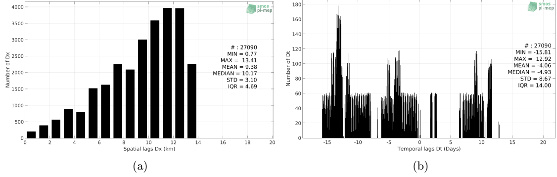
Figure 5: Histograms of the spatial (a) and temporal (b) lags between the location/time of the TSG (SAMOS) measurement and the date of the corresponding SMAP SSS L4 OI v1 - Monthly (IPRC) SSS pixel.
