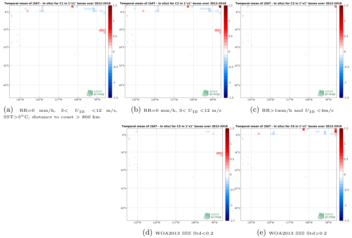
Figure 12: Temporal mean gridded over spatial boxes of size 1^\circ \times 1^\circ of \Delta SSS (SMAP SSS L4 OI v1 - Monthly (IPRC) - TSG (SAMOS)) for 5 different subdatasets corresponding to: RR=0 mm/h, 3 < U_{10} < 12 m/s, SST > 5^\circ C , distance to coast > 800 km (a), RR=0 mm/h, 3 < U_{10} < 12 m/s (b), RR > 1 mm/h and U_{10} < 4 m/s (c), WOA2013 SSS Std < 0.2 (d), WOA2013 SSS Std > 0.2 (e).
