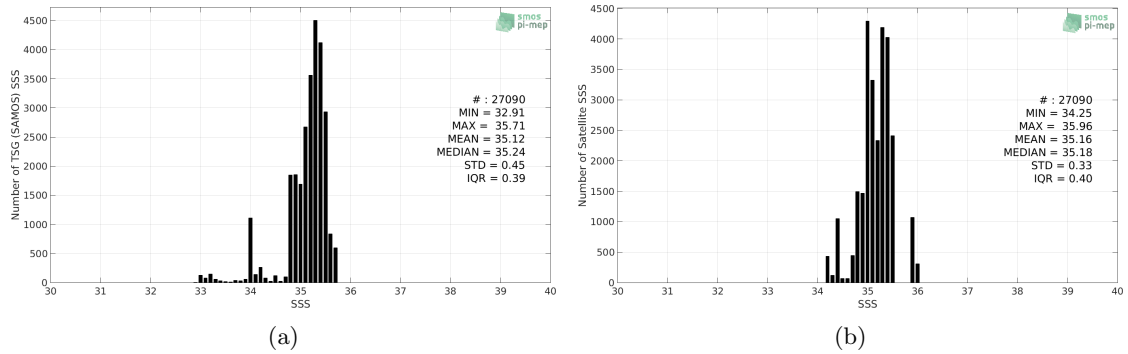
Figure 2: Histograms of SSS from TSG (SAMOS) (a) and SMAP SSS L4 OI v1 - Monthly (IPRC) (b) considering all match-up pairs per bins of 0.1 over the OTT zone Pi-MEP region and for the full satellite product period.
