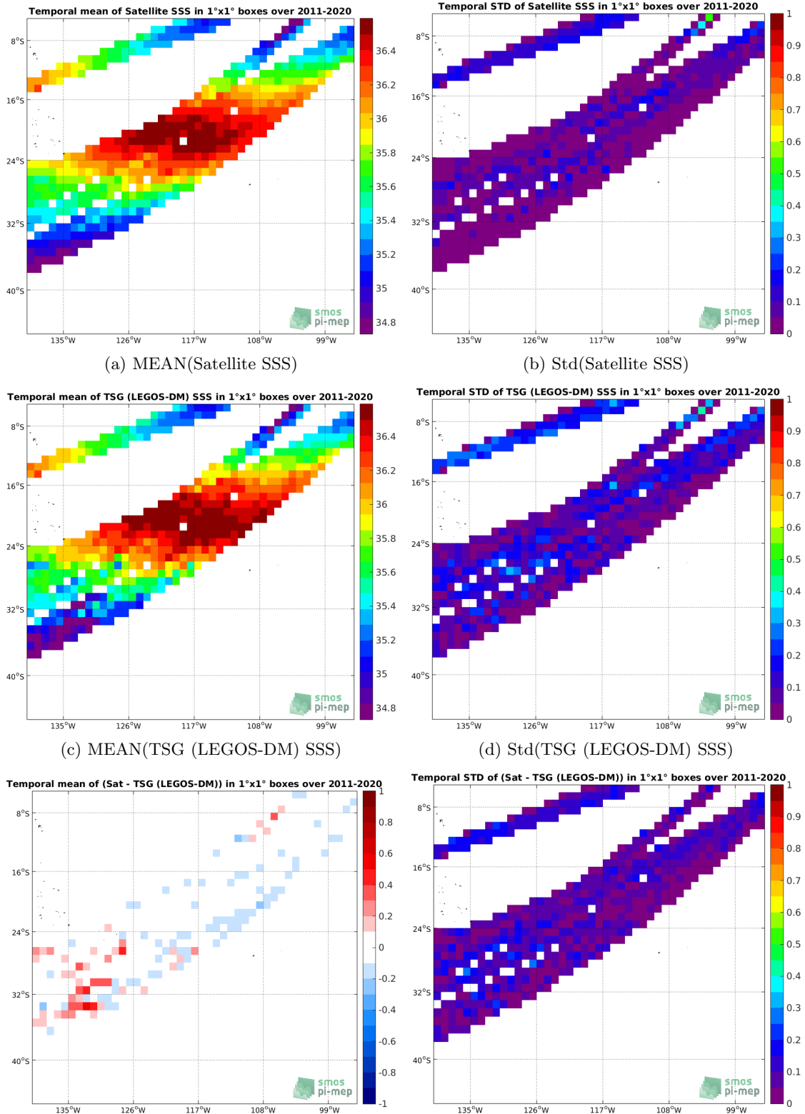
Figure 6: Temporal mean (left) and Std (right) of SSS from SMAP SSS L4 OI v1 - Monthly (IPRC) (top), TSG (LEGOS-DM) (middle), and \Delta SSS (Satellite - TSG (LEGOS-DM)). Only match-up pairs are used to generate these maps.
