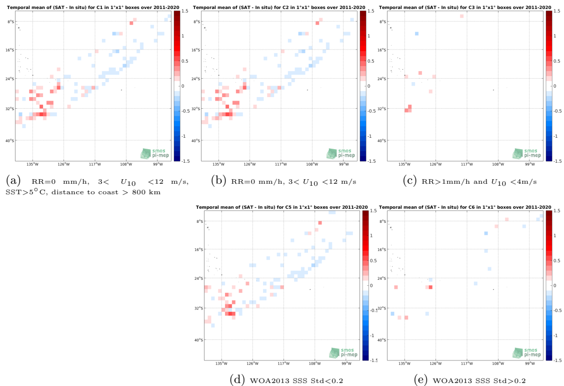
Figure 12: Temporal mean gridded over spatial boxes of size 1^\circ \times 1^\circ of \Delta SSS (SMAP SSS L4 OI v1 - Monthly (IPRC) - TSG (LEGOS-DM)) for 5 different subdatasets corresponding to: RR=0 mm/h, 3 < U_{10} < 12 m/s, SST > 5^\circ C , distance to coast > 800 km (a), RR=0 mm/h, 3 < U_{10} < 12 m/s (b), RR > 1 mm/h and U_{10} < 4 m/s (c), WOA2013 SSS Std < 0.2 (d), WOA2013 SSS Std > 0.2 (e).
