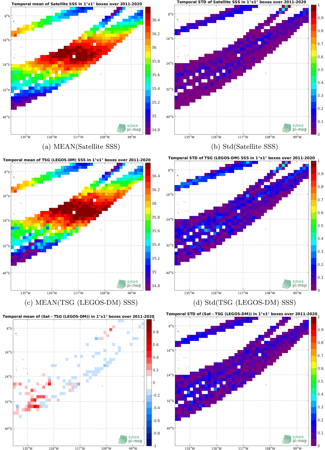
(e) MEAN( \Delta SSS) (Satellite - TSG (LEGOS-DM)) (f) Std( \Delta SSS) (Satellite - TSG (LEGOS-DM))
