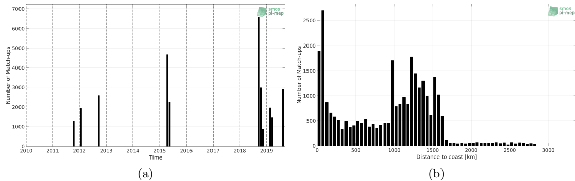
Figure 1: Number of match-ups between TSG (GOSUD-Research-vessel) and SMAP SSS L4 OI v1 - Monthly (IPRC) SSS as a function of time (a) and as function of the distance to coast (b) over the OTT zone Pi-MEP region and for the full satellite product period.
