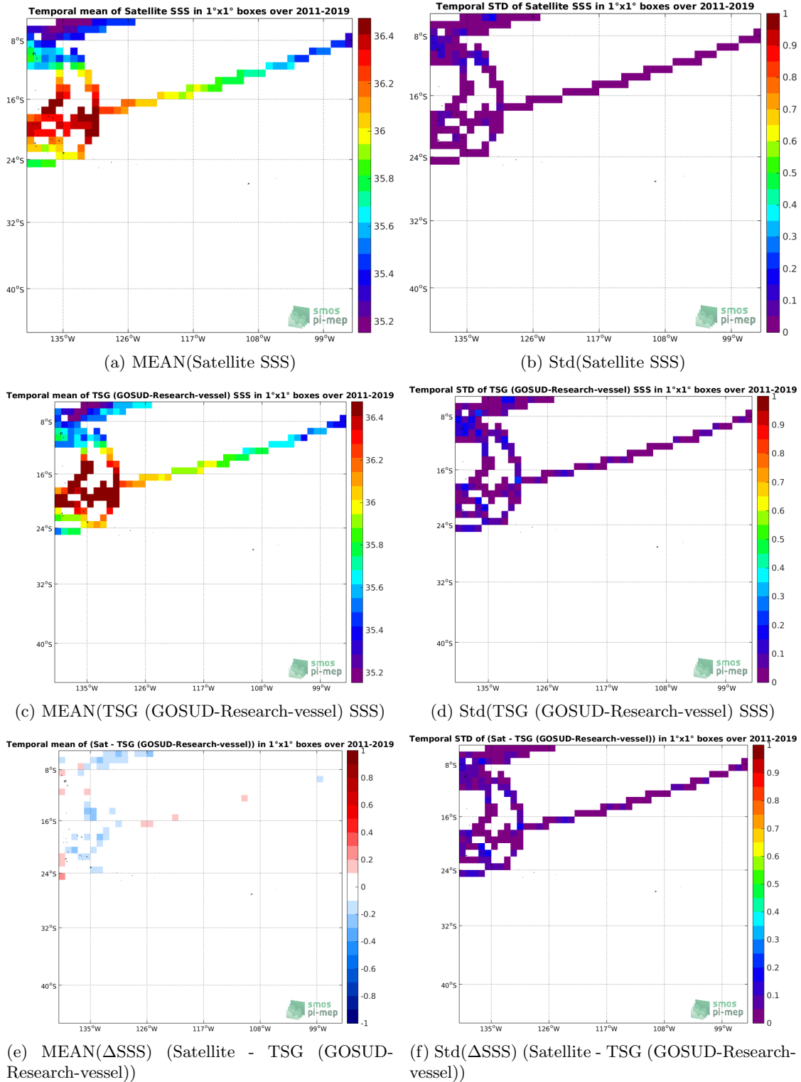
Figure 6: Temporal mean (left) and Std (right) of SSS from SMAP SSS L4 OI v1 - Monthly (IPRC) (top), TSG (GOSUD-Research-vessel) (middle), and of \Delta SSS (Satellite - TSG (GOSUD-Research-vessel)). Only match-up pairs are used to generate these maps.
