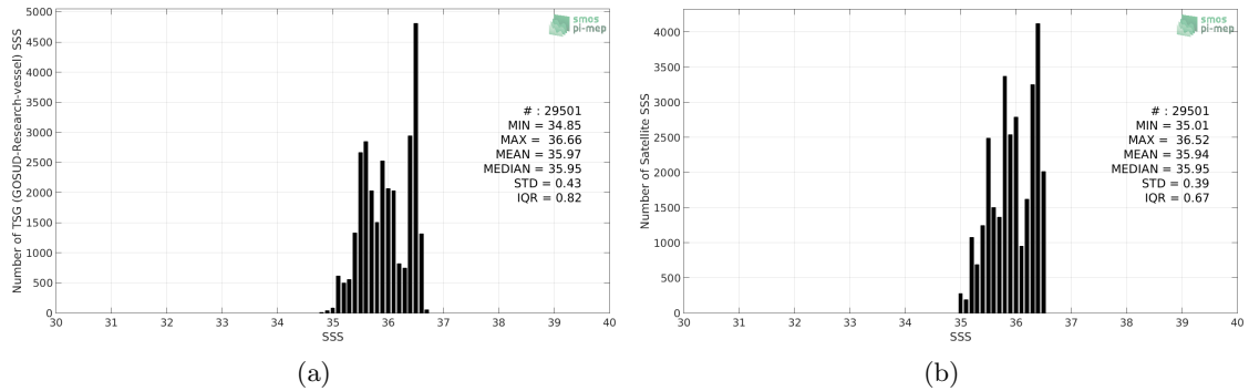
Figure 2: Histograms of SSS from TSG (GOSUD-Research-vessel) (a) and SMAP SSS L4 OI v1 - Monthly (IPRC) (b) considering all match-up pairs per bins of 0.1 over the OTT zone Pi-MEP region and for the full satellite product period.
