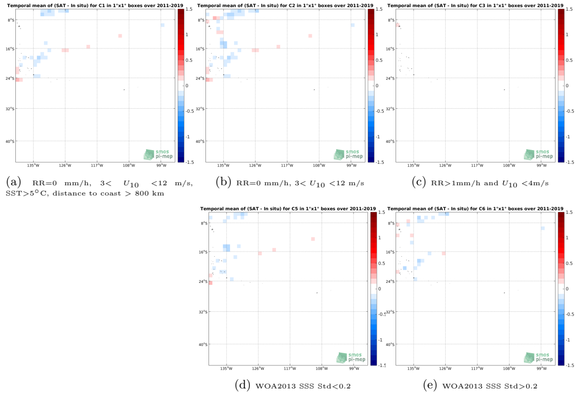
Figure 12: Temporal mean gridded over spatial boxes of size 1^\circ \times 1^\circ of \Delta\text{SSS} (SMAP SSS L4 OI v1 - Monthly (IPRC) - TSG (GOSUD-Research-vessel)) for 5 different subdatasets corresponding to: RR=0 mm/h, 3 < U_{10} < 12 m/s, SST > 5°C, distance to coast > 800 km (a), RR=0 mm/h, 3 < U_{10} < 12 m/s (b), RR > 1mm/h and U_{10} < 4 m/s (c), WOA2013 SSS Std < 0.2 (d), WOA2013 SSS Std > 0.2 (e).
