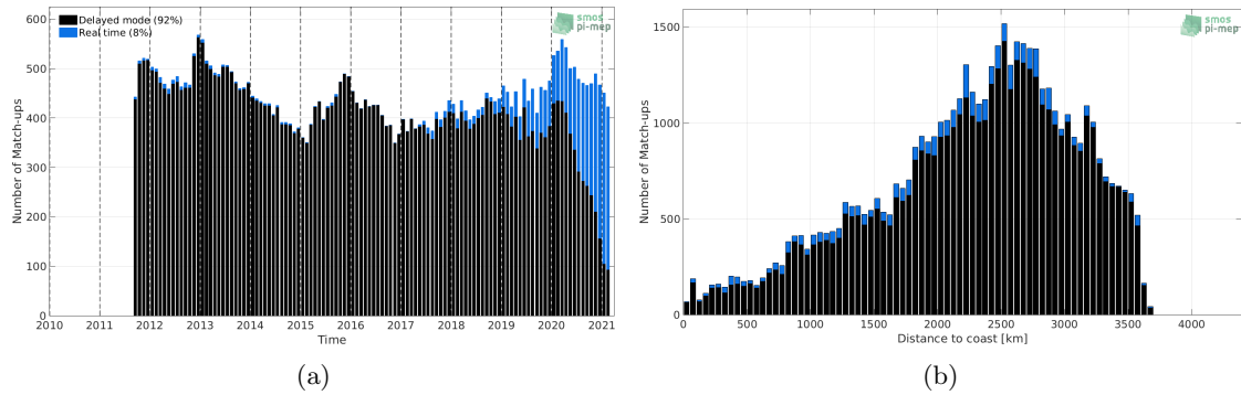
Figure 1: Number of match-ups between Argo and SMAP SSS L4 OI v1 - Monthly (IPRC) SSS as a function of time (a) and as function of the distance to coast (b) over the OTT zone Pi-MEP region and for the full satellite product period.
