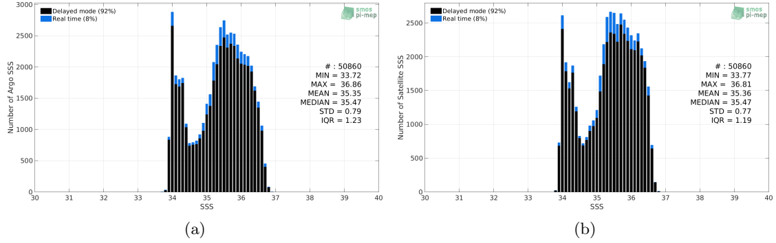
Figure 2: Histograms of SSS from Argo (a) and SMAP SSS L4 OI v1 - Monthly (IPRC) (b) considering all match-up pairs per bins of 0.1 over the OTT zone Pi-MEP region and for the full satellite product period.
