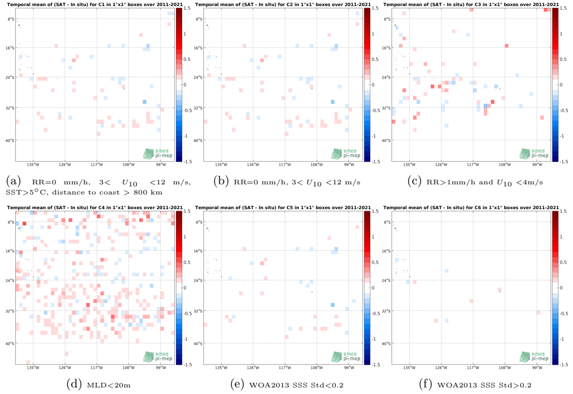
Figure 12: Temporal mean gridded over spatial boxes of size 1^\circ \times 1^\circ of \Delta SSS (SMAP SSS L4 OI v1 - Monthly (IPRC) - Argo) for 6 different subdatasets corresponding to:RR=0 mm/h, 3 < U_{10} < 12 m/s, SST >5^\circ\text{C} , distance to coast > 800 km (a), RR=0 mm/h, 3 < U_{10} < 12 m/s (b), RR >1 mm/h and U_{10} < 4 m/s (c),MLD <20 m (d),WOA2013 SSS Std <0.2 (e),WOA2013 SSS Std >0.2 (f).
