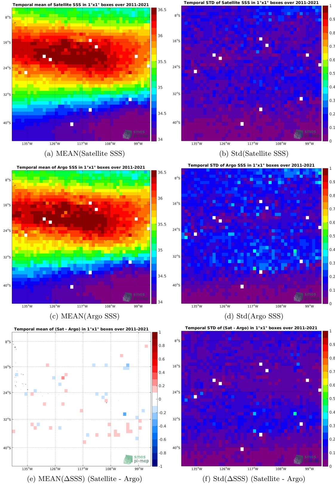
Figure 6: Temporal mean (left) and Std (right) of SSS from SMAP SSS L4 OI v1 - Monthly (IPRC) (top), Argo (middle), and of \Delta SSS (Satellite - Argo). Only match-up pairs are used to generate these maps.
