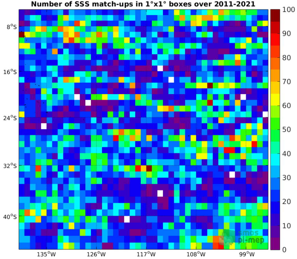
Figure 4: Number of SSS match-ups between Argo SSS and the SMAP SSS L4 OI v1 - Monthly (IPRC) SSS product for the OTT zone Pi-MEP region over 1^\circ \times 1^\circ boxes and for the full satellite product period.
