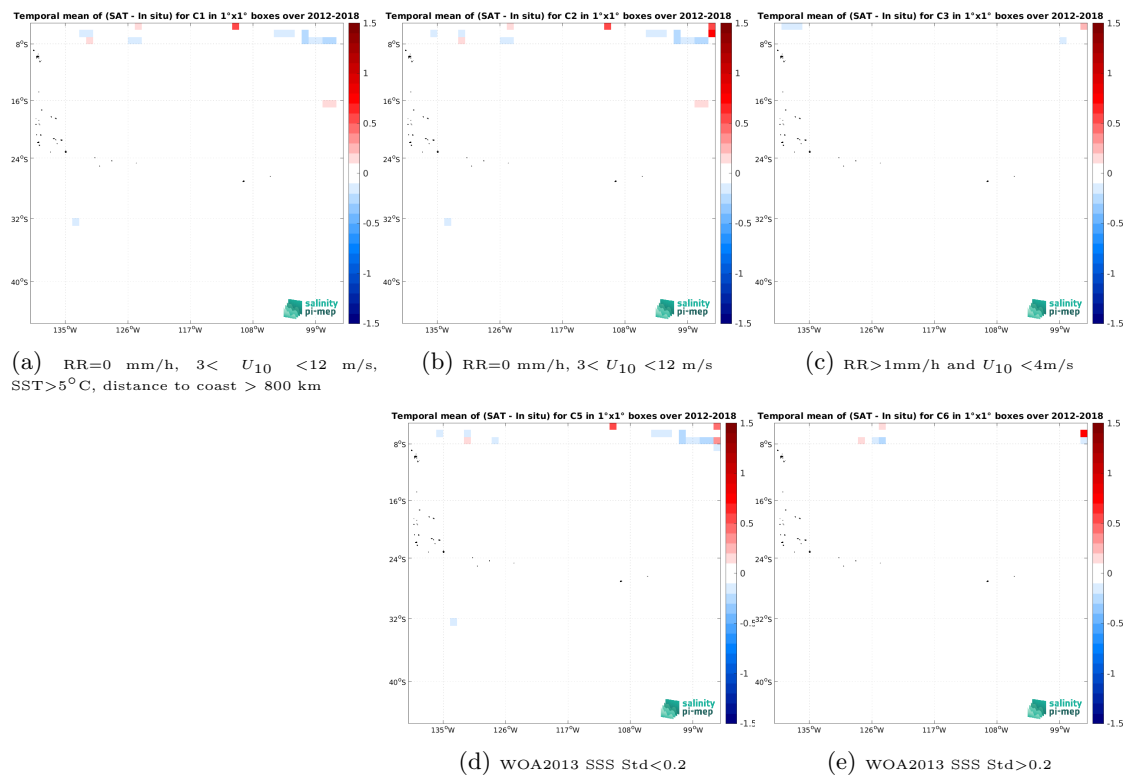
Figure 14: Temporal mean gridded over spatial boxes of size 1^\circ \times 1^\circ of \Delta SSS (SMAP SSS L4 OI v3 - Monthly (ESR) - TSG (SAMOS)) for 5 different subdatasets corresponding to:RR=0 mm/h, 3 < U_{10} < 12 m/s, SST>5°C, distance to coast > 800 km (a), RR=0 mm/h, 3 < U_{10} < 12 m/s (b), RR>1mm/h and U_{10} < 4 m/s (c), WOA2013 SSS Std<0.2 (d), WOA2013 SSS Std>0.2 (e).
