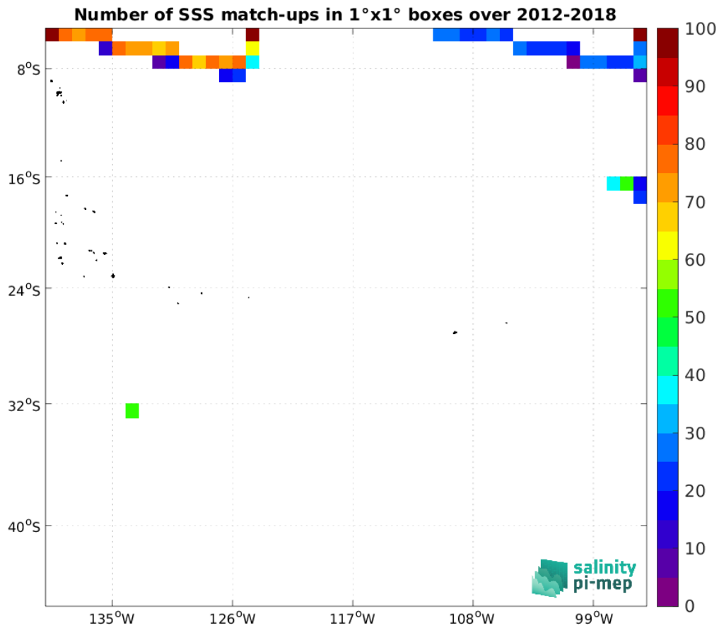
Figure 5: Number of SSS match-ups between TSG (SAMOS) SSS and the SMAP SSS L4 OI v3 - Monthly (ESR) SSS product for the OTT zone Pi-MEP region over 1^\circ \times 1^\circ boxes and for the full satellite product period.
