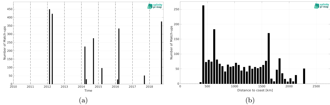
Figure 2: Number of match-ups between TSG (SAMOS) and SMAP SSS L4 OI v3 - Monthly (ESR) SSS as a function of time (a) and as function of the distance to coast (b) over the OTT zone Pi-MEP region and for the full satellite product period.
