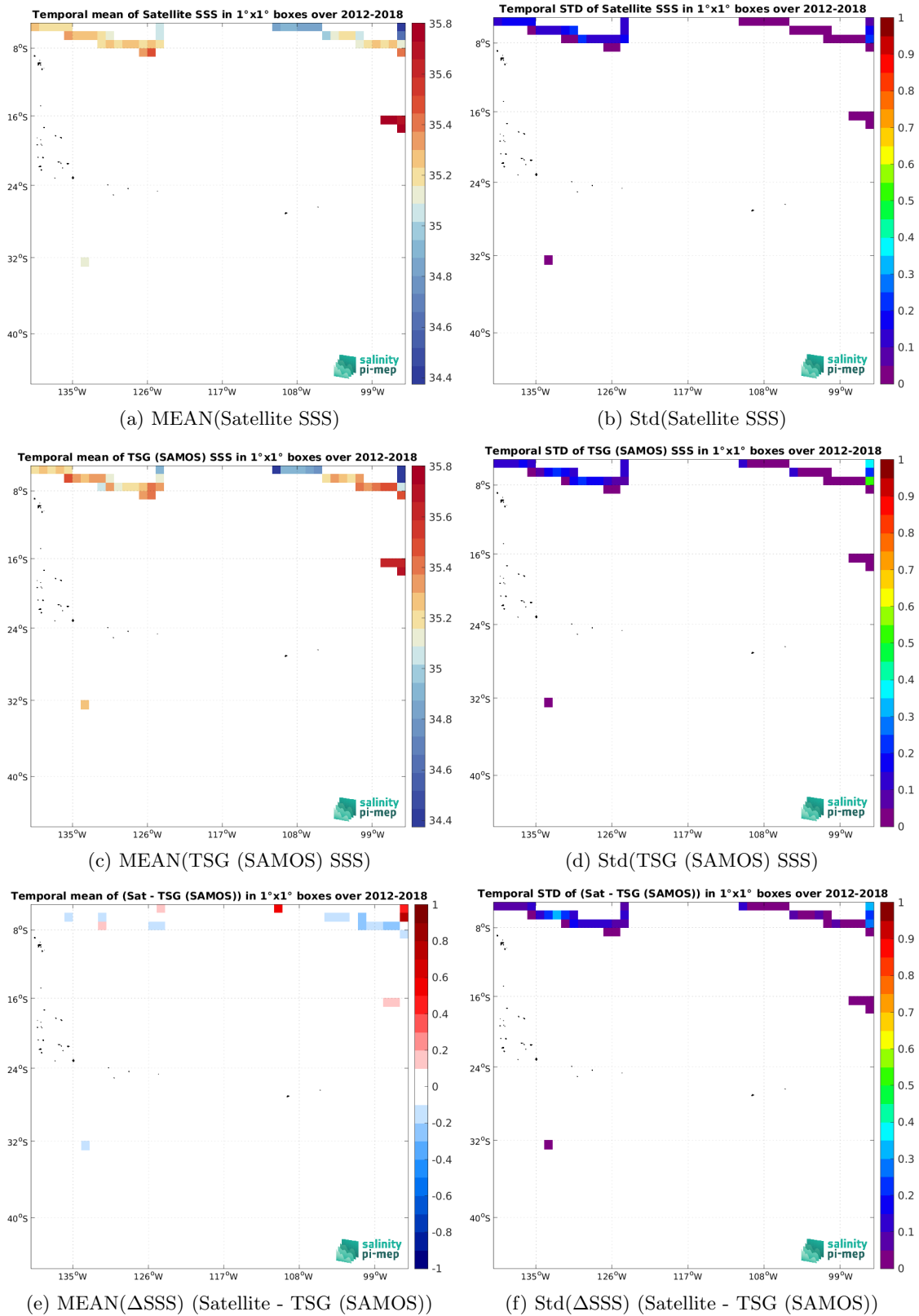
Figure 7: Temporal mean (left) and Std (right) of SSS from SMAP SSS L4 OI v3 - Monthly (ESR) (top), TSG (SAMOS) (middle), and of \Delta SSS (Satellite - TSG (SAMOS)). Only match-up pairs are used to generate these maps.
