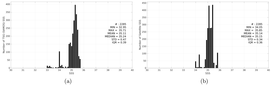
Figure 3: Histograms of SSS from TSG (SAMOS) (a) and SMAP SSS L4 OI v3 - Monthly (ESR) (b) considering all match-up pairs per bins of 0.1 over the OTT zone Pi-MEP region and for the full satellite product period.
