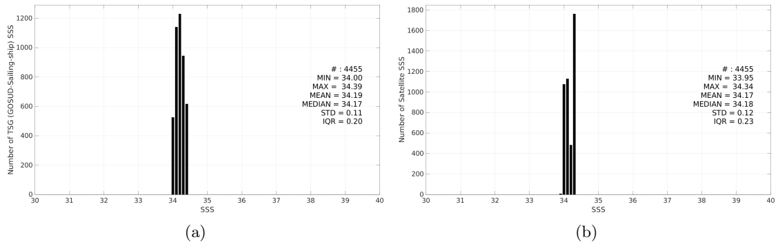
Figure 3: Histograms of SSS from TSG (GOSUD-Sailing-ship) (a) and SMAP SSS L4 OI v3 - Monthly (ESR) (b) considering all match-up pairs per bins of 0.1 over the OTT zone Pi-MEP region and for the full satellite product period.
