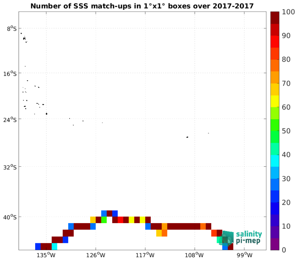
Figure 5: Number of SSS match-ups between TSG (GOSUD-Sailing-ship) SSS and the SMAP SSS L4 OI v3 - Monthly (ESR) SSS product for the OTT zone Pi-MEP region over 1°x1° boxes and for the full satellite product period.
