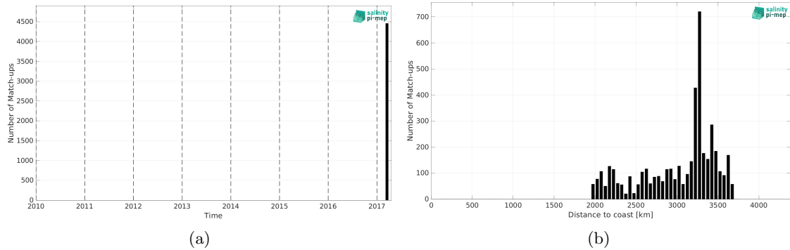
Figure 2: Number of match-ups between TSG (GOSUD-Sailing-ship) and SMAP SSS L4 OI v3 - Monthly (ESR) SSS as a function of time (a) and as function of the distance to coast (b) over the OTT zone Pi-MEP region and for the full satellite product period.
