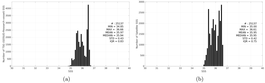
Figure 3: Histograms of SSS from TSG (GOSUD-Research-vessel) (a) and SMAP SSS L4 OI v3 - Monthly (ESR) (b) considering all match-up pairs per bins of 0.1 over the OTT zone Pi-MEP region and for the full satellite product period.
