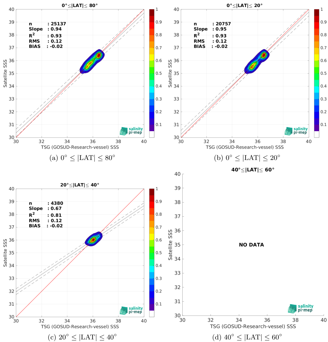
Figure 10: Contour maps of the concentration of SMAP SSS L4 OI v3 - Monthly (ESR) SSS (y-axis) versus TSG (GOSUD-Research-vessel) SSS (x-axis) at match-up pairs for different latitude bands. For each plot, the red line shows x=y . The black thin and dashed lines indicate a linear fit through the data cloud and the \pm 95\% confidence levels, respectively. The number match-up pairs n , the slope and R^2 coefficient of the linear fit, the root mean square (RMS) and the mean bias between satellite and in situ data are indicated for each latitude band in each plots.
