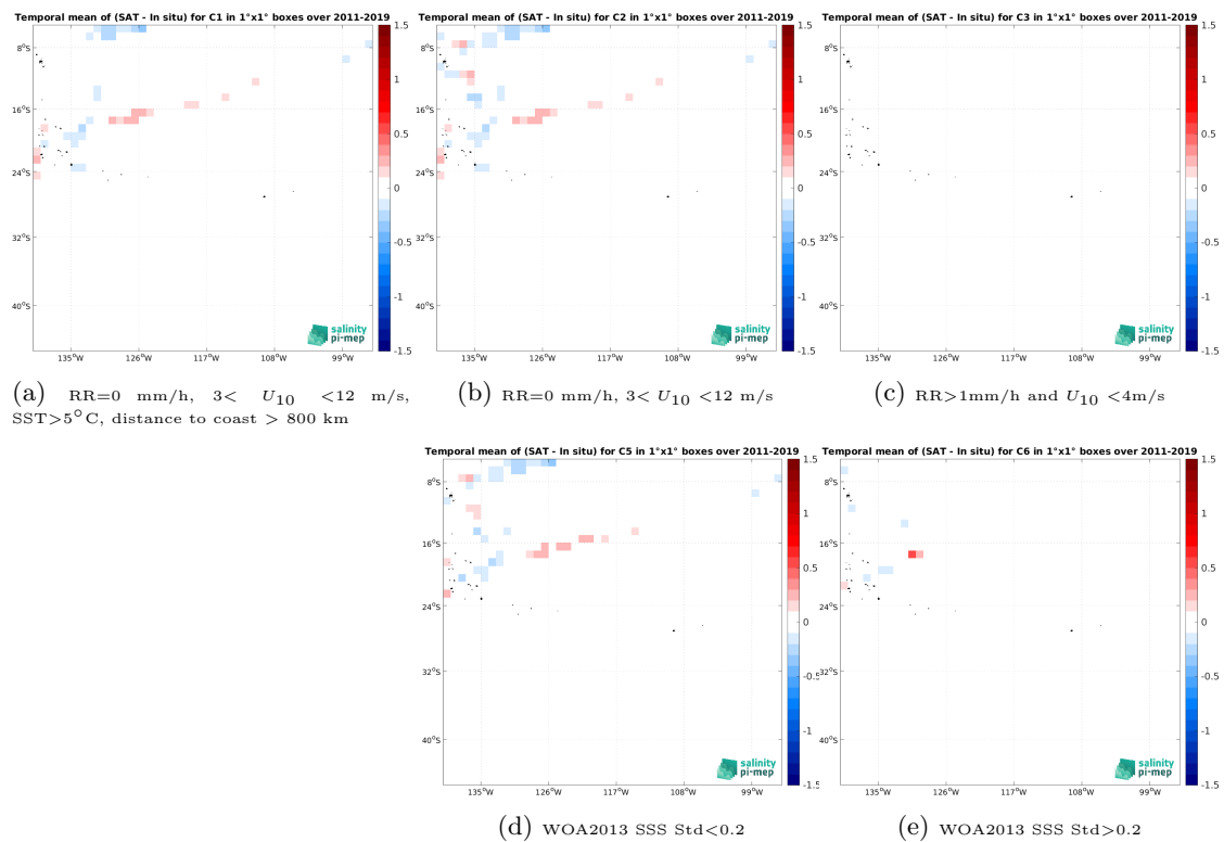
Figure 14: Temporal mean gridded over spatial boxes of size 1^\circ \times 1^\circ of \Delta SSS (SMAP SSS L4 OI v3 - Monthly (ESR) - TSG (GOSUD-Research-vessel)) for 5 different subdatasets corresponding to:RR=0 mm/h, 3 < U_{10} < 12 m/s, SST >5^\circ\text{C} , distance to coast > 800 km (a), RR=0 mm/h, 3 < U_{10} < 12 m/s (b), RR >1 mm/h and U_{10} < 4 m/s (c), WOA2013 SSS Std <0.2 (d), WOA2013 SSS Std >0.2 (e).
