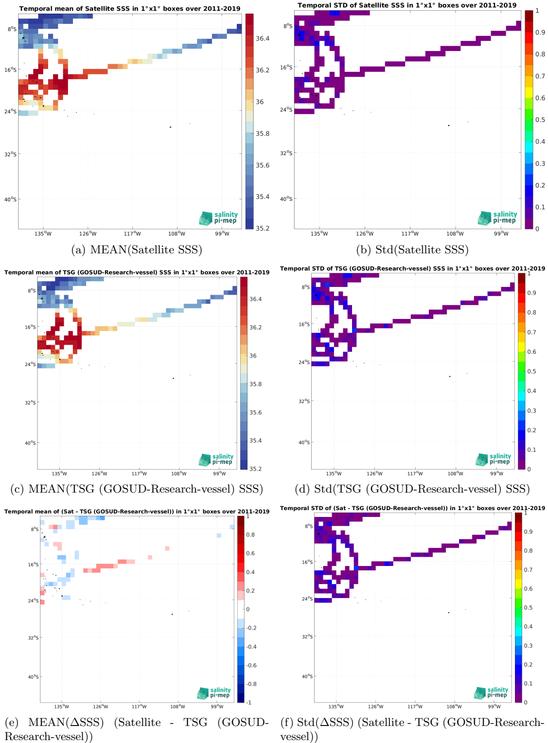
Figure 7: Temporal mean (left) and Std (right) of SSS from SMAP SSS L4 OI v3 - Monthly (ESR) (top), TSG (GOSUD-Research-vessel) (middle), and of \Delta SSS (Satellite - TSG (GOSUD-Research-vessel)). Only match-up pairs are used to generate these maps.
