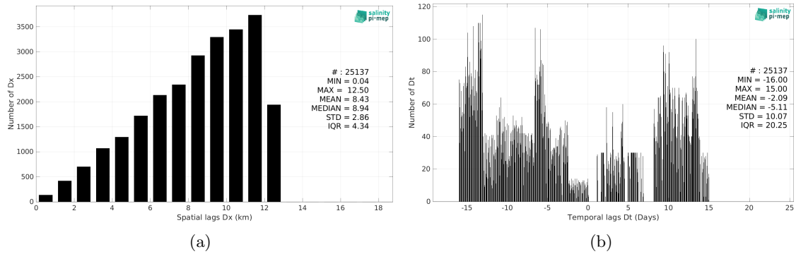
Figure 6: Histograms of the spatial (a) and temporal (b) lags between the location/time of the TSG (GOSUD-Research-vessel) measurement and the date of the corresponding SMAP SSS L4 OI v3 - Monthly (ESR) SSS pixel.
