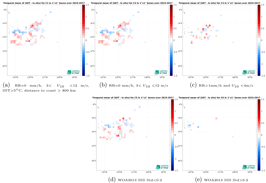
Figure 13: Temporal mean gridded over spatial boxes of size 1^\circ \times 1^\circ of \Delta SSS (SMAP SSS L4 OI v3 - Monthly (ESR) - Surface drifters) for 5 different subdatasets corresponding to:RR=0 mm/h, 3 < U_{10} < 12 m/s, SST >5^\circ C, distance to coast > 800 km (a), RR=0 mm/h, 3 < U_{10} < 12 m/s (b), RR >1 mm/h and U_{10} < 4 m/s (c), WOA2013 SSS Std <0.2 (d), WOA2013 SSS Std >0.2 (e).
