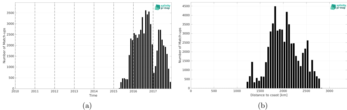
Figure 2: Number of match-ups between Surface drifters and SMAP SSS L4 OI v3 - Monthly (ESR) SSS as a function of time (a) and as function of the distance to coast (b) over the OTT zone Pi-MEP region and for the full satellite product period.
