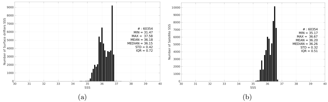
Figure 3: Histograms of SSS from Surface drifters (a) and SMAP SSS L4 OI v3 - Monthly (ESR) (b) considering all match-up pairs per bins of 0.1 over the OTT zone Pi-MEP region and for the full satellite product period.
