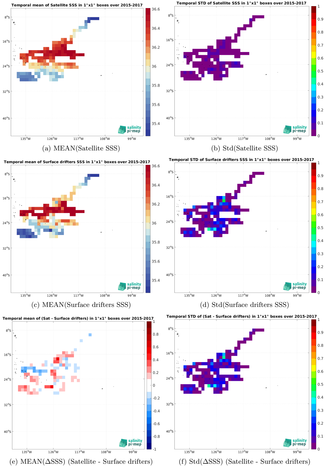
Figure 6: Temporal mean (left) and Std (right) of SSS from SMAP SSS L4 OI v3 - Monthly (ESR) (top), Surface drifters (middle), and of \Delta SSS (Satellite - Surface drifters). Only match-up pairs are used to generate these maps.
