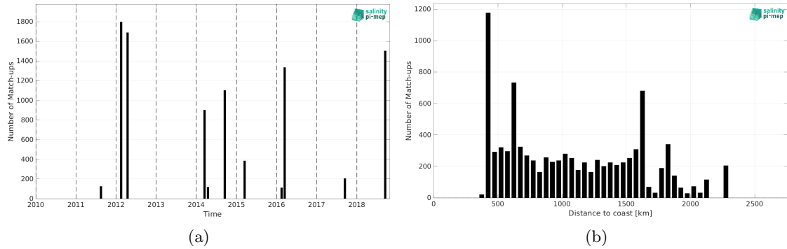
Figure 2: Number of match-ups between TSG (SAMOS) and SMAP SSS L4 OI v3 - Daily (ESR) SSS as a function of time (a) and as function of the distance to coast (b) over the OTT zone Pi-MEP region and for the full satellite product period.
