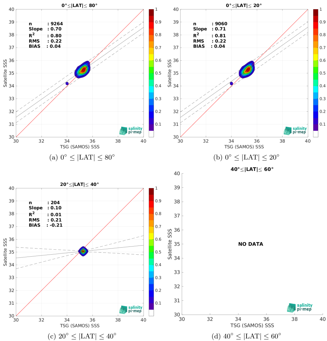
Figure 10: Contour maps of the concentration of SMAP SSS L4 OI v3 - Daily (ESR) SSS (y-axis) versus TSG (SAMOS) SSS (x-axis) at match-up pairs for different latitude bands. For each plot, the red line shows x=y . The black thin and dashed lines indicate a linear fit through the data cloud and the \pm 95\% confidence levels, respectively. The number match-up pairs n , the slope and R^2 coefficient of the linear fit, the root mean square (RMS) and the mean bias between satellite and in situ data are indicated for each latitude band in each plots.
