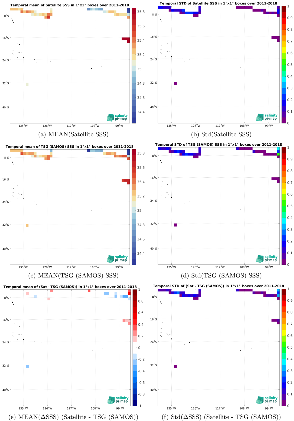
Figure 7: Temporal mean (left) and Std (right) of SSS from SMAP SSS L4 OI v3 - Daily (ESR) (top), TSG (SAMOS) (middle), and of \Delta SSS (Satellite - TSG (SAMOS)). Only match-up pairs are used to generate these maps.
