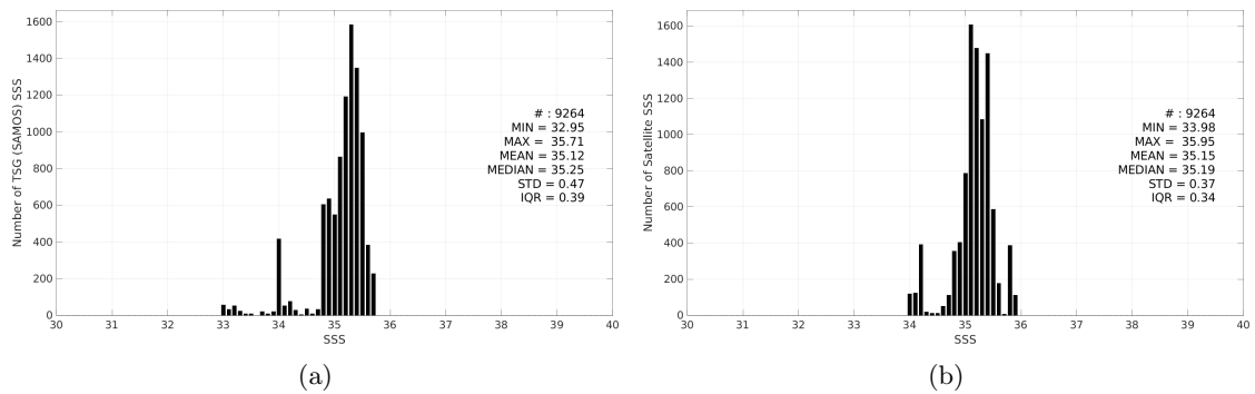
Figure 3: Histograms of SSS from TSG (SAMOS) (a) and SMAP SSS L4 OI v3 - Daily (ESR) (b) considering all match-up pairs per bins of 0.1 over the OTT zone Pi-MEP region and for the full satellite product period.
