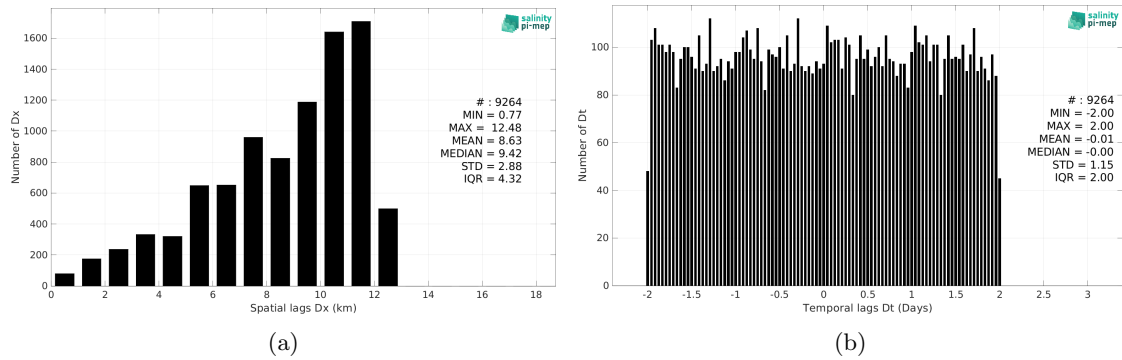
Figure 6: Histograms of the spatial (a) and temporal (b) lags between the location/time of the TSG (SAMOS) measurement and the date of the corresponding SMAP SSS L4 OI v3 - Daily (ESR) SSS pixel.
