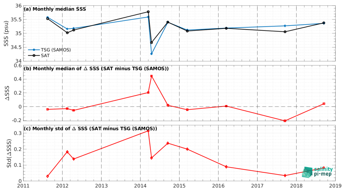
Figure 8: Time series of the monthly median SSS (top), median of \Delta SSS (Satellite - TSG (SAMOS)) and Std of \Delta SSS (Satellite - TSG (SAMOS)) over the OTT zone Pi-MEP region considering all match-ups collected by the Pi-MEP.
