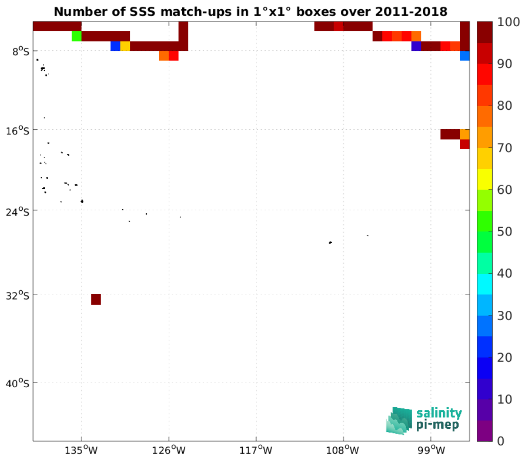
Figure 5: Number of SSS match-ups between TSG (SAMOS) SSS and the SMAP SSS L4 OI v3 - Daily (ESR) SSS product for the OTT zone Pi-MEP region over 1^\circ \times 1^\circ boxes and for the full satellite product period.
