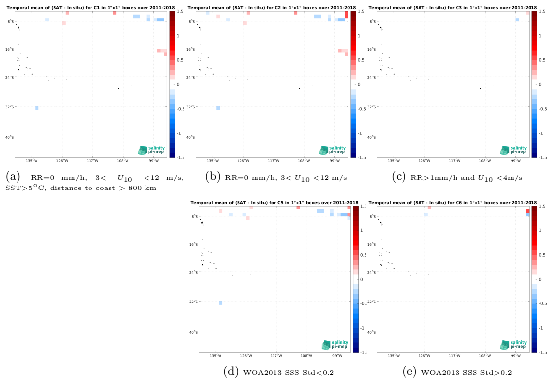
Figure 14: Temporal mean gridded over spatial boxes of size 1^\circ \times 1^\circ of \Delta SSS (SMAP SSS L4 OI v3 - Daily (ESR) - TSG (SAMOS)) for 5 different subdatasets corresponding to:RR=0 mm/h, 3 < U_{10} < 12 m/s, SST>5°C, distance to coast > 800 km (a), RR=0 mm/h, 3 < U_{10} < 12 m/s (b), RR>1mm/h and U_{10} < 4 m/s (c), WOA2013 SSS Std<0.2 (d), WOA2013 SSS Std>0.2 (e).
