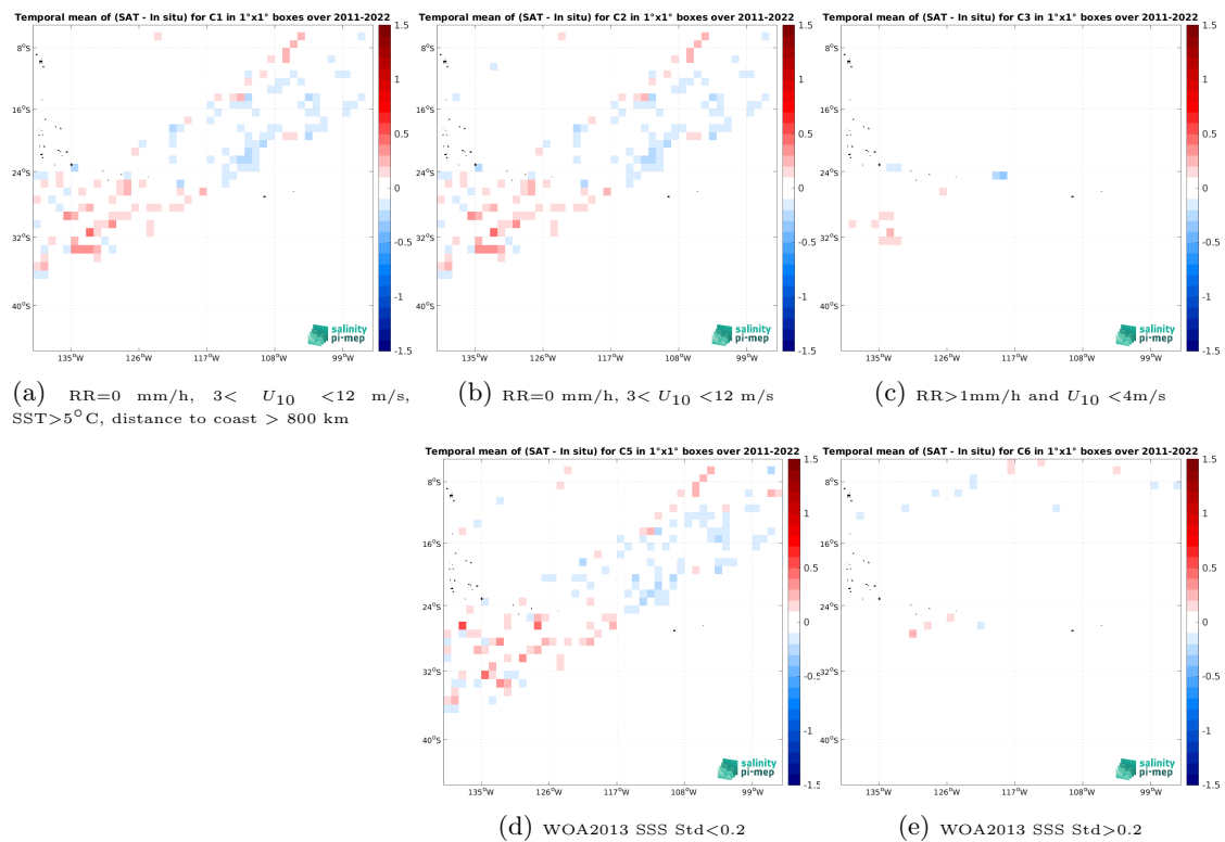
Figure 14: Temporal mean gridded over spatial boxes of size 1^\circ \times 1^\circ of \Delta SSS (SMAP SSS L4 OI v3 - Daily (ESR) - TSG (LEGOS-DM)) for 5 different subdatasets corresponding to:RR=0 mm/h, 3 < U_{10} < 12 m/s, SST >5^\circ\text{C} , distance to coast > 800 km (a), RR=0 mm/h, 3 < U_{10} < 12 m/s (b), RR >1 mm/h and U_{10} < 4 m/s (c), WOA2013 SSS Std <0.2 (d), WOA2013 SSS Std >0.2 (e).
