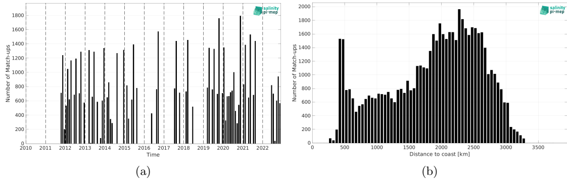
Figure 2: Number of match-ups between TSG (LEGOS-DM) and SMAP SSS L4 OI v3 - Daily (ESR) SSS as a function of time (a) and as function of the distance to coast (b) over the OTT zone Pi-MEP region and for the full satellite product period.
