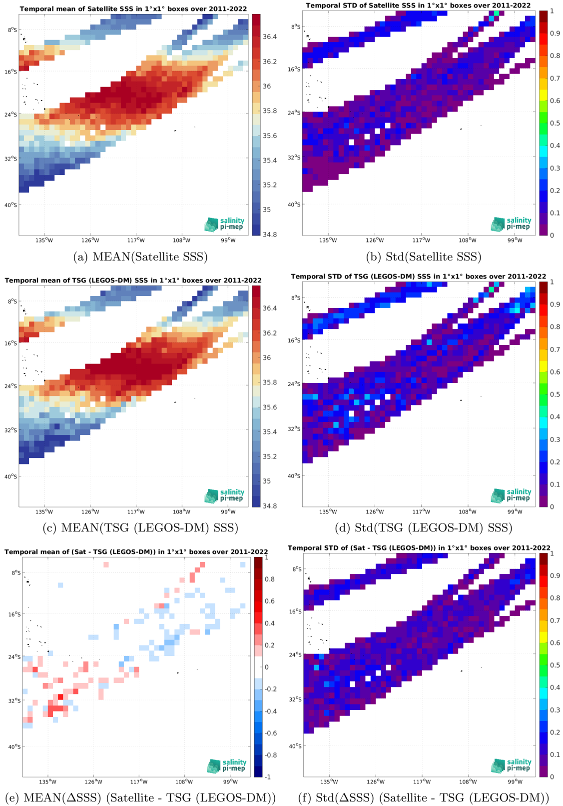
Figure 7: Temporal mean (left) and Std (right) of SSS from SMAP SSS L4 OI v3 - Daily (ESR) (top), TSG (LEGOS-DM) (middle), and of \Delta SSS (Satellite - TSG (LEGOS-DM)). Only match-up pairs are used to generate these maps.
