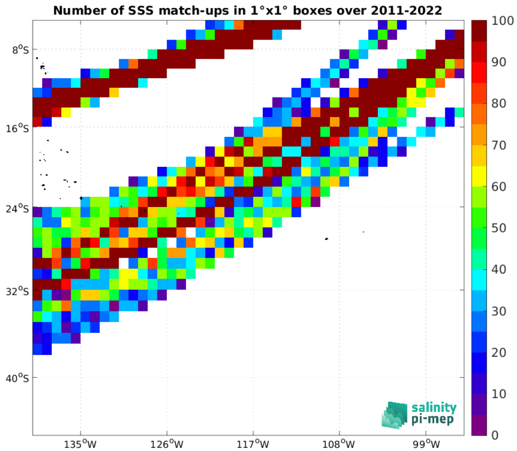
Figure 5: Number of SSS match-ups between TSG (LEGOS-DM) SSS and the SMAP SSS L4 OI v3 - Daily (ESR) SSS product for the OTT zone Pi-MEP region over 1°x1° boxes and for the full satellite product period.
