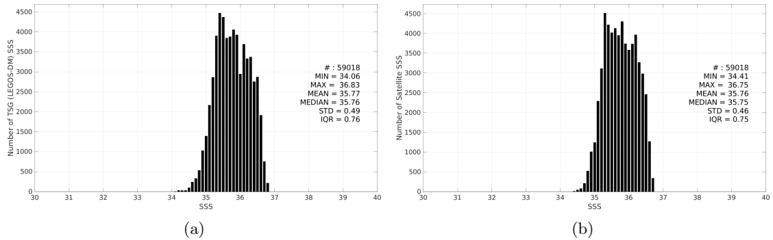
Figure 3: Histograms of SSS from TSG (LEGOS-DM) (a) and SMAP SSS L4 OI v3 - Daily (ESR) (b) considering all match-up pairs per bins of 0.1 over the OTT zone Pi-MEP region and for the full satellite product period.
