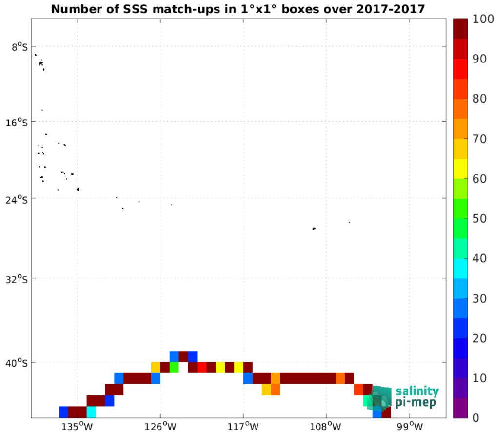
Figure 5: Number of SSS match-ups between TSG (GOSUD-Sailing-ship) SSS and the SMAP SSS L4 OI v3 - Daily (ESR) SSS product for the OTT zone Pi-MEP region over 1^\circ \times 1^\circ boxes and for the full satellite product period.
