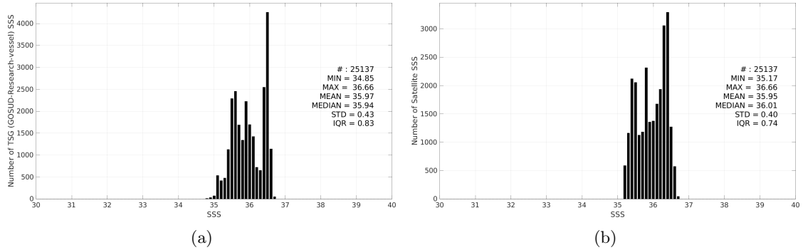
Figure 3: Histograms of SSS from TSG (GOSUD-Research-vessel) (a) and SMAP SSS L4 OI v3 - Daily (ESR) (b) considering all match-up pairs per bins of 0.1 over the OTT zone Pi-MEP region and for the full satellite product period.
