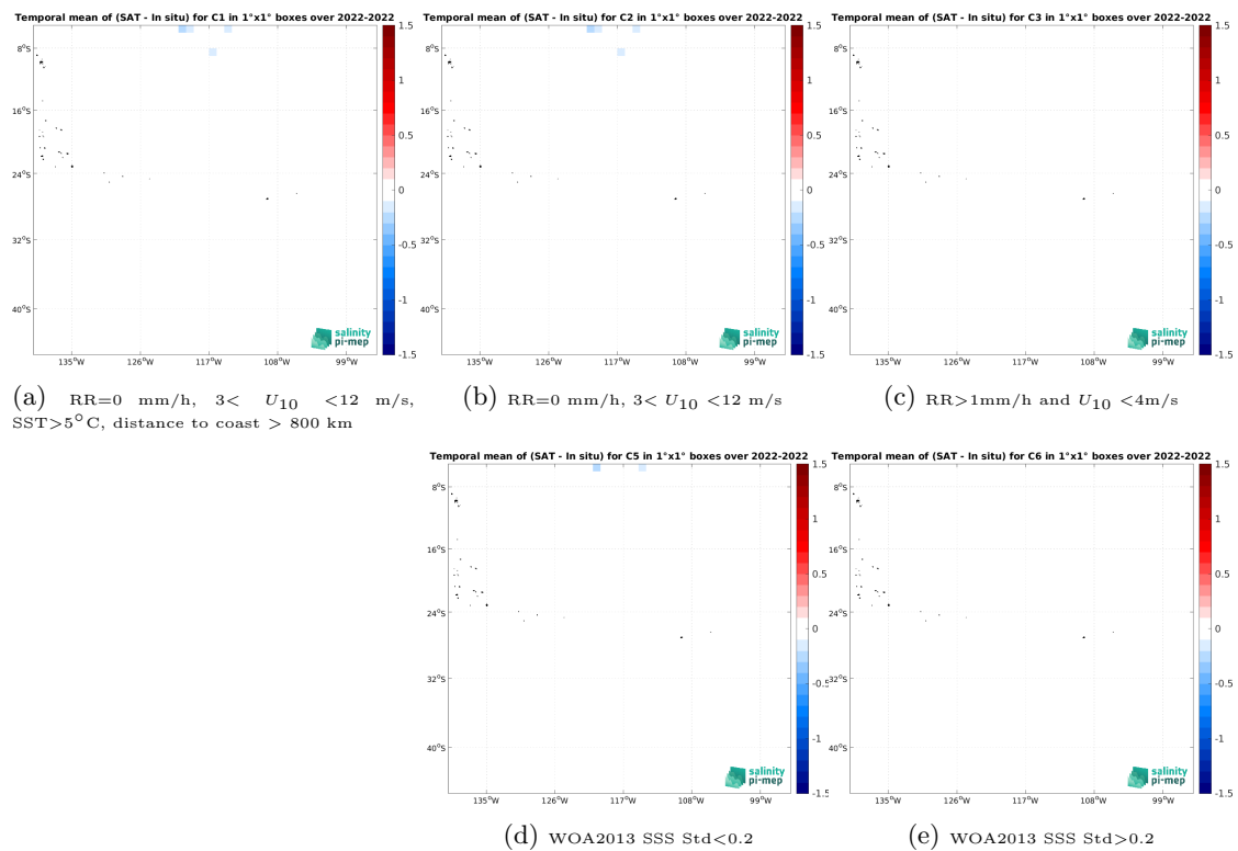
Figure 14: Temporal mean gridded over spatial boxes of size 1^\circ \times 1^\circ of \Delta SSS (SMAP SSS L4 OI v3 - Daily (ESR) - Saildrone) for 5 different subdatasets corresponding to: RR=0 mm/h, 3 < U_{10} < 12 m/s, SST > 5^\circ C , distance to coast > 800 km (a), RR=0 mm/h, 3 < U_{10} < 12 m/s (b), RR > 1 mm/h and U_{10} < 4 m/s (c), WOA2013 SSS Std < 0.2 (d), WOA2013 SSS Std > 0.2 (e).
