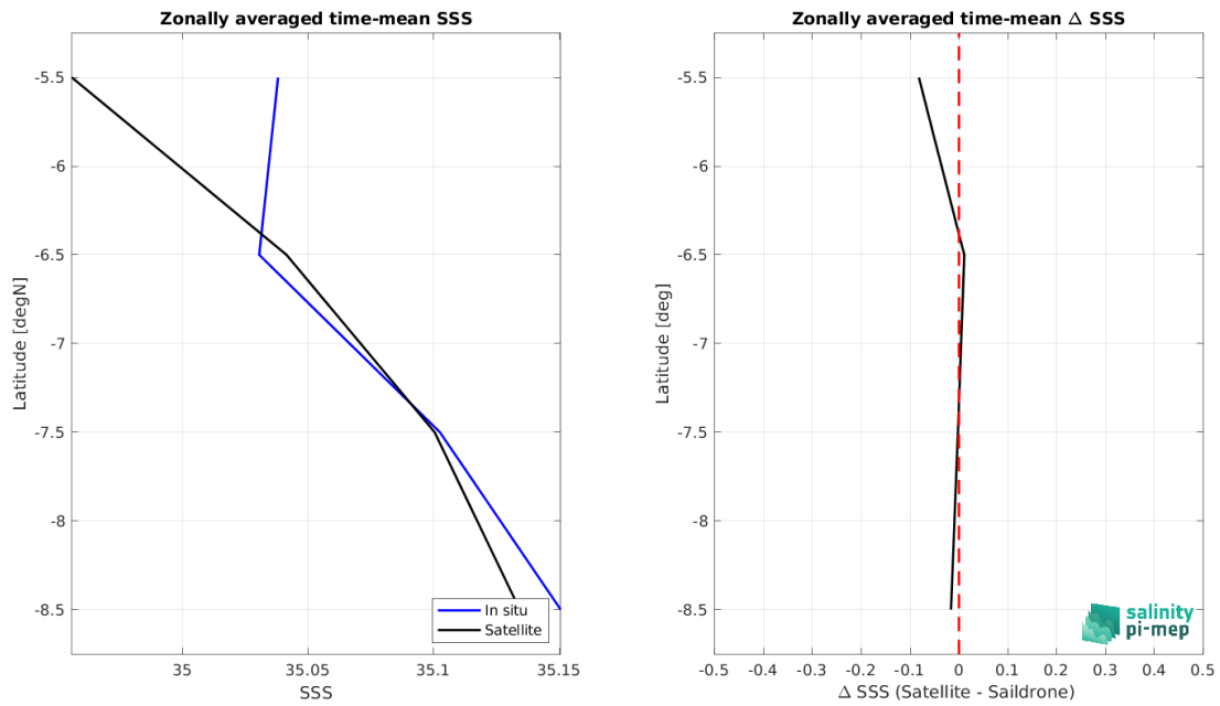
Figure 9: Left panel: Zonal mean SSS from SMAP SSS L4 OI v3 - Daily (ESR) satellite product (black) and from Sairdrone (blue). Right panel: Zonal mean of \Delta SSS (Satellite - Sairdrone) for all the collected Pi-MEP match-up pairs estimated over the full satellite product period.
