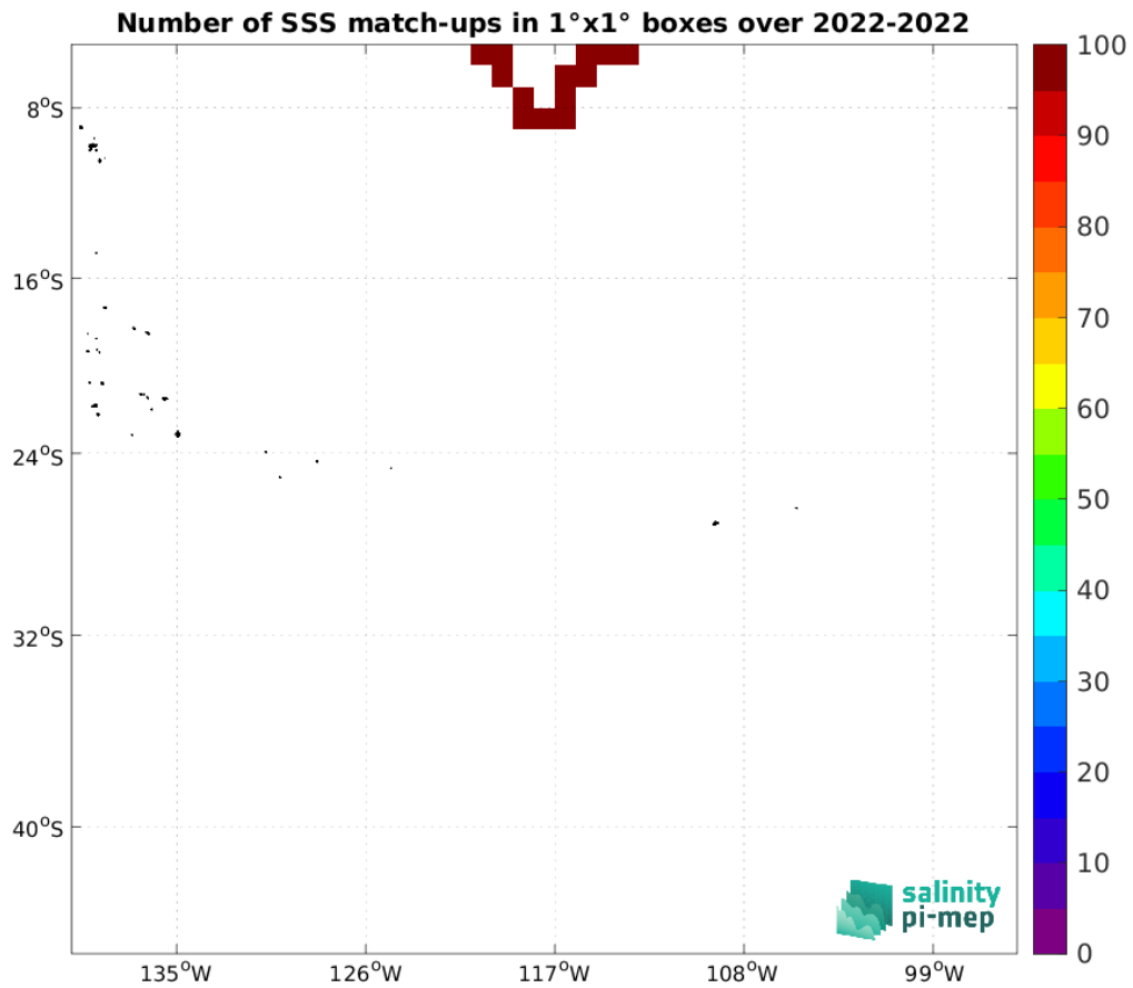
Figure 5: Number of SSS match-ups between Saildrone SSS and the SMAP SSS L4 OI v3 - Daily (ESR) SSS product for the OTT zone Pi-MEP region over 1^\circ \times 1^\circ boxes and for the full satellite product period.
