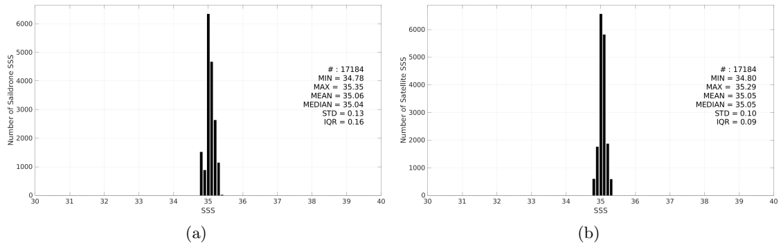
Figure 3: Histograms of SSS from Saildrone (a) and SMAP SSS L4 OI v3 - Daily (ESR) (b) considering all match-up pairs per bins of 0.1 over the OTT zone Pi-MEP region and for the full satellite product period.
