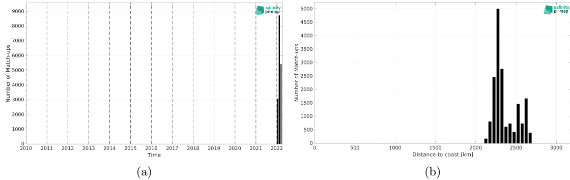
Figure 2: Number of match-ups between Saildrone and SMAP SSS L4 OI v3 - Daily (ESR) SSS as a function of time (a) and as function of the distance to coast (b) over the OTT zone Pi-MEP region and for the full satellite product period.
