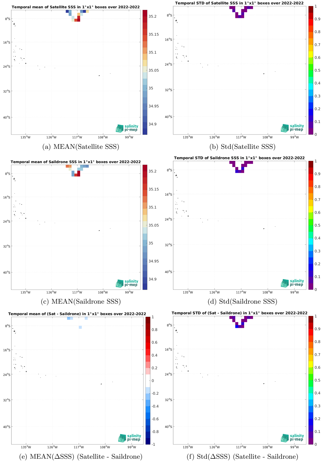
Figure 7: Temporal mean (left) and Std (right) of SSS from SMAP SSS L4 OI v3 - Daily (ESR) (top), Saildrone (middle), and of \Delta SSS (Satellite - Saildrone). Only match-up pairs are used to generate these maps.
