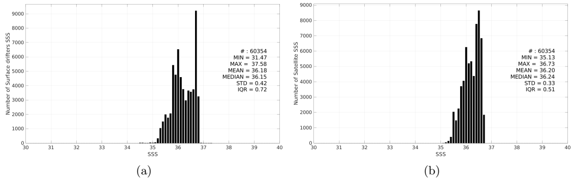
Figure 3: Histograms of SSS from Surface drifters (a) and SMAP SSS L4 OI v3 - Daily (ESR) (b) considering all match-up pairs per bins of 0.1 over the OTT zone Pi-MEP region and for the full satellite product period.
