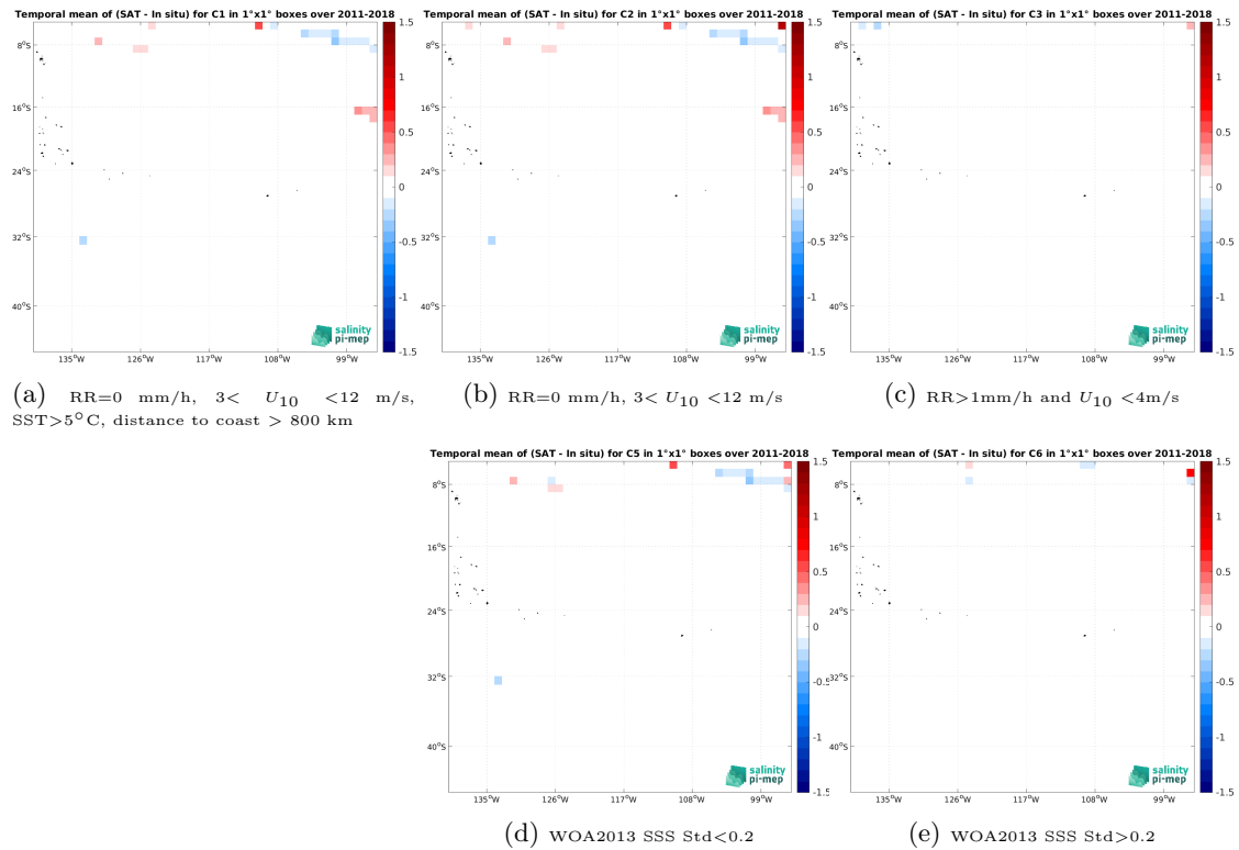
Figure 12: Temporal mean gridded over spatial boxes of size 1^\circ \times 1^\circ of \Delta SSS (SMAP SSS L4 OI v2 - 7 Days (ESR) - TSG (SAMOS)) for 5 different subdatasets corresponding to:RR=0 mm/h, 3 < U_{10} < 12 m/s, SST >5^\circ C, distance to coast > 800 km (a), RR=0 mm/h, 3 < U_{10} < 12 m/s (b), RR >1 mm/h and U_{10} < 4 m/s (c), WOA2013 SSS Std <0.2 (d), WOA2013 SSS Std >0.2 (e).
