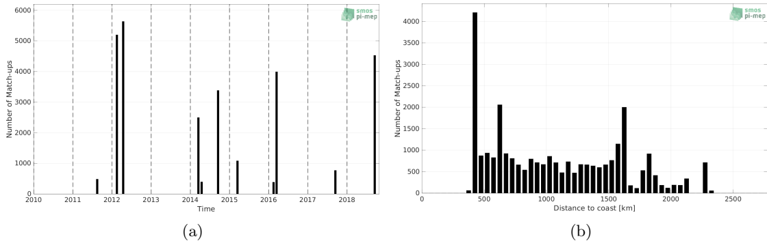
Figure 1: Number of match-ups between TSG (SAMOS) and SMAP SSS L4 OI v2 - 7 Days (ESR) SSS as a function of time (a) and as function of the distance to coast (b) over the OTT zone Pi-MEP region and for the full satellite product period.
