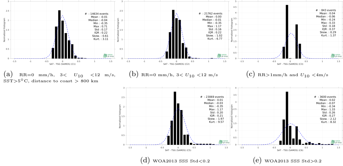
Figure 13: Normalized histogram of \Delta SSS (SMAP SSS L4 OI v2 - 7 Days (ESR) - TSG (SAMOS)) for 5 different subdatasets corresponding to: RR=0 mm/h, 3 < U_{10} < 12 m/s, SST>5°C, distance to coast > 800 km (a), RR=0 mm/h, 3 < U_{10} < 12 m/s (b), RR>1mm/h and U_{10} < 4 m/s (c), WOA2013 SSS Std<0.2 (d), WOA2013 SSS Std>0.2 (e).
