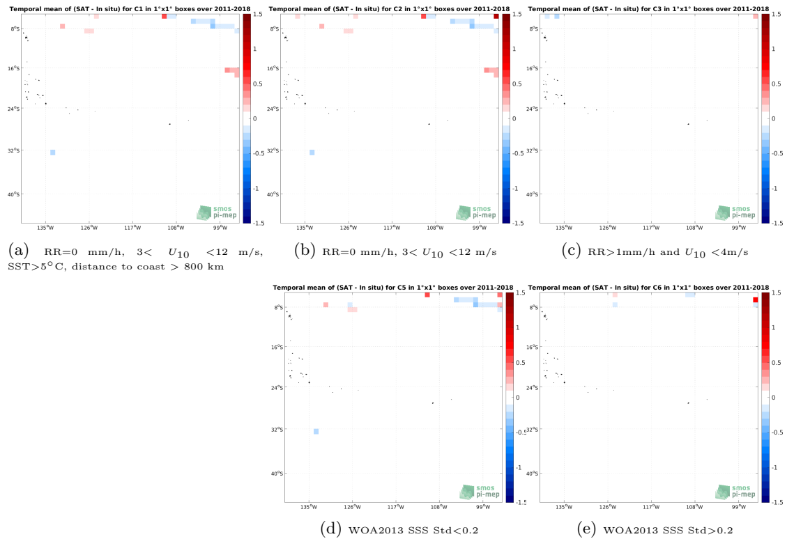
Figure 12: Temporal mean gridded over spatial boxes of size 1^\circ \times 1^\circ of \Delta SSS (SMAP SSS L4 OI v2 - 7 Days (ESR) - TSG (SAMOS)) for 5 different subdatasets corresponding to: RR=0 mm/h, 3 < U_{10} < 12 m/s, SST > 5^\circ\text{C} , distance to coast > 800 km (a), RR=0 mm/h, 3 < U_{10} < 12 m/s (b), RR > 1 mm/h and U_{10} < 4 m/s (c), WOA2013 SSS Std < 0.2 (d), WOA2013 SSS Std > 0.2 (e).
