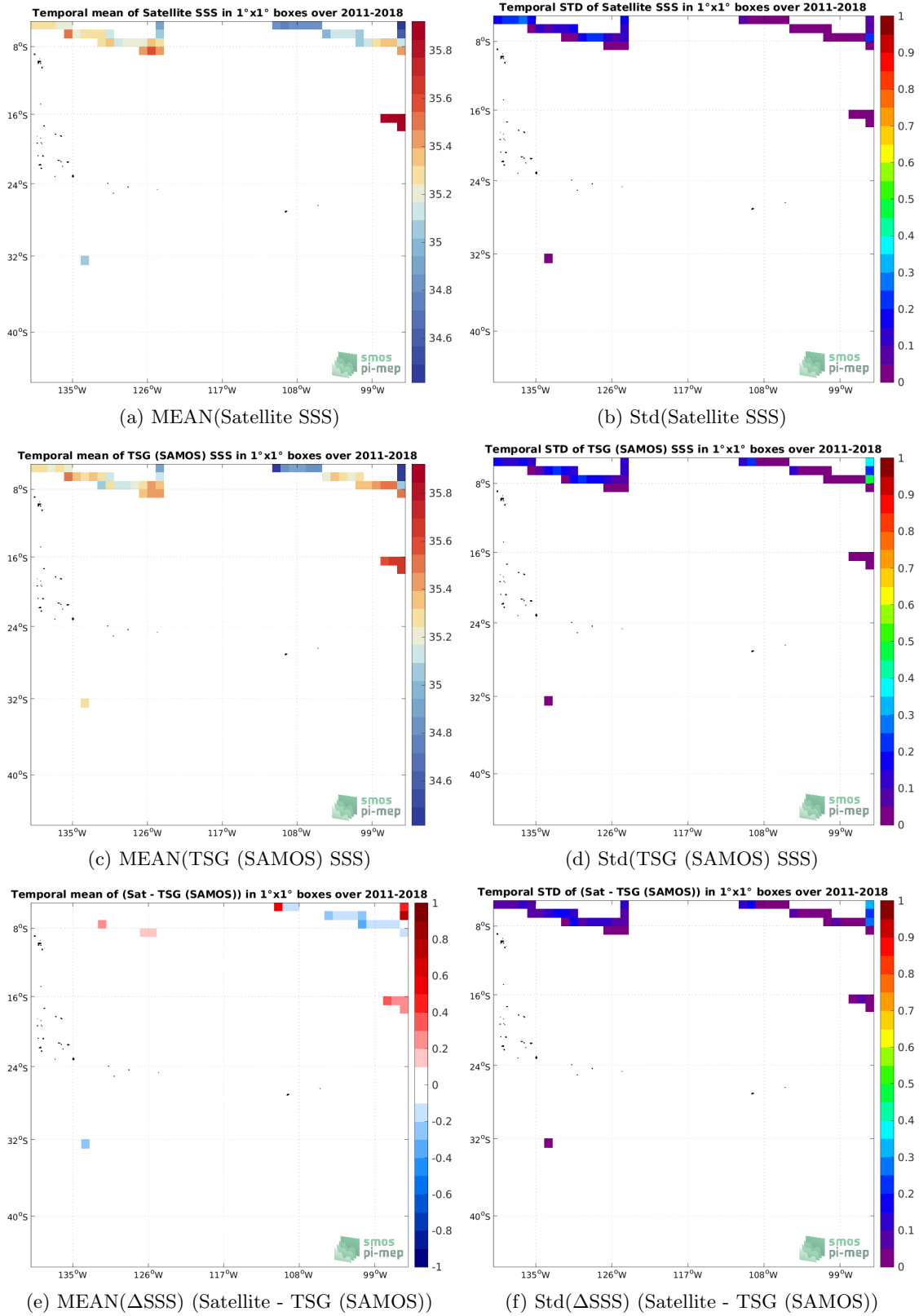
Figure 6: Temporal mean (left) and Std (right) of SSS from SMAP SSS L4 OI v2 - 7 Days (ESR) (top), TSG (SAMOS) (middle), and of \Delta SSS (Satellite - TSG (SAMOS)). Only match-up pairs are used to generate these maps.
