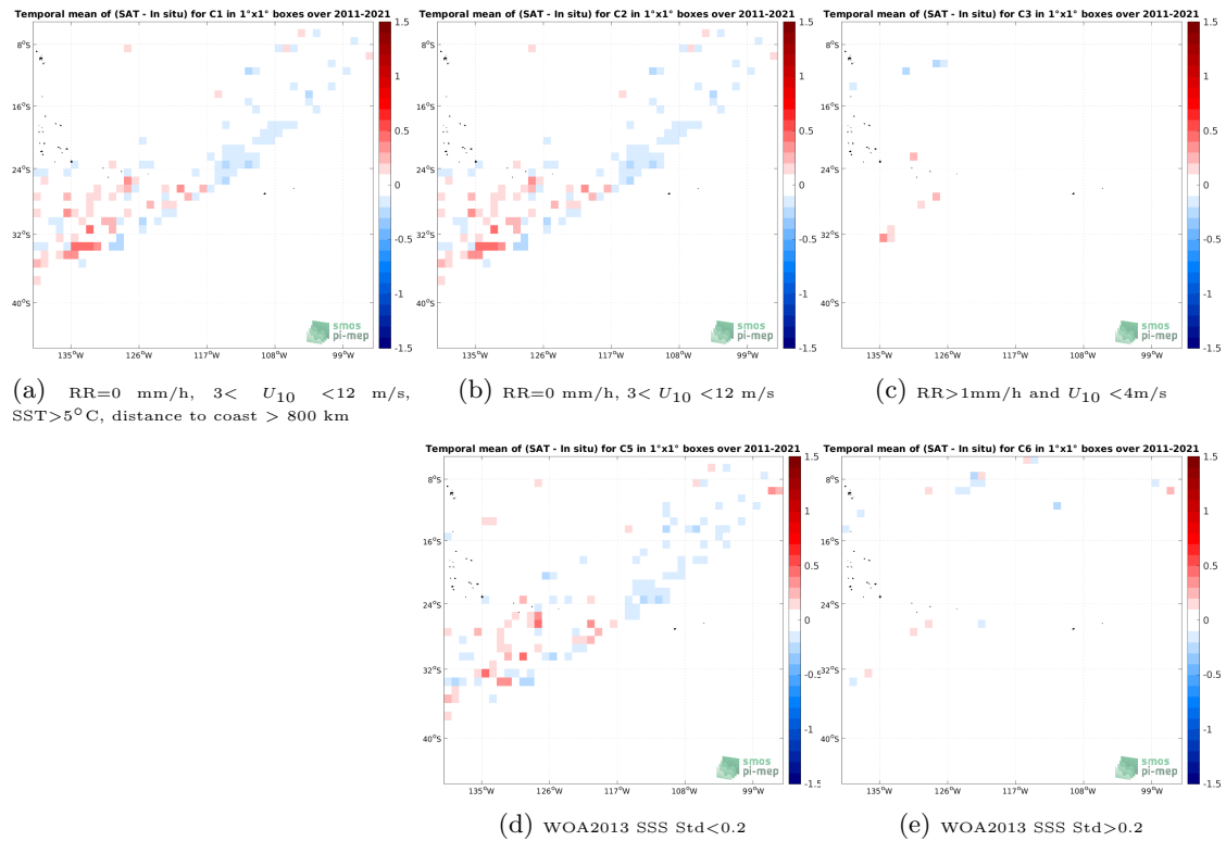
Figure 12: Temporal mean gridded over spatial boxes of size 1^\circ \times 1^\circ of \Delta SSS (SMAP SSS L4 OI v2 - 7 Days (ESR) - TSG (LEGOS-DM)) for 5 different subdatasets corresponding to:RR=0 mm/h, 3 < U_{10} < 12 m/s, SST >5^\circ C, distance to coast > 800 km (a), RR=0 mm/h, 3 < U_{10} < 12 m/s (b), RR >1 mm/h and U_{10} < 4 m/s (c), WOA2013 SSS Std <0.2 (d), WOA2013 SSS Std >0.2 (e).
