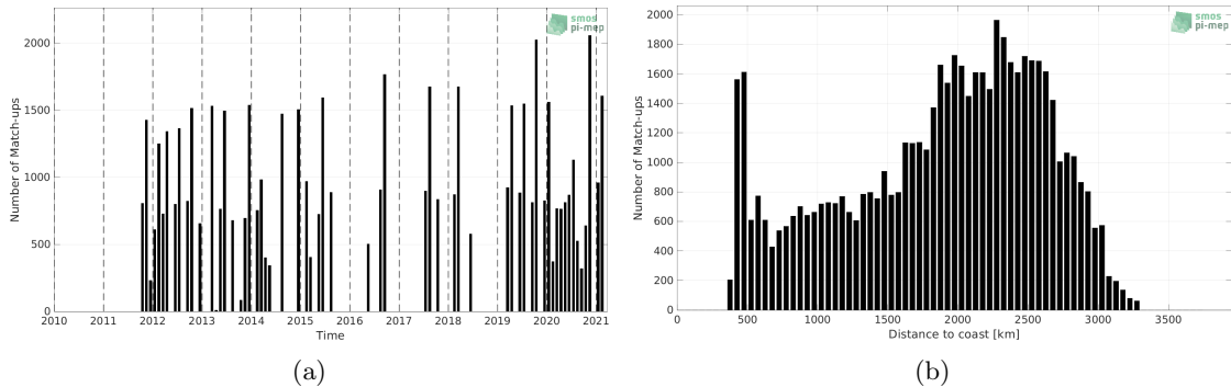
Figure 1: Number of match-ups between TSG (LEGOS-DM) and SMAP SSS L4 OI v2 - 7 Days (ESR) SSS as a function of time (a) and as function of the distance to coast (b) over the OTT zone Pi-MEP region and for the full satellite product period.
