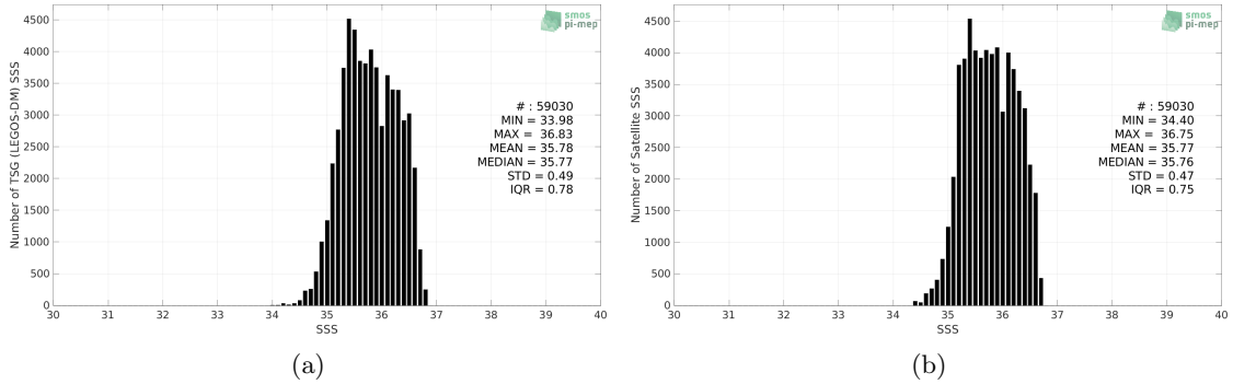
Figure 2: Histograms of SSS from TSG (LEGOS-DM) (a) and SMAP SSS L4 OI v2 - 7 Days (ESR) (b) considering all match-up pairs per bins of 0.1 over the OTT zone Pi-MEP region and for the full satellite product period.
