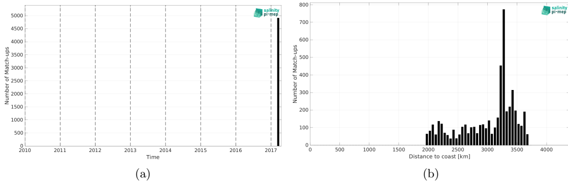
Figure 1: Number of match-ups between TSG (GOSUD-Sailing-ship) and SMAP SSS L4 OI v2 - 7 Days (ESR) SSS as a function of time (a) and as function of the distance to coast (b) over the OTT zone Pi-MEP region and for the full satellite product period.
