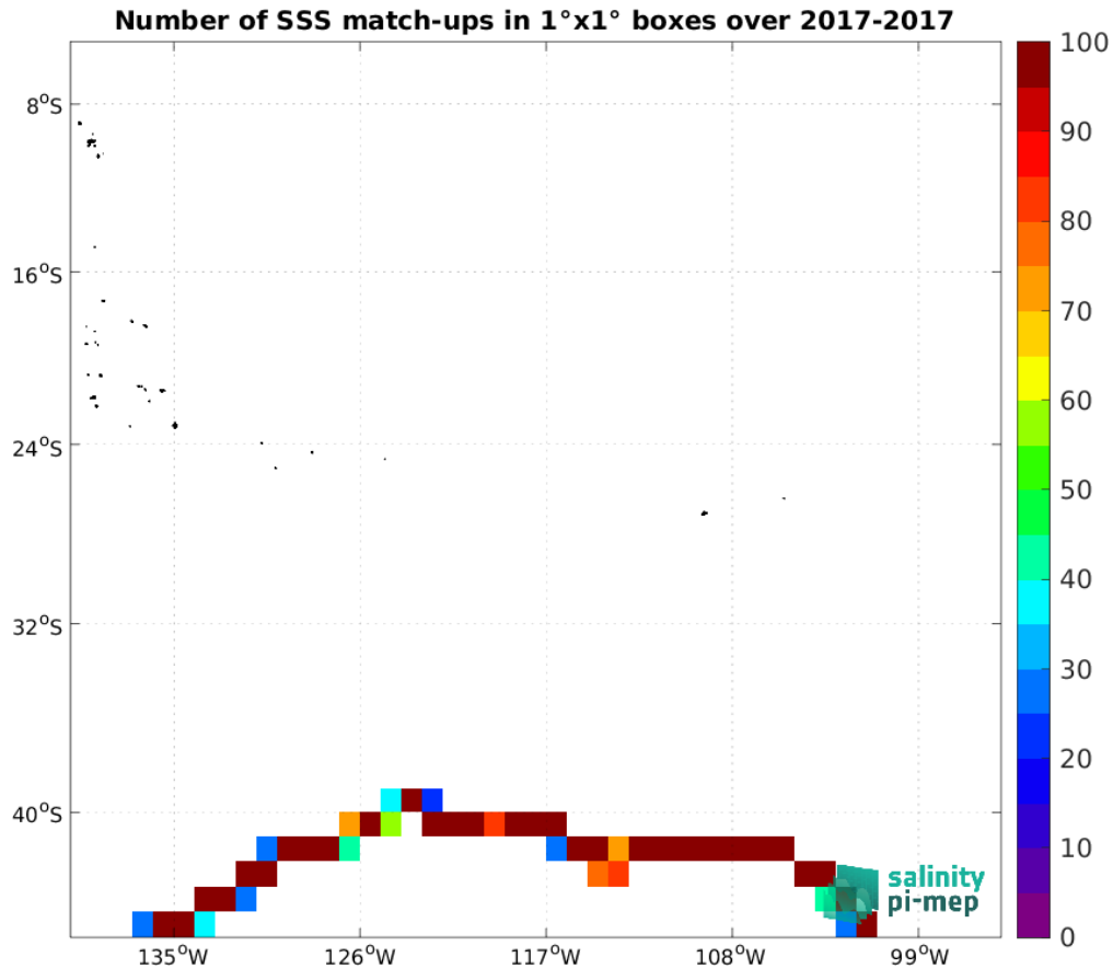
Figure 4: Number of SSS match-ups between TSG (GOSUD-Sailing-ship) SSS and the SMAP SSS L4 OI v2 - 7 Days (ESR) SSS product for the OTT zone Pi-MEP region over 1^\circ \times 1^\circ boxes and for the full satellite product period.
