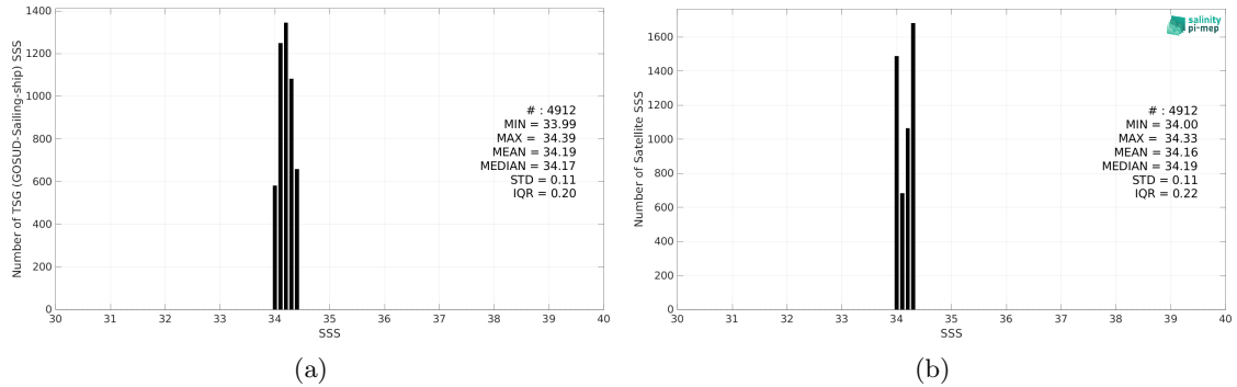
Figure 2: Histograms of SSS from TSG (GOSUD-Sailing-ship) (a) and SMAP SSS L4 OI v2 - 7 Days (ESR) (b) considering all match-up pairs per bins of 0.1 over the OTT zone Pi-MEP region and for the full satellite product period.
