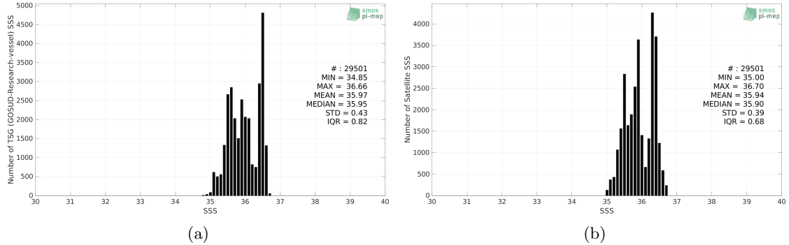
Figure 2: Histograms of SSS from TSG (GOSUD-Research-vessel) (a) and SMAP SSS L4 OI v2 - 7 Days (ESR) (b) considering all match-up pairs per bins of 0.1 over the OTT zone Pi-MEP region and for the full satellite product period.
