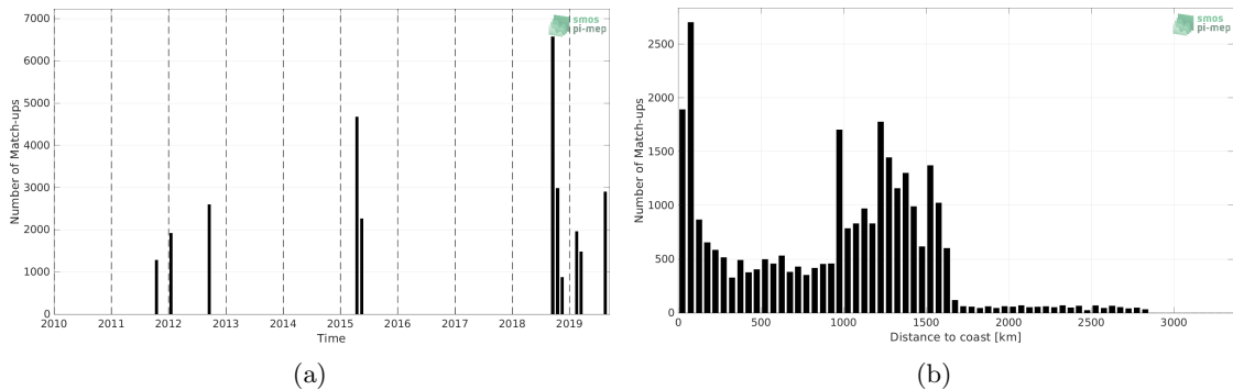
Figure 1: Number of match-ups between TSG (GOSUD-Research-vessel) and SMAP SSS L4 OI v2 - 7 Days (ESR) SSS as a function of time (a) and as function of the distance to coast (b) over the OTT zone Pi-MEP region and for the full satellite product period.
