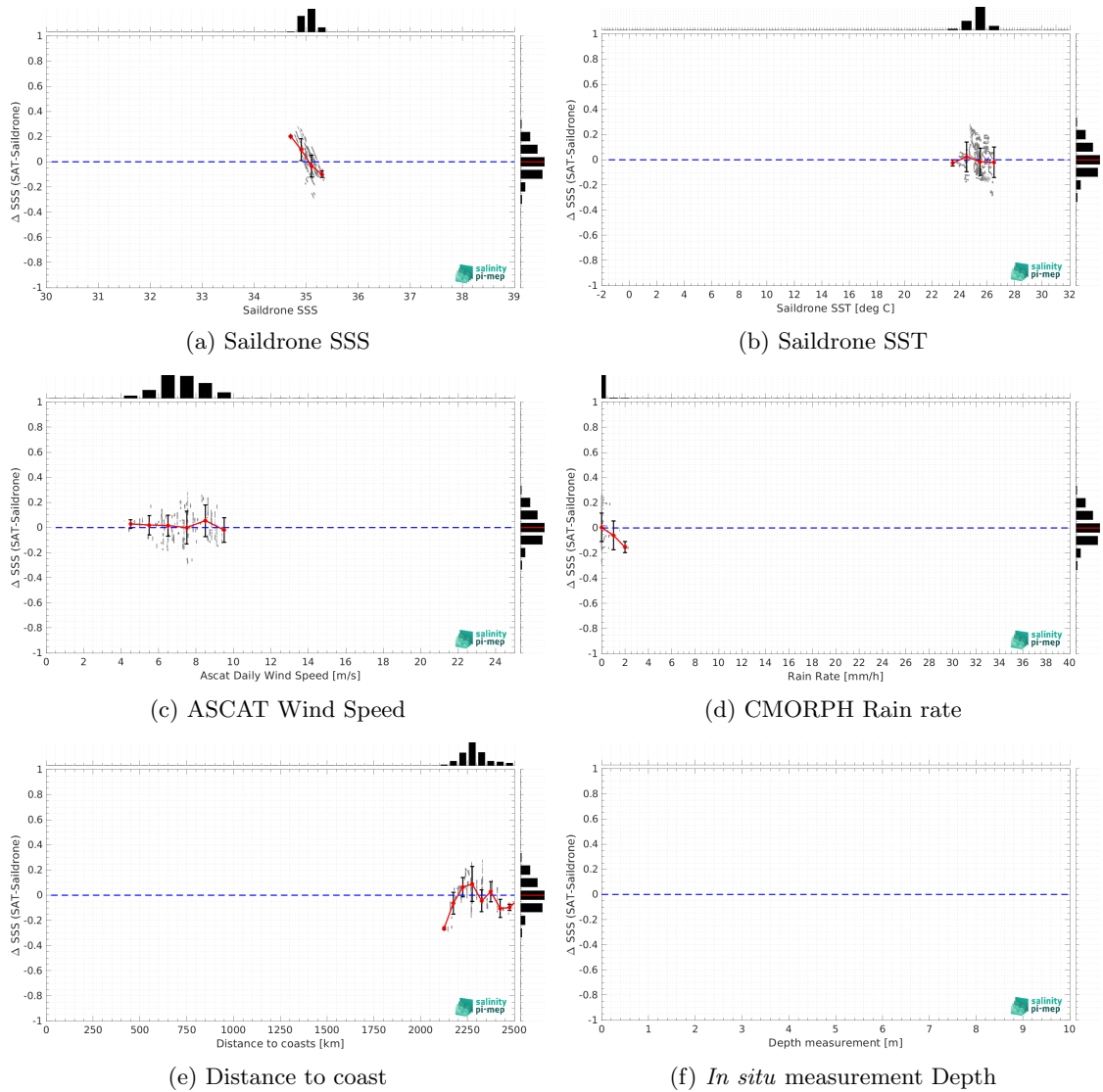
Figure 11: \Delta \text{SSS} (Satellite - Saildrone) sorted as function of Saildrone SSS values a), Saildrone SST b), ASCAT Wind speed c), CMORPH rain rate d), distance to coast (e) and in situ measurement depth (f). In all plots the median and Std of \Delta \text{SSS} for each bin is indicated by the red curves and black vertical thick bars ( \pm 1 \text{ Std} )
