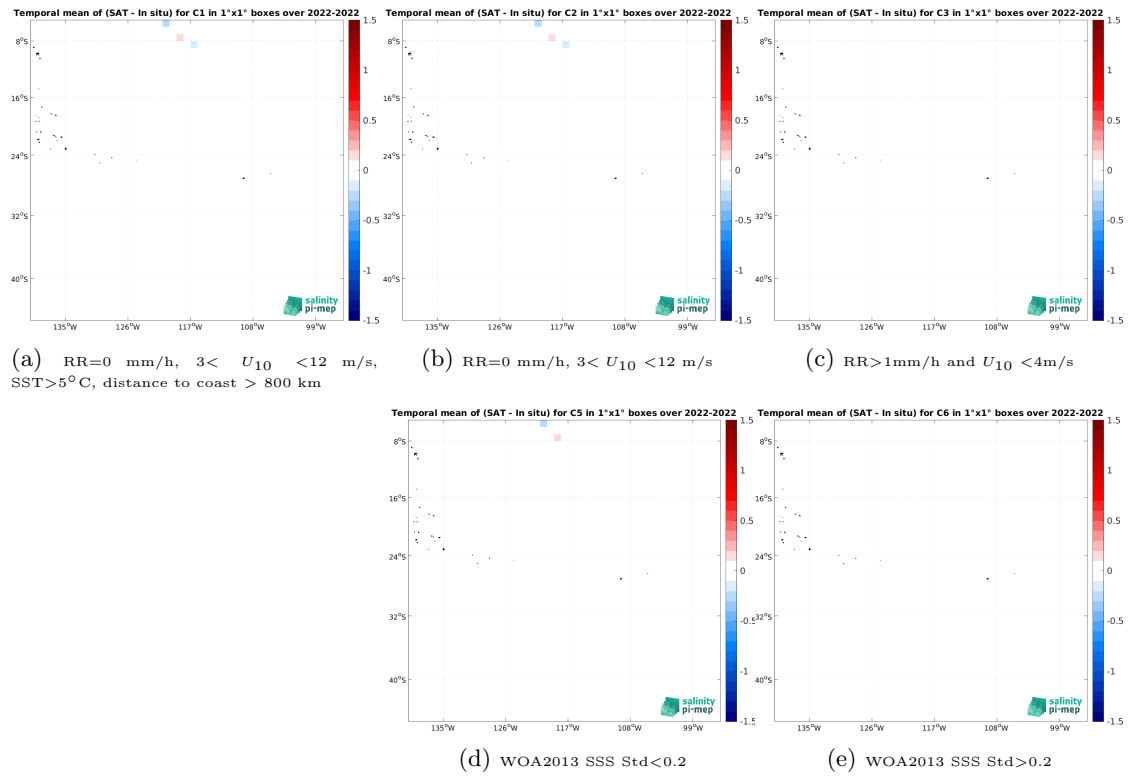
Figure 12: Temporal mean gridded over spatial boxes of size 1^\circ \times 1^\circ of \Delta SSS (SMAP SSS L4 OI v2 - 7 Days (ESR) - Saldrone) for 5 different subdatasets corresponding to:RR=0 mm/h, 3 < U_{10} < 12 m/s, SST > 5^\circ\text{C} , distance to coast > 800 km (a), RR=0 mm/h, 3 < U_{10} < 12 m/s (b), RR > 1 mm/h and U_{10} < 4 m/s (c), WOA2013 SSS Std < 0.2 (d), WOA2013 SSS Std > 0.2 (e).
