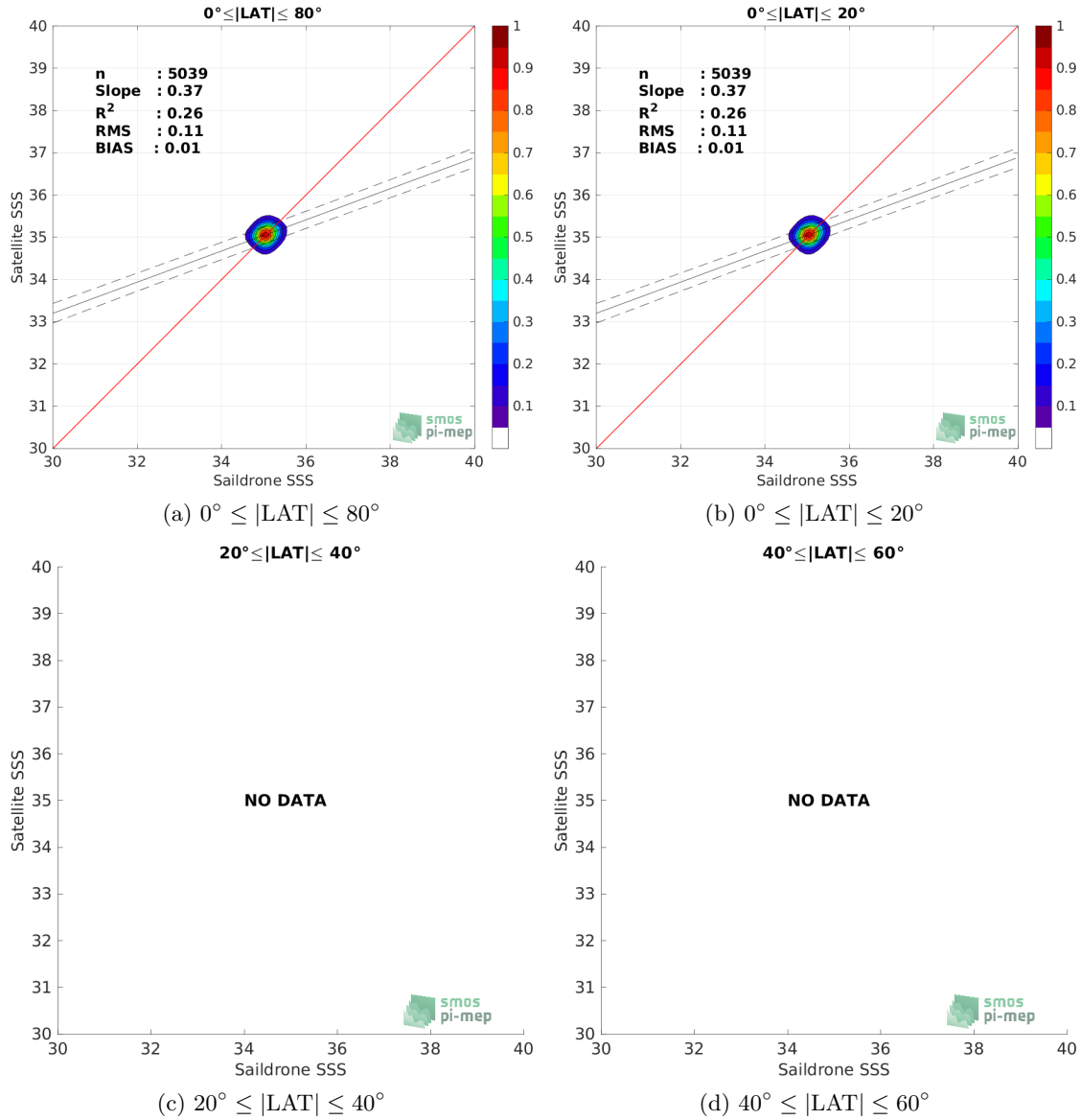
Figure 9: Contour maps of the concentration of SMAP SSS L4 OI v2 - 7 Days (ESR) SSS (y-axis) versus Sailldrone SSS (x-axis) at match-up pairs for different latitude bands. For each plot, the red line shows x=y . The black thin and dashed lines indicate a linear fit through the data cloud and the \pm 95\% confidence levels, respectively. The number match-up pairs n , the slope and R^2 coefficient of the linear fit, the root mean square (RMS) and the mean bias between satellite and in situ data are indicated for each latitude band in each plots.
