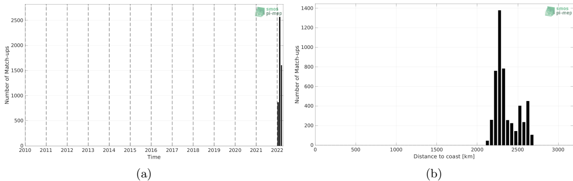
Figure 1: Number of match-ups between Saildrone and SMAP SSS L4 OI v2 - 7 Days (ESR) SSS as a function of time (a) and as function of the distance to coast (b) over the OTT zone Pi-MEP region and for the full satellite product period.
