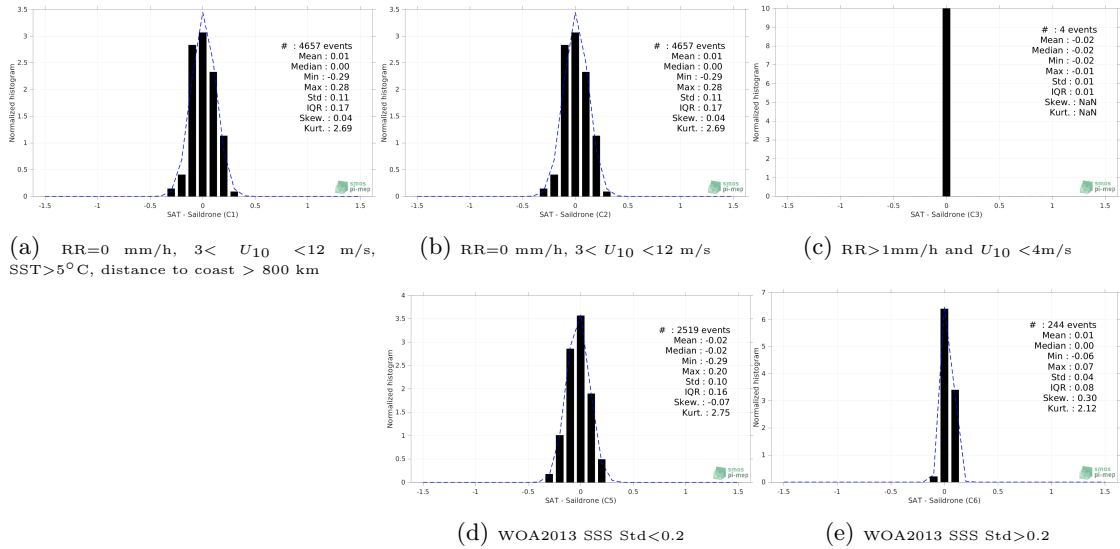
Figure 13: Normalized histogram of \Delta SSS (SMAP SSS L4 OI v2 - 7 Days (ESR) - Saildrone) for 5 different subdatasets corresponding to: RR=0 mm/h, 3 < U_{10} < 12 m/s, SST > 5°C, distance to coast > 800 km (a), RR=0 mm/h, 3 < U_{10} < 12 m/s (b), RR > 1mm/h and U_{10} < 4 m/s (c), WOA2013 SSS Std < 0.2 (d), WOA2013 SSS Std > 0.2 (e).
