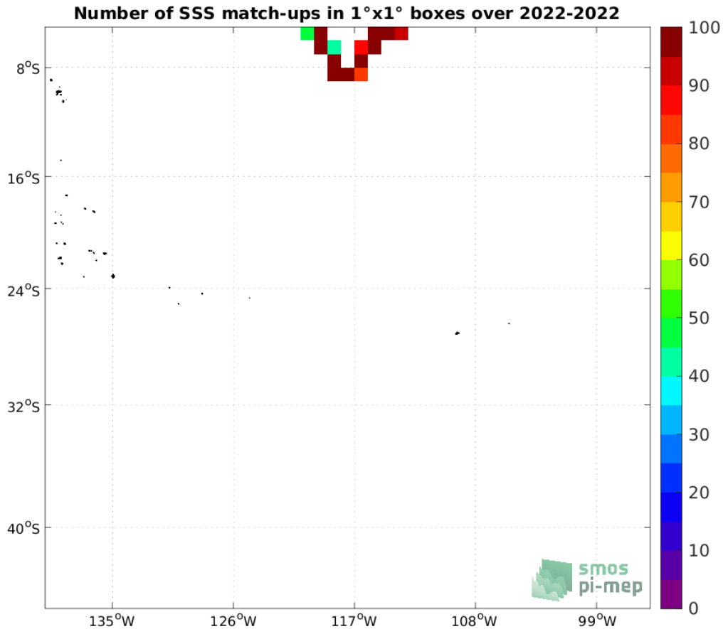
Figure 4: Number of SSS match-ups between Saildrone SSS and the SMAP SSS L4 OI v2 - 7 Days (ESR) SSS product for the OTT zone Pi-MEP region over 1^\circ \times 1^\circ boxes and for the full satellite product period.
