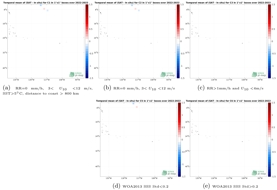
Figure 12: Temporal mean gridded over spatial boxes of size 1^\circ \times 1^\circ of \Delta SSS (SMAP SSS L4 OI v2 - 7 Days (ESR) - Sairdrone) for 5 different subdatasets corresponding to:RR=0 mm/h, 3 < U_{10} < 12 m/s, SST >5^\circ\text{C} , distance to coast > 800 km (a), RR=0 mm/h, 3 < U_{10} < 12 m/s (b), RR >1 mm/h and U_{10} < 4 m/s (c), WOA2013 SSS Std <0.2 (d), WOA2013 SSS Std >0.2 (e).
