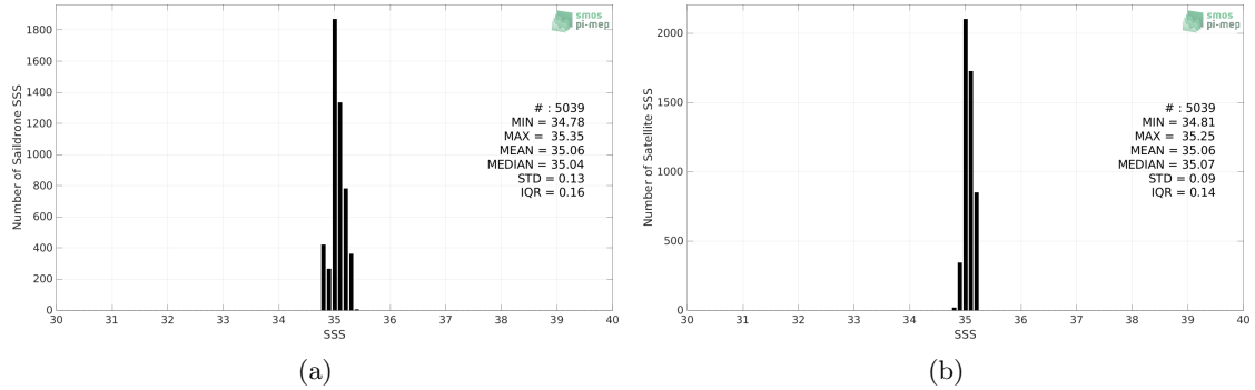
Figure 2: Histograms of SSS from Saildrone (a) and SMAP SSS L4 OI v2 - 7 Days (ESR) (b) considering all match-up pairs per bins of 0.1 over the OTT zone Pi-MEP region and for the full satellite product period.
