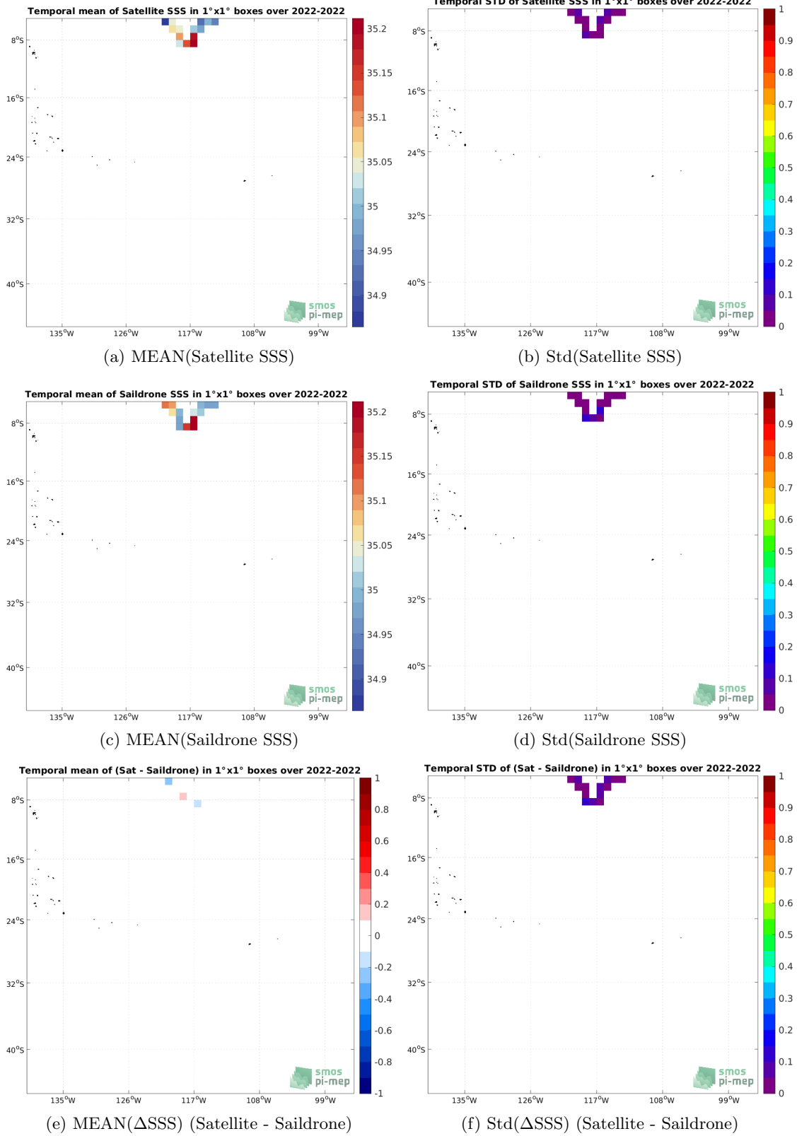
Figure 6: Temporal mean (left) and Std (right) of SSS from SMAP SSS L4 OI v2 - 7 Days (ESR) (top), Saildrone (middle), and of \Delta SSS (Satellite - Saildrone). Only match-up pairs are used to generate these maps.
